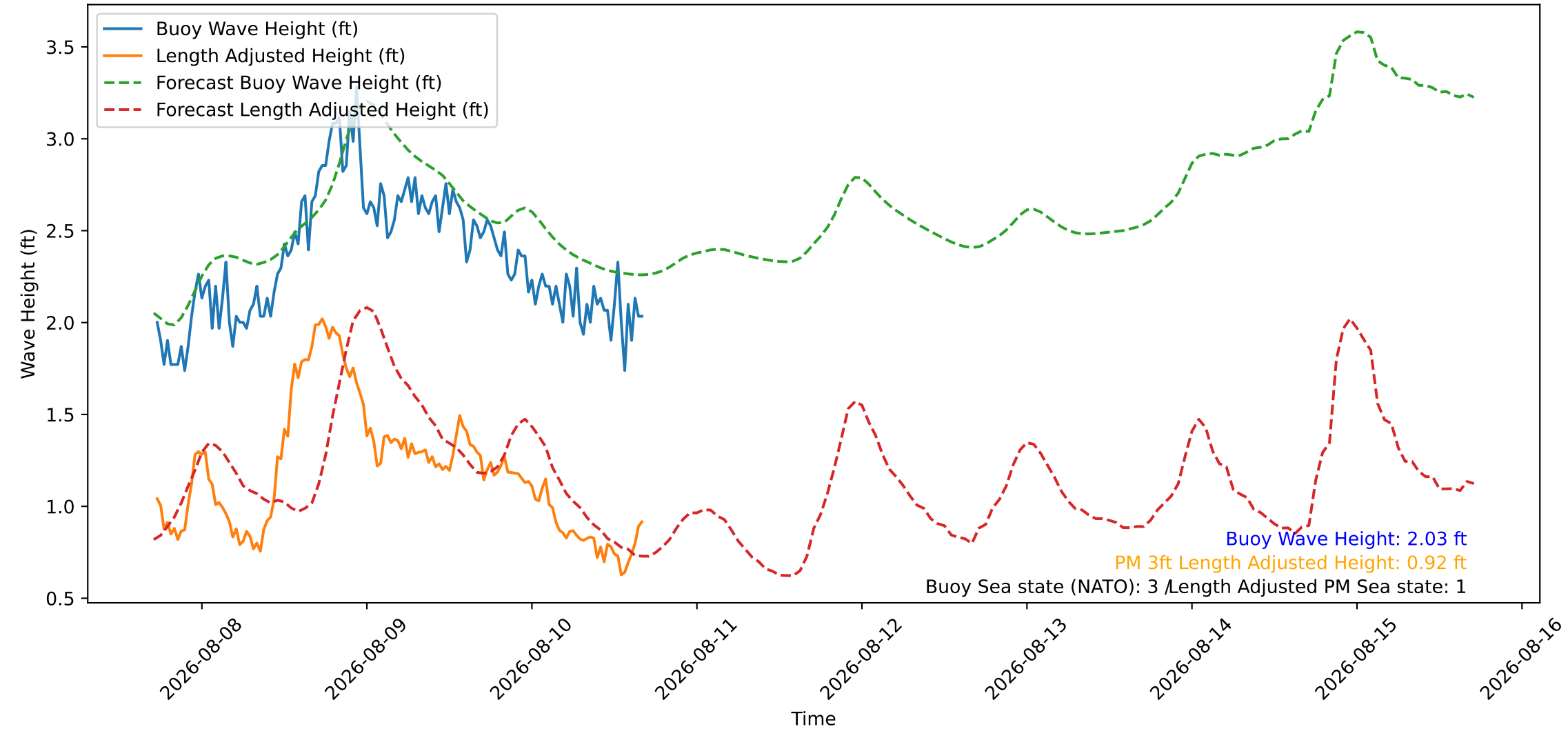
Wave Heights over Time for Red Beach at 2026-08-10 17:10:46
