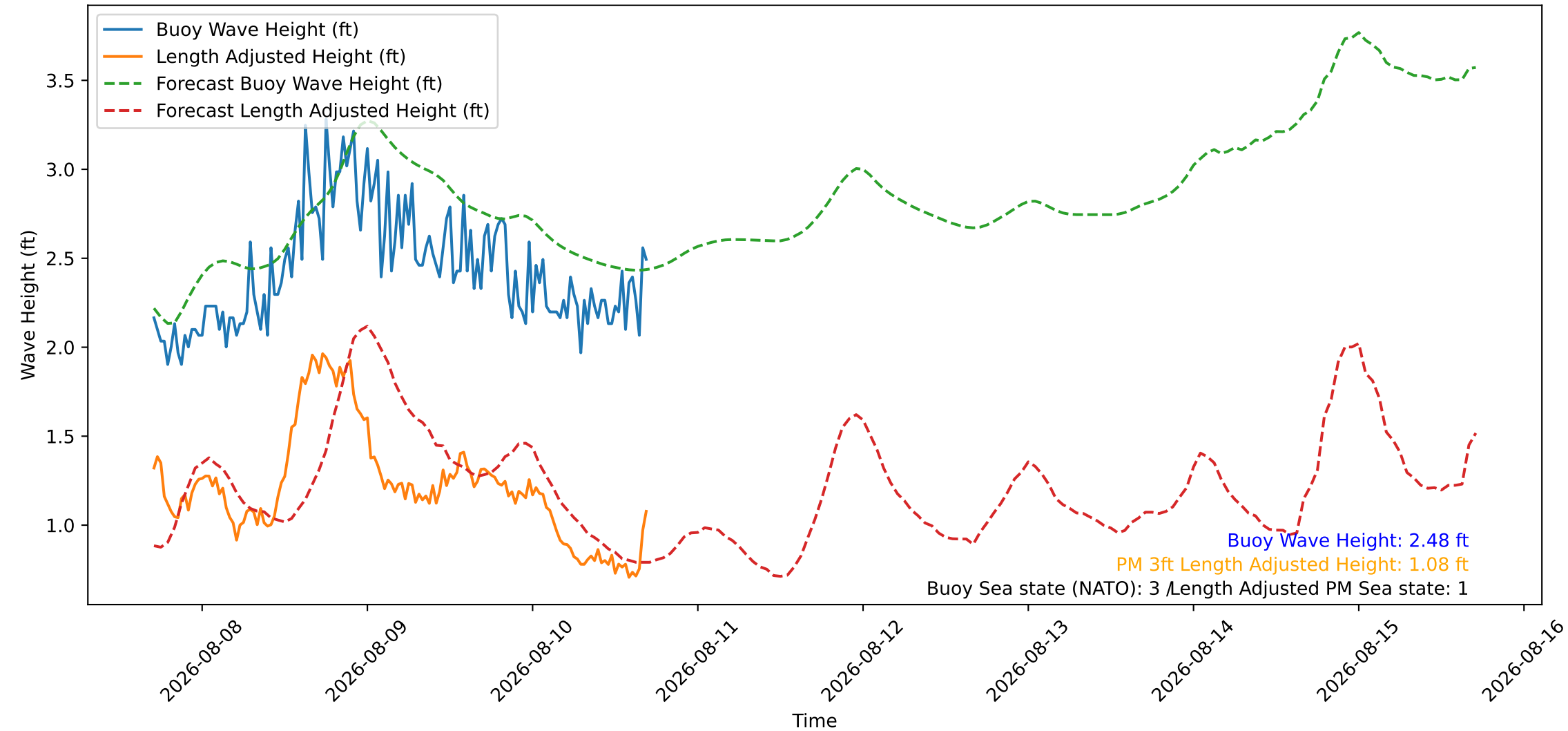
Wave Heights over Time for Oceanside Harbor at 2026-08-10 17:10:26
