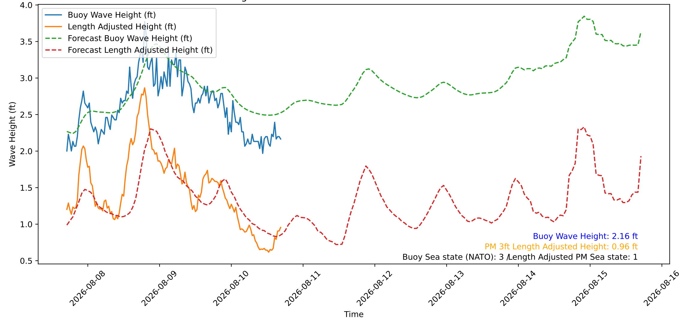
Wave Heights over Time for Green Beach at 2026-08-10 17:11:09
