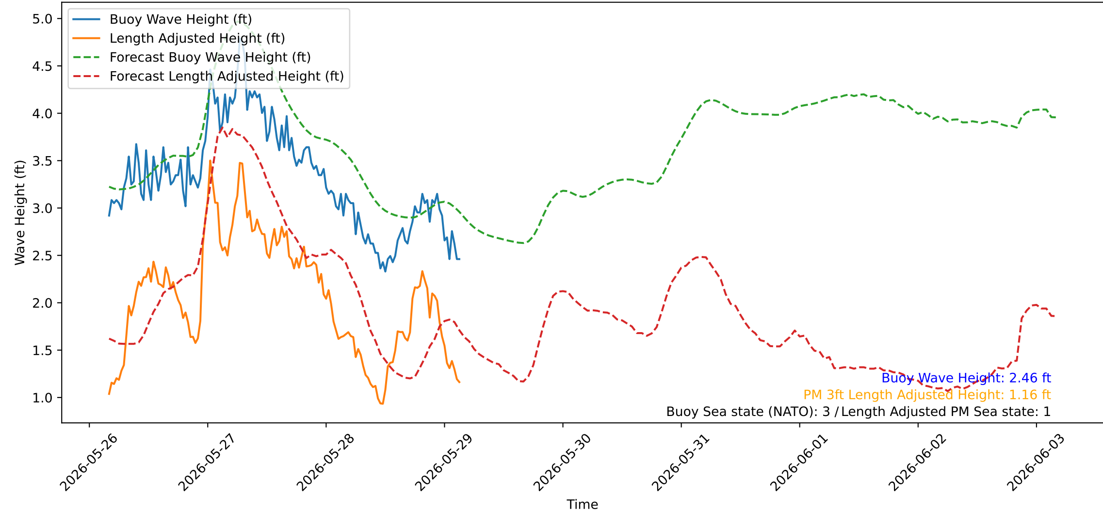
Wave Heights over Time for Red Beach at 2026-05-29 03:40:40
