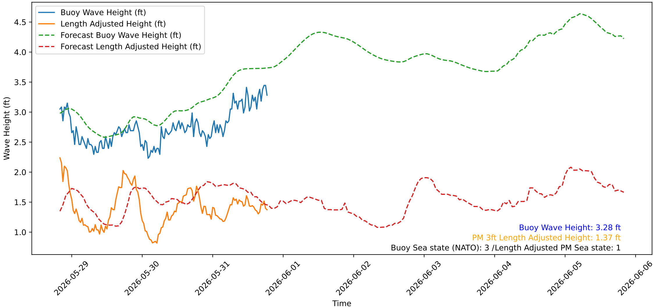
Wave Heights over Time for Red Beach at 2026-05-31 19:30:45
