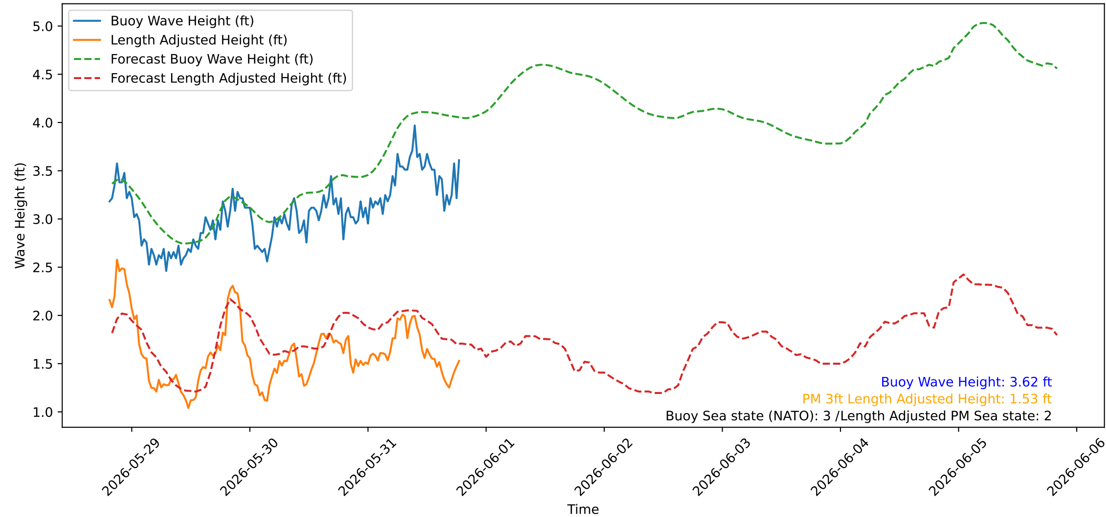
Wave Heights over Time for Green Beach at 2026-05-31 19:31:08
