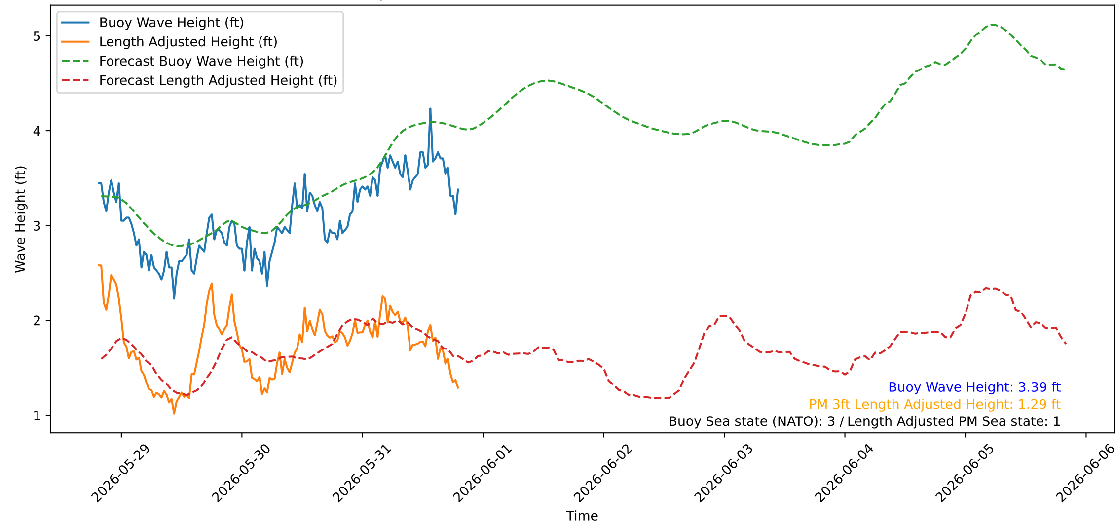
Wave Heights over Time for Oceanside Harbor at 2026-05-31 19:30:26
