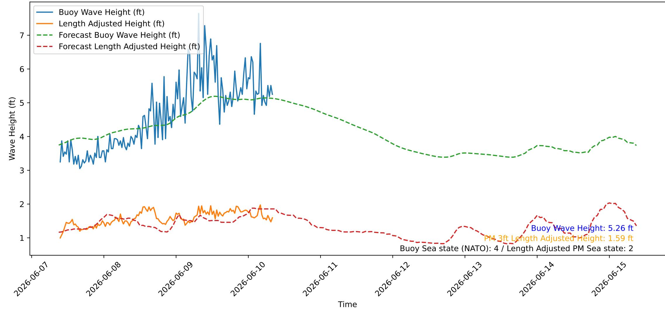
Wave Heights over Time for Red Beach at 2026-06-10 09:00:47
