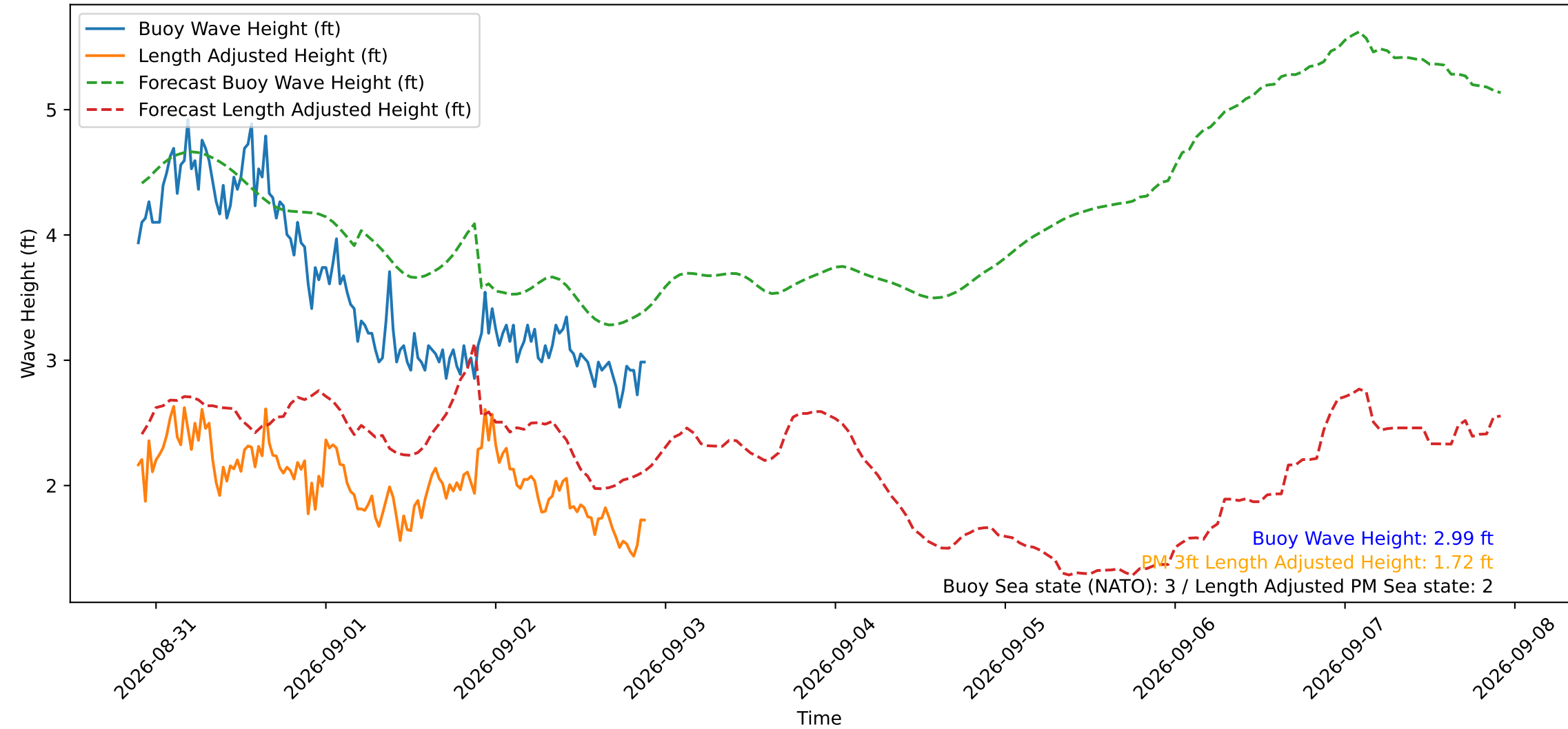
Wave Heights over Time for Oceanside Harbor at 2026-09-02 21:40:30
