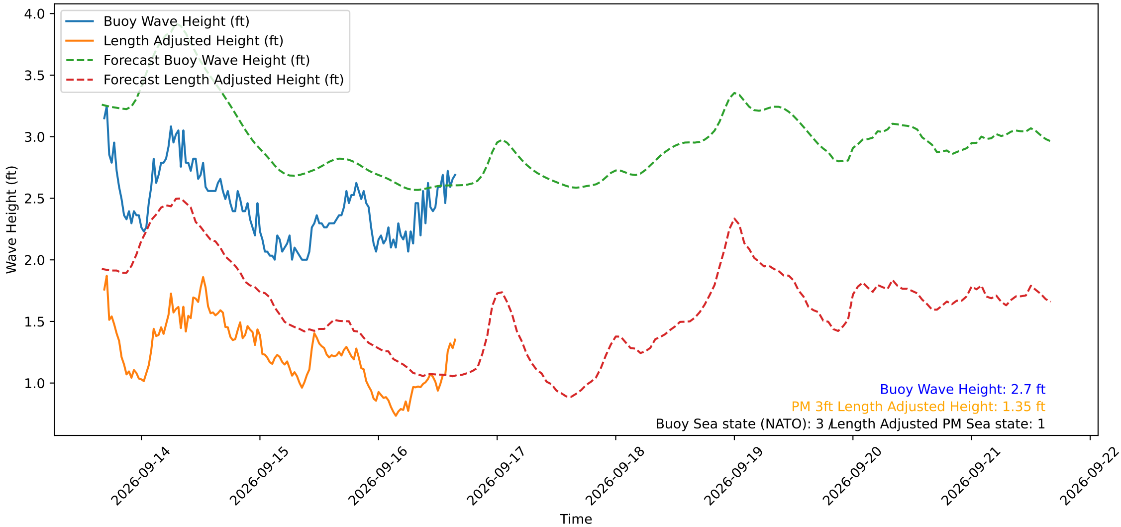
Wave Heights over Time for Red Beach at 2026-09-16 16:20:50
