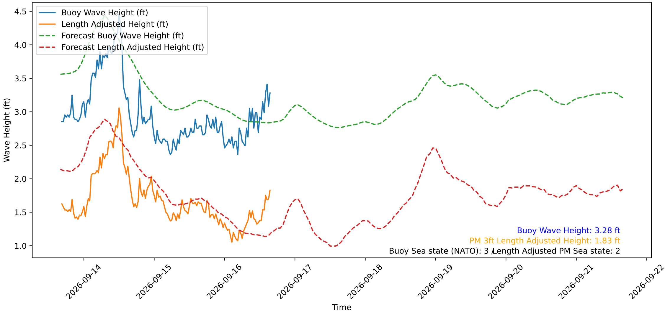
Wave Heights over Time for Oceanside Harbor at 2026-09-16 16:20:29
