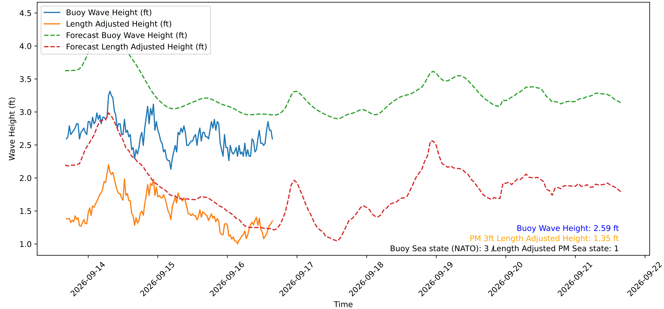
Wave Heights over Time for Green Beach at 2026-09-16 16:21:15
