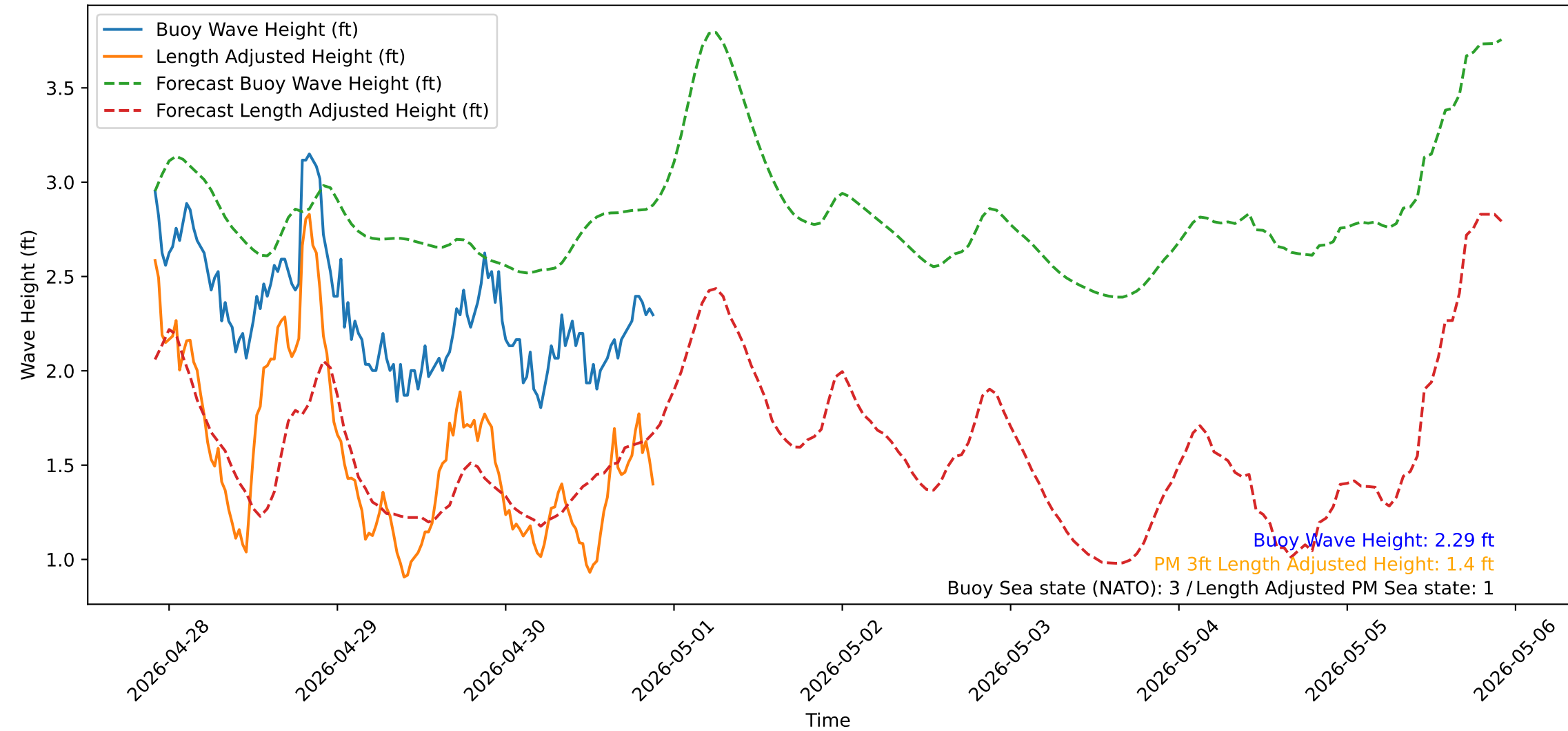
Wave Heights over Time for Green Beach at 2026-04-30 21:51:16
