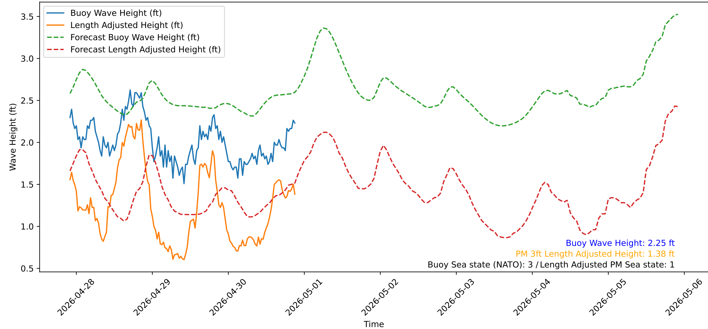
Wave Heights over Time for Red Beach at 2026-04-30 21:50:53
