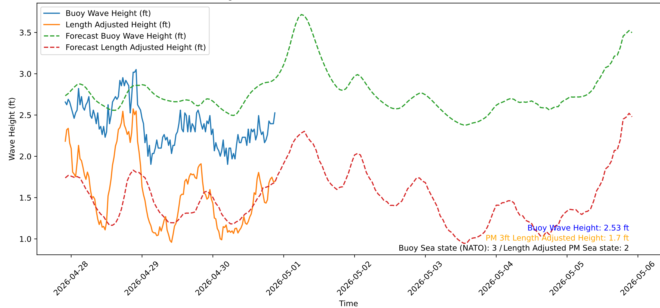
Wave Heights over Time for Oceanside Harbor at 2026-04-30 21:50:32
