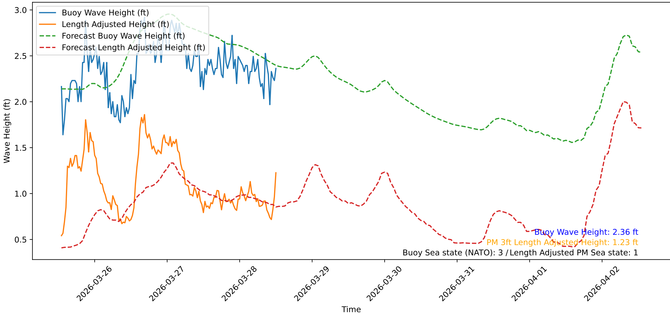
Wave Heights over Time for Oceanside Harbor at 2026-03-28 12:50:31
