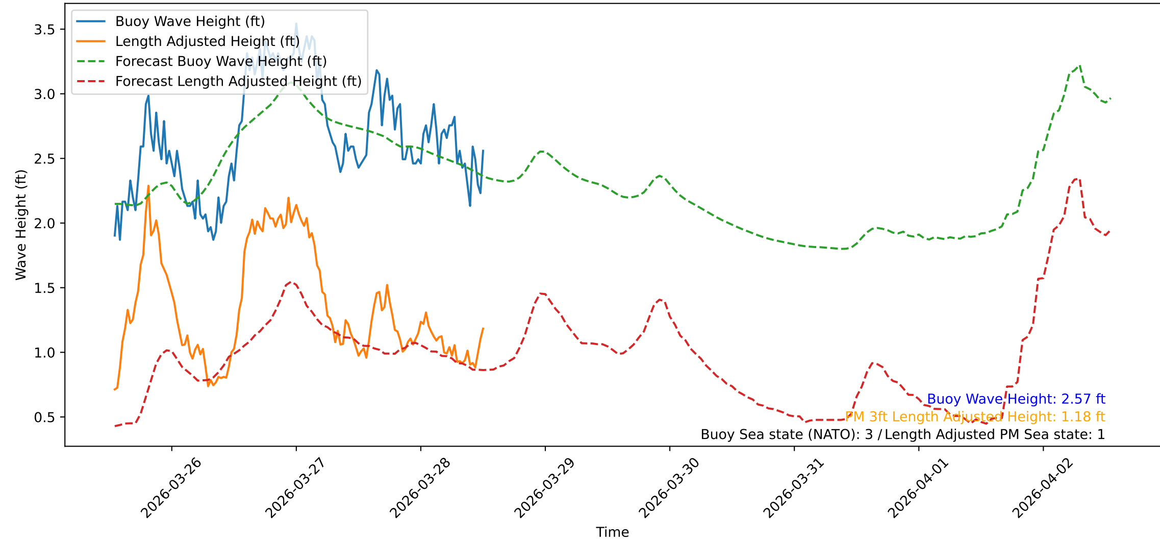
Wave Heights over Time for Green Beach at 2026-03-28 12:51:08
