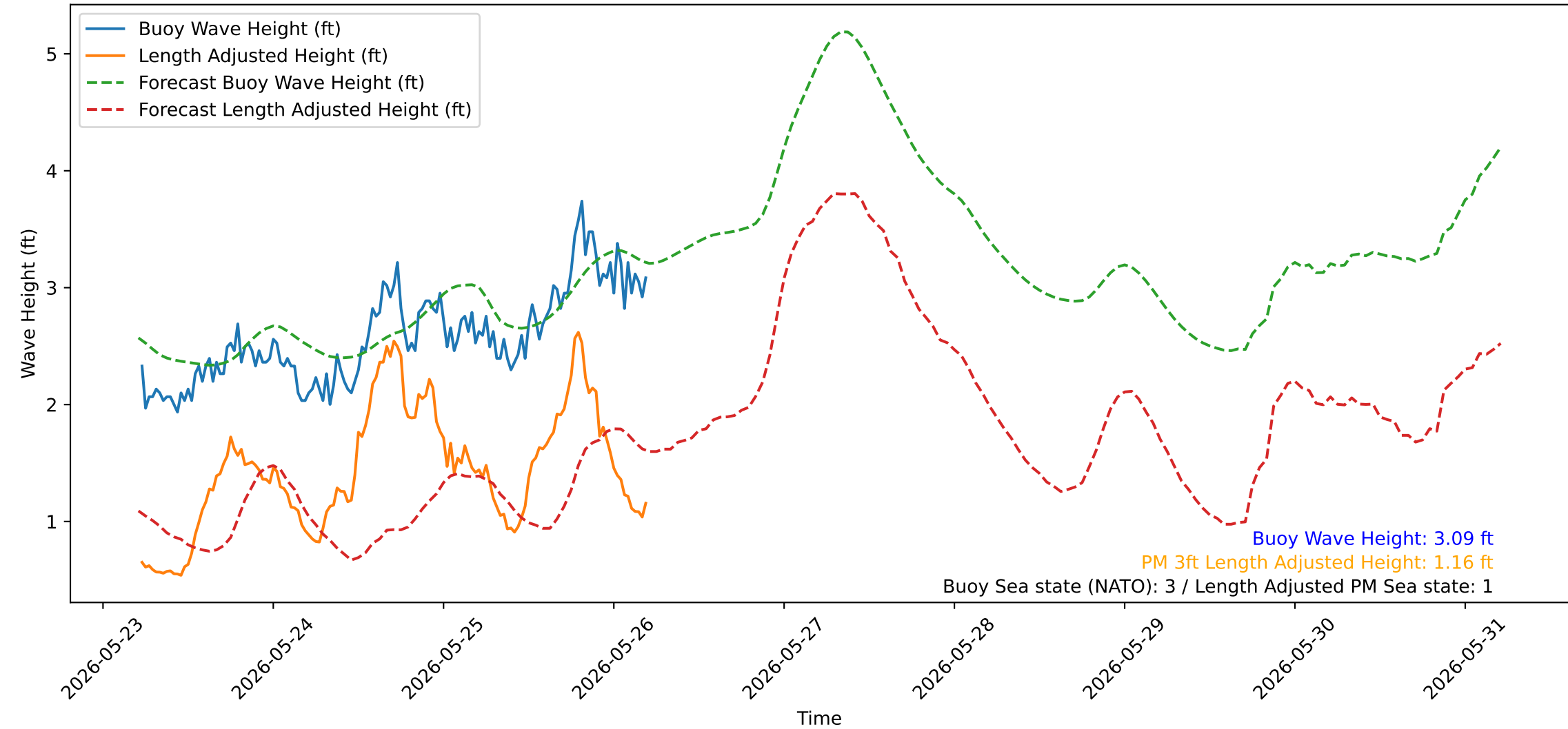
Wave Heights over Time for Red Beach at 2026-05-26 05:20:50
