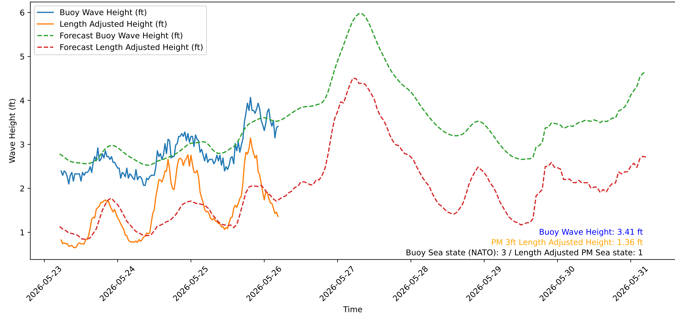
Wave Heights over Time for Green Beach at 2026-05-26 05:21:12
