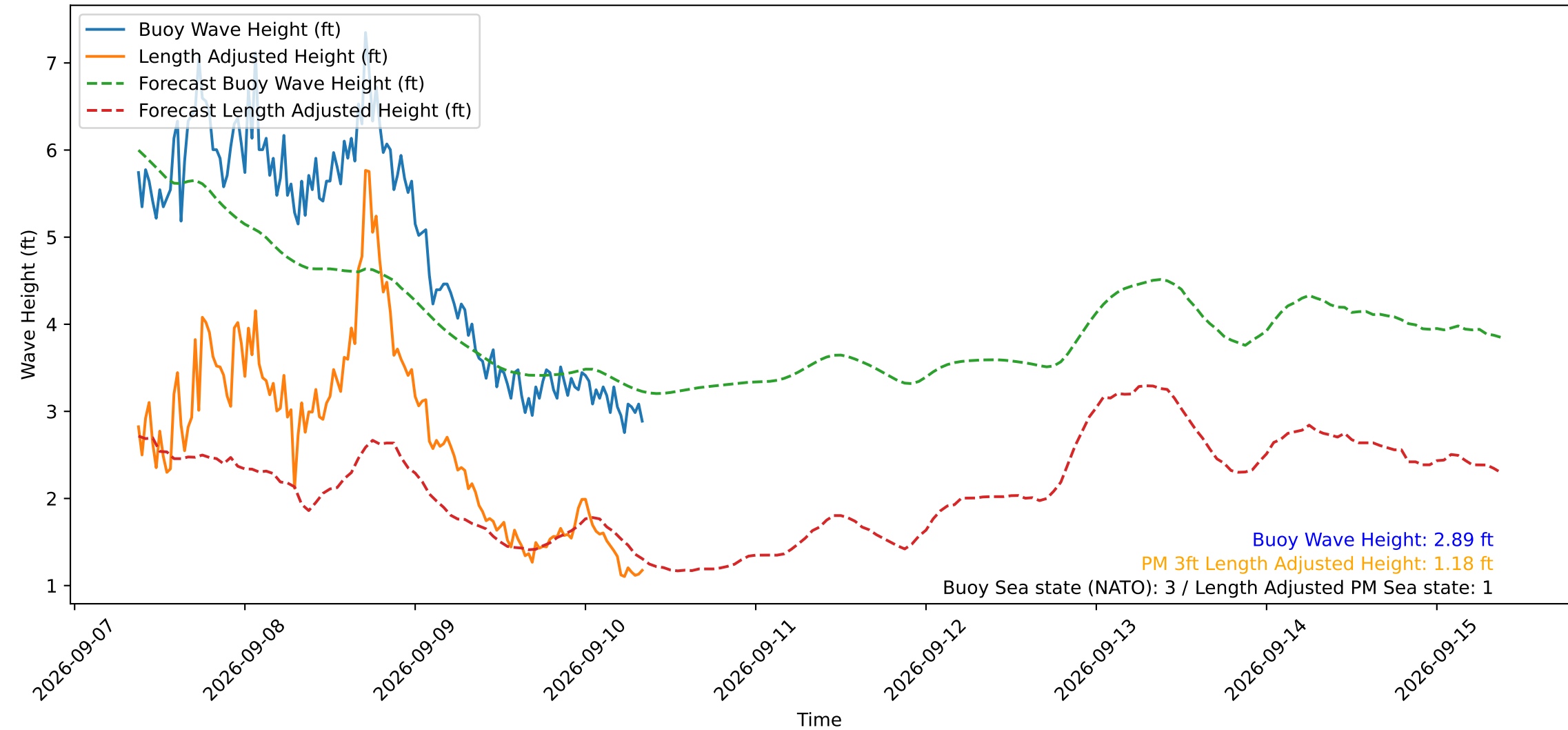
Wave Heights over Time for Oceanside Harbor at 2026-09-10 09:00:29
