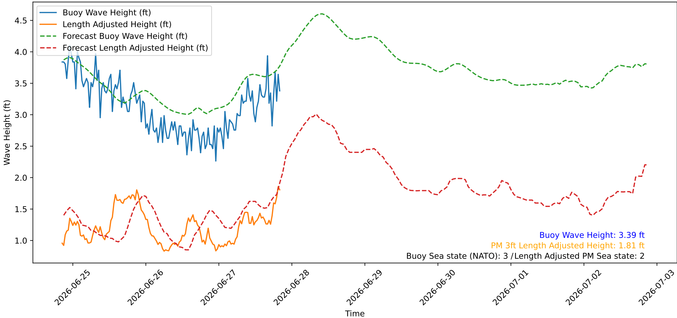
Wave Heights over Time for Green Beach at 2026-06-27 20:41:09
