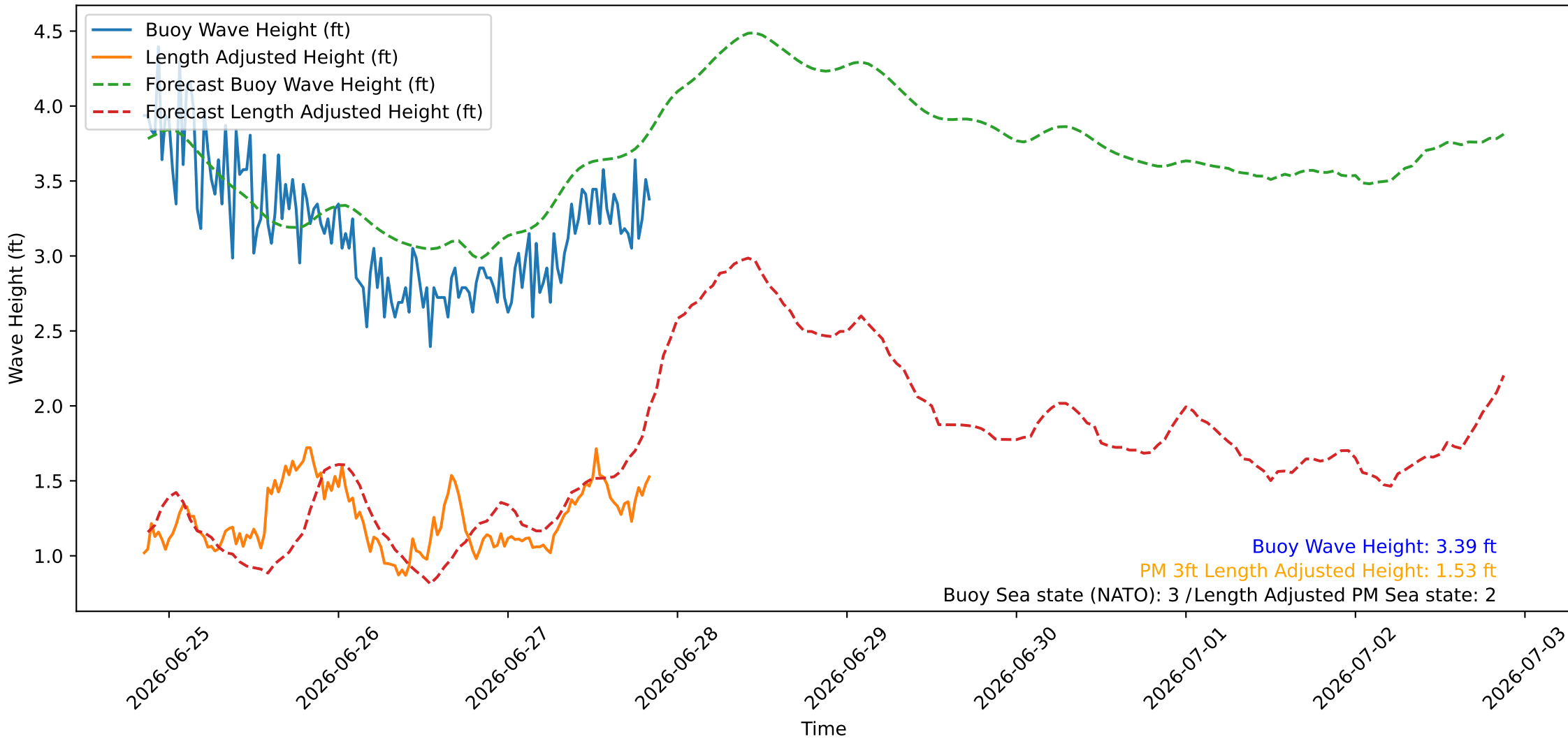
Wave Heights over Time for Oceanside Harbor at 2026-06-27 20:40:26
