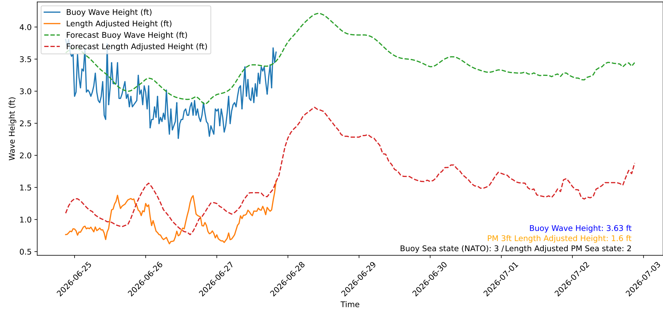
Wave Heights over Time for Red Beach at 2026-06-27 20:40:46
