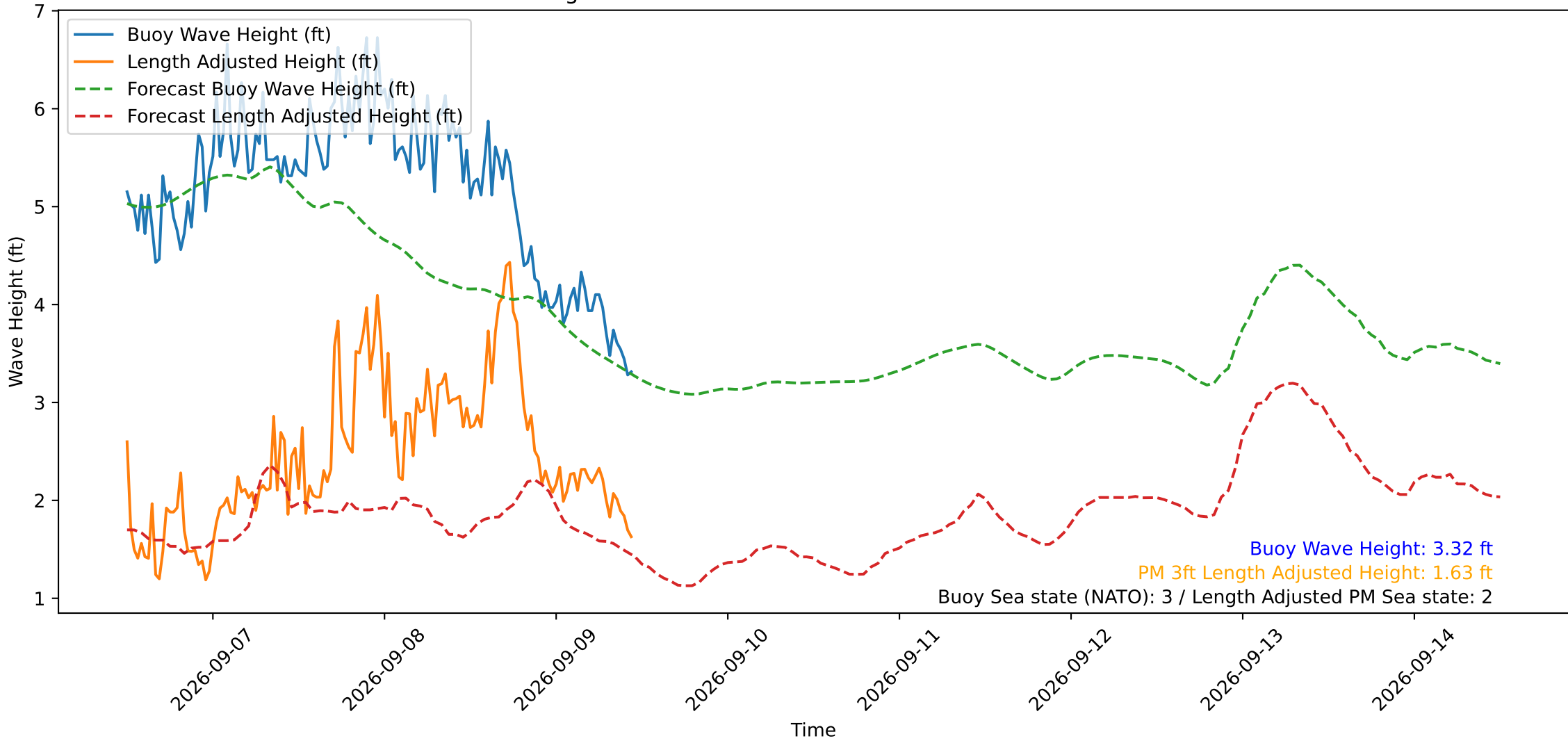
Wave Heights over Time for Red Beach at 2026-09-09 11:30:48
