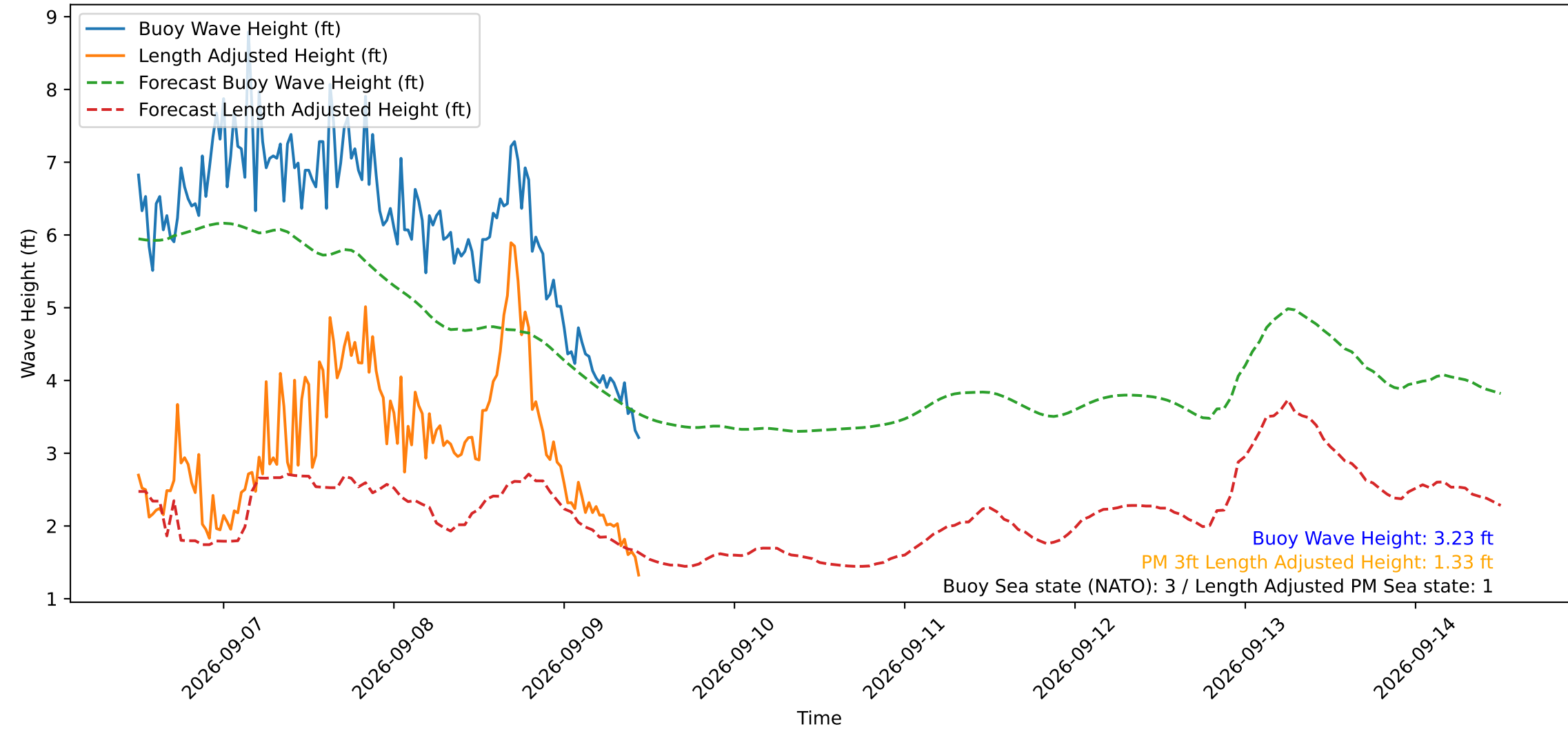
Wave Heights over Time for Green Beach at 2026-09-09 11:31:11
