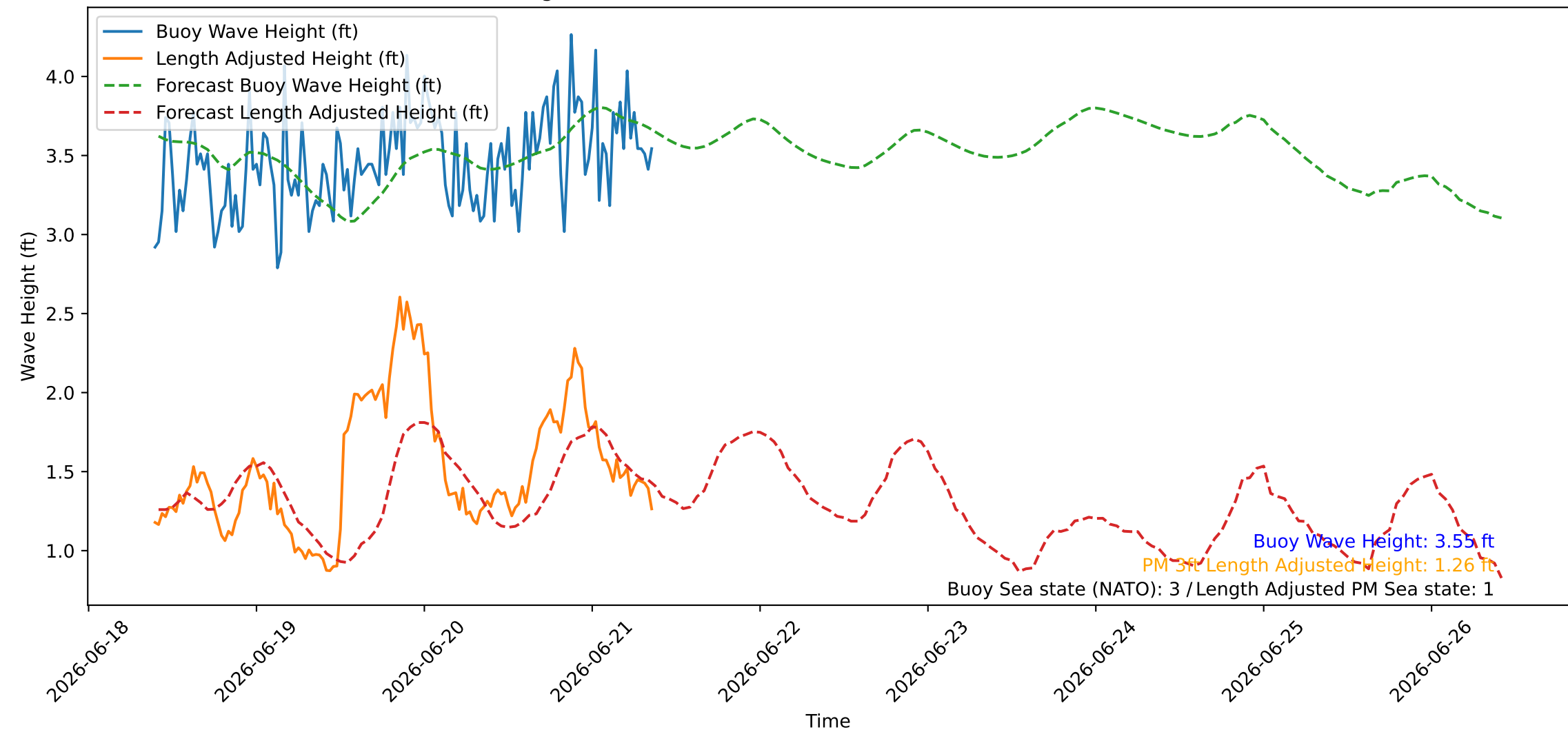
Wave Heights over Time for Oceanside Harbor at 2026-06-21 09:30:26
