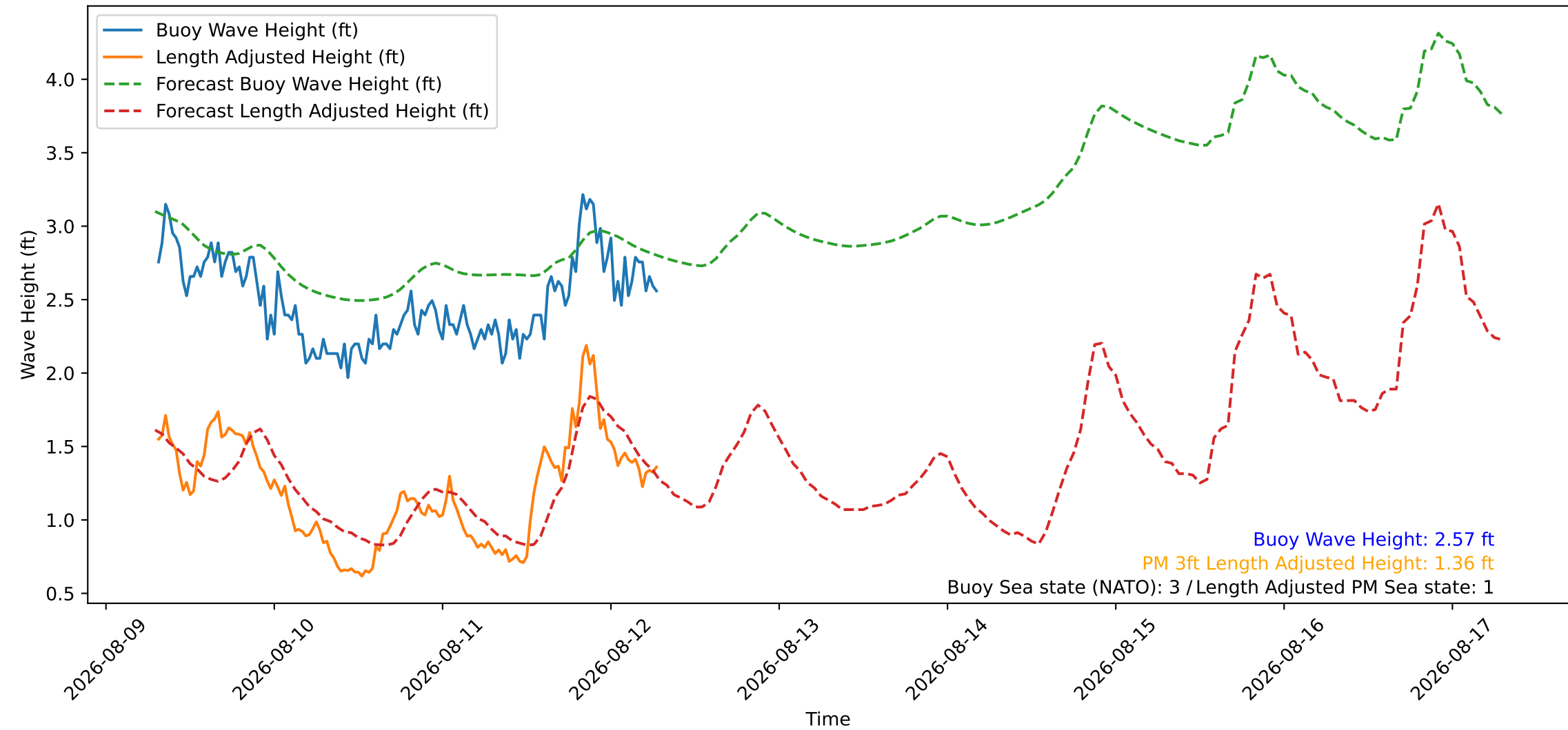
Wave Heights over Time for Green Beach at 2026-08-12 07:21:10
