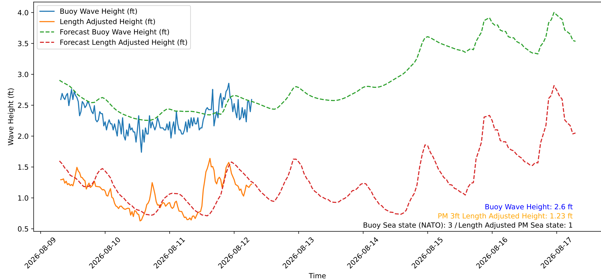
Wave Heights over Time for Red Beach at 2026-08-12 07:20:47
