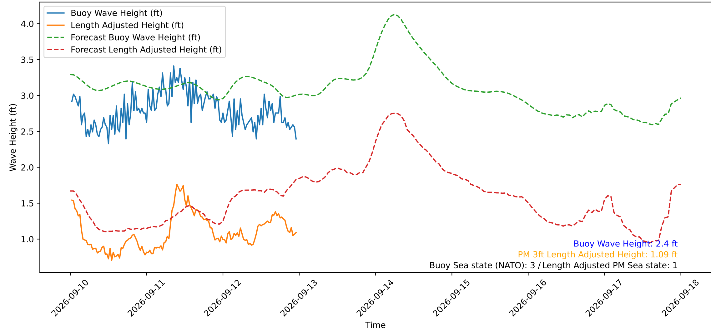
Wave Heights over Time for Red Beach at 2026-09-13 00:00:48
