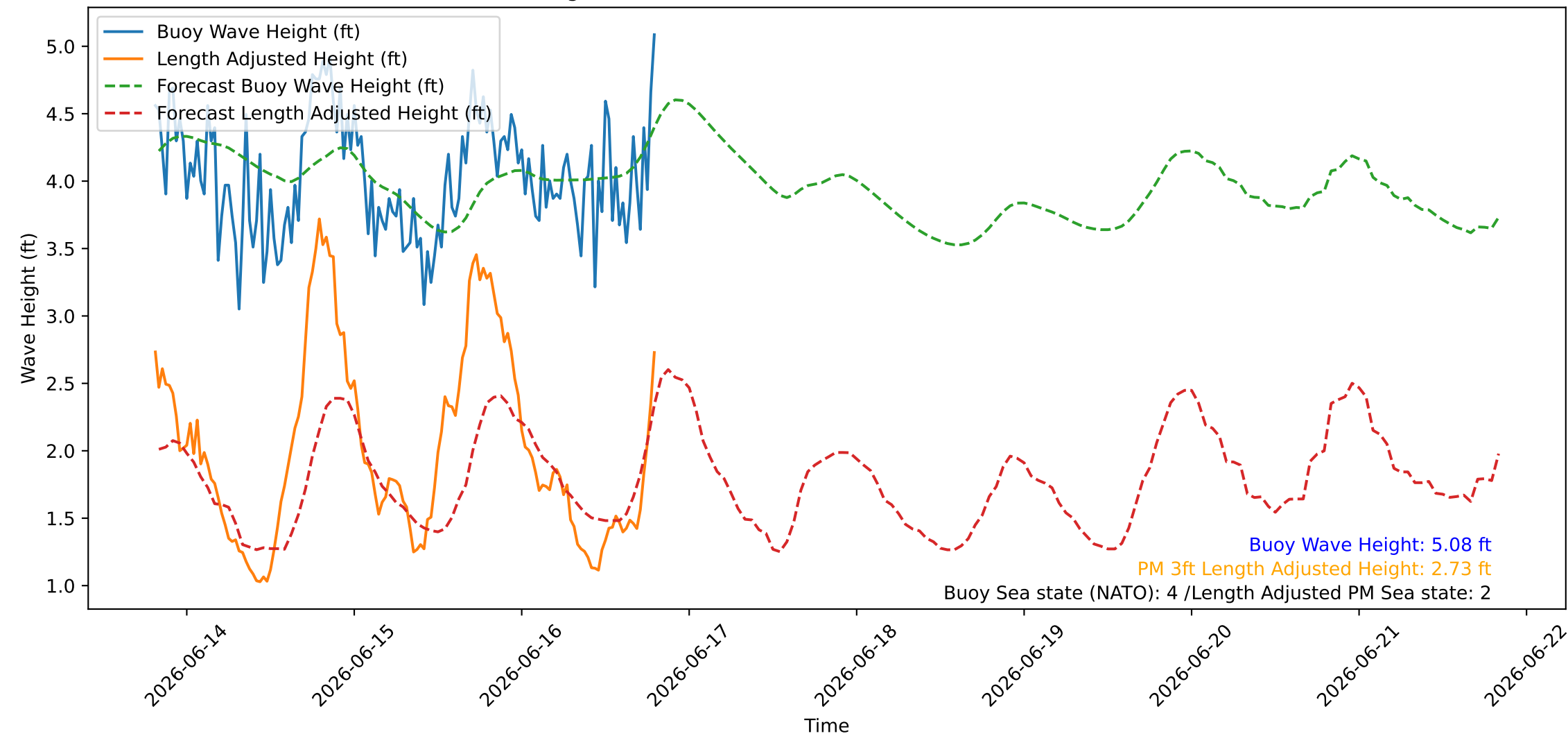
Wave Heights over Time for Green Beach at 2026-06-16 19:41:09
