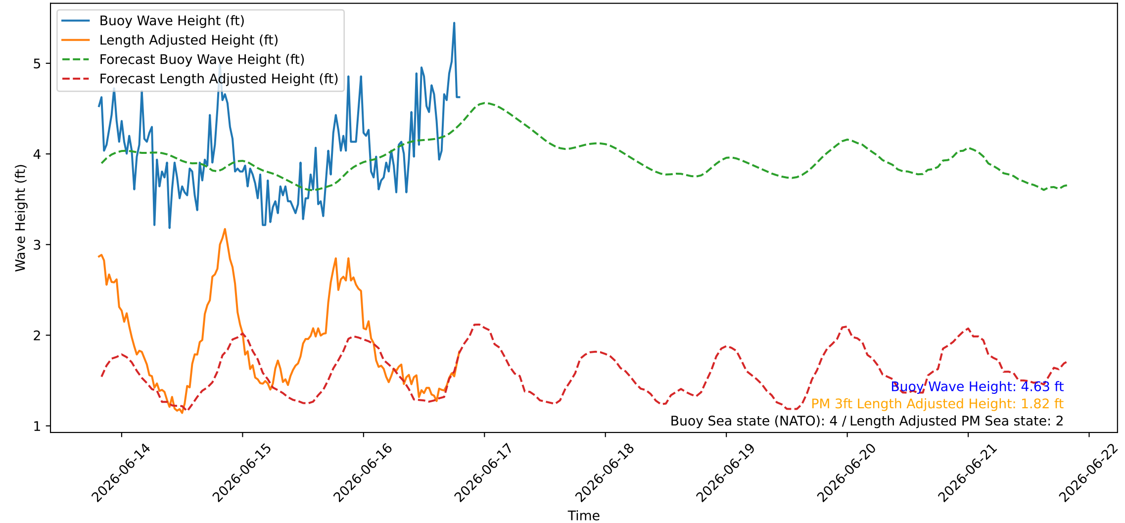
Wave Heights over Time for Oceanside Harbor at 2026-06-16 19:40:26
