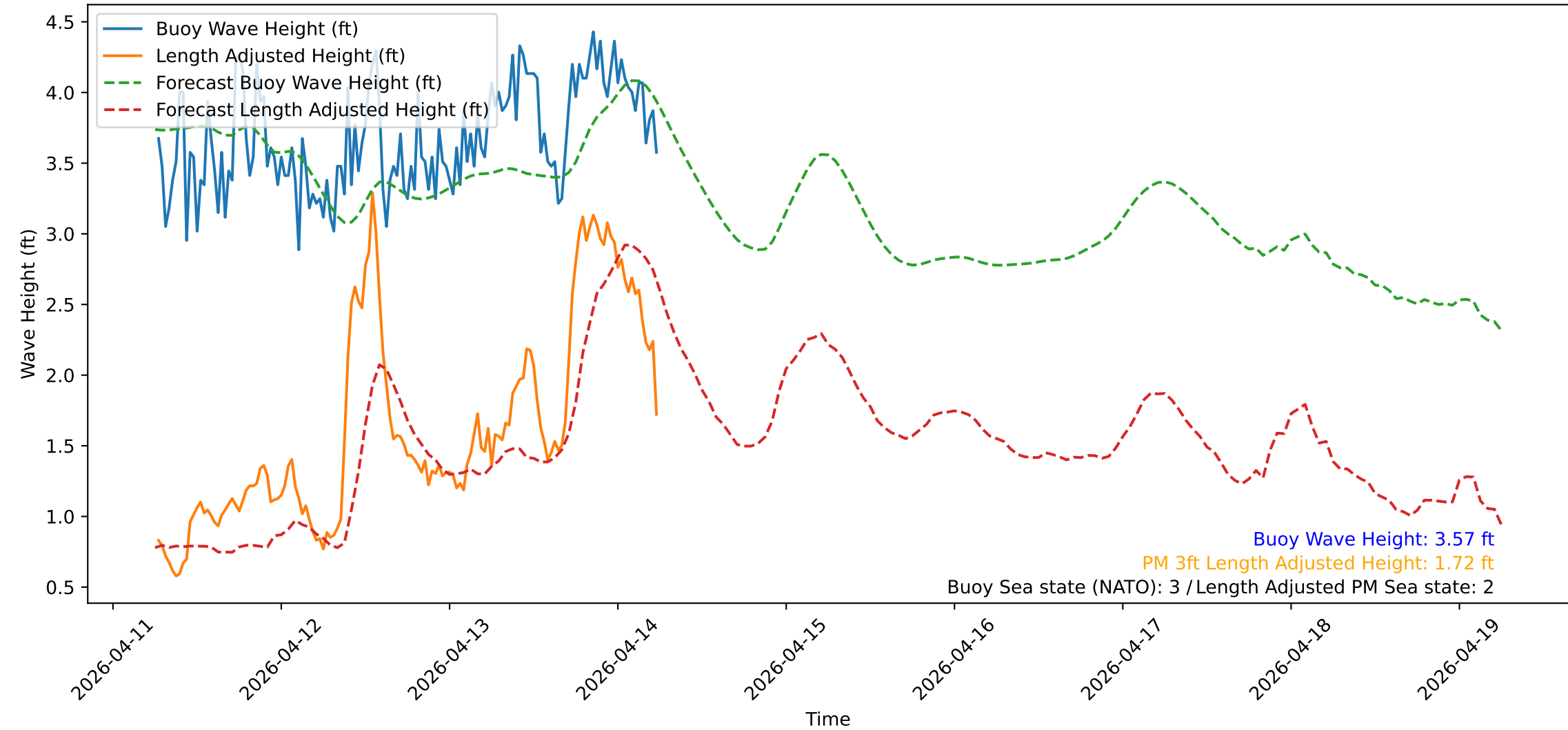
Wave Heights over Time for Red Beach at 2026-04-14 06:20:51
