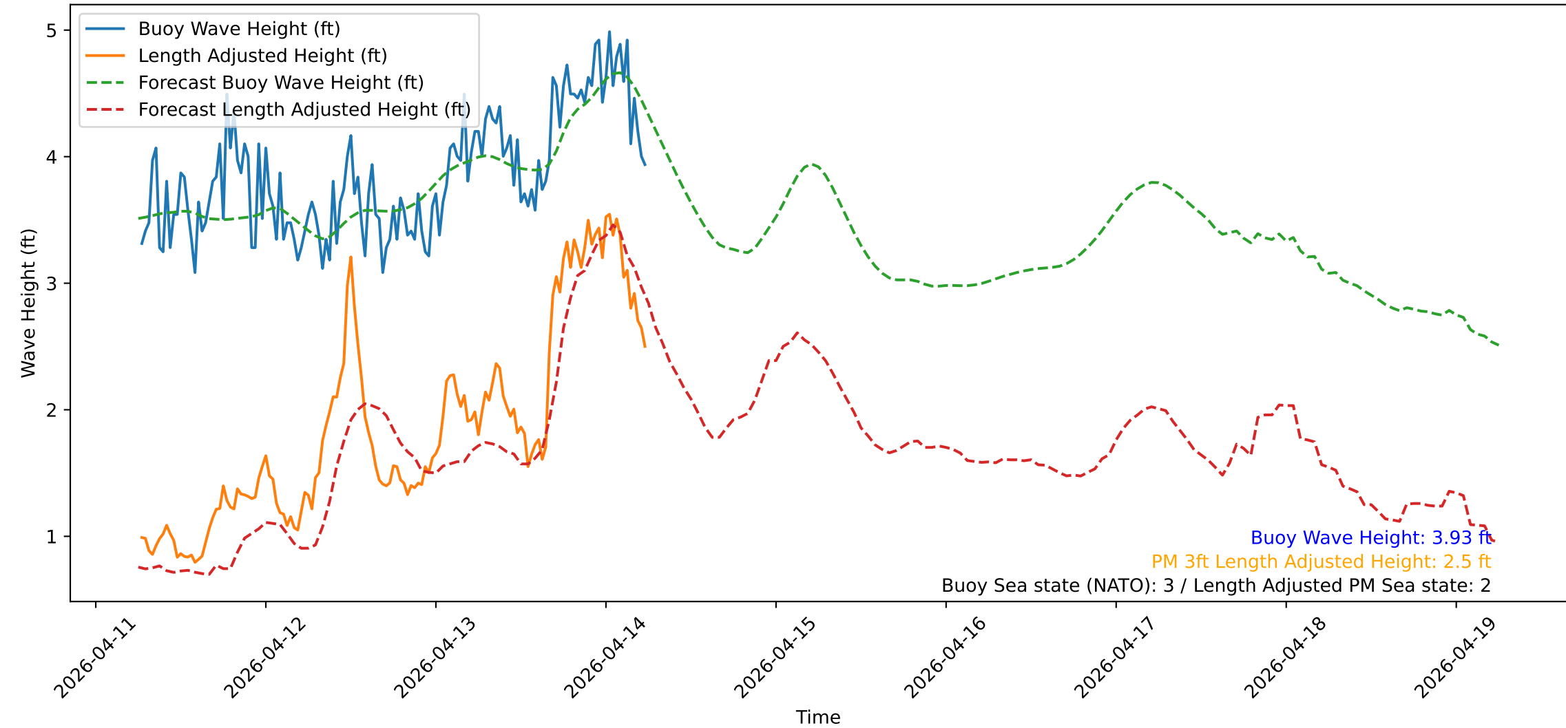
Wave Heights over Time for Green Beach at 2026-04-14 06:21:14
