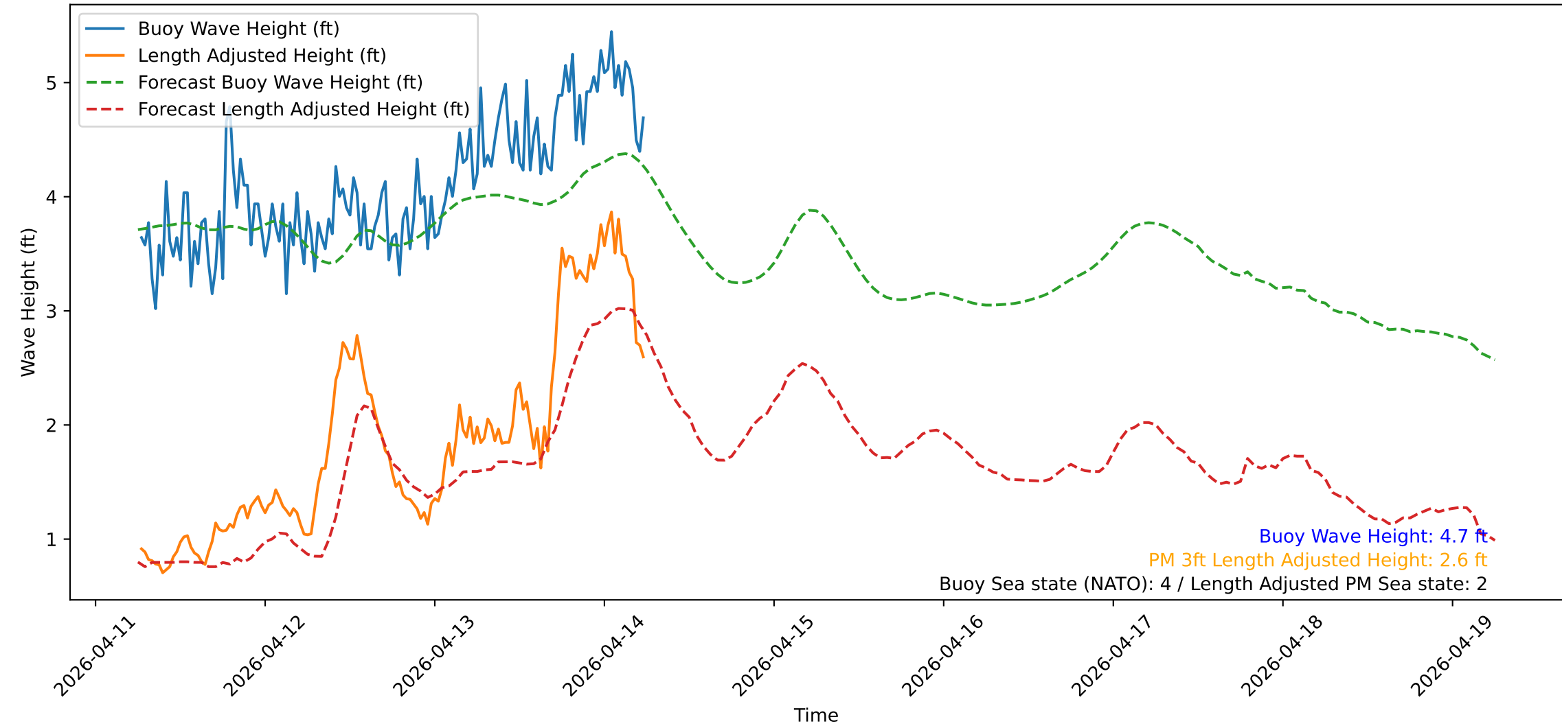
Wave Heights over Time for Oceanside Harbor at 2026-04-14 06:20:31
