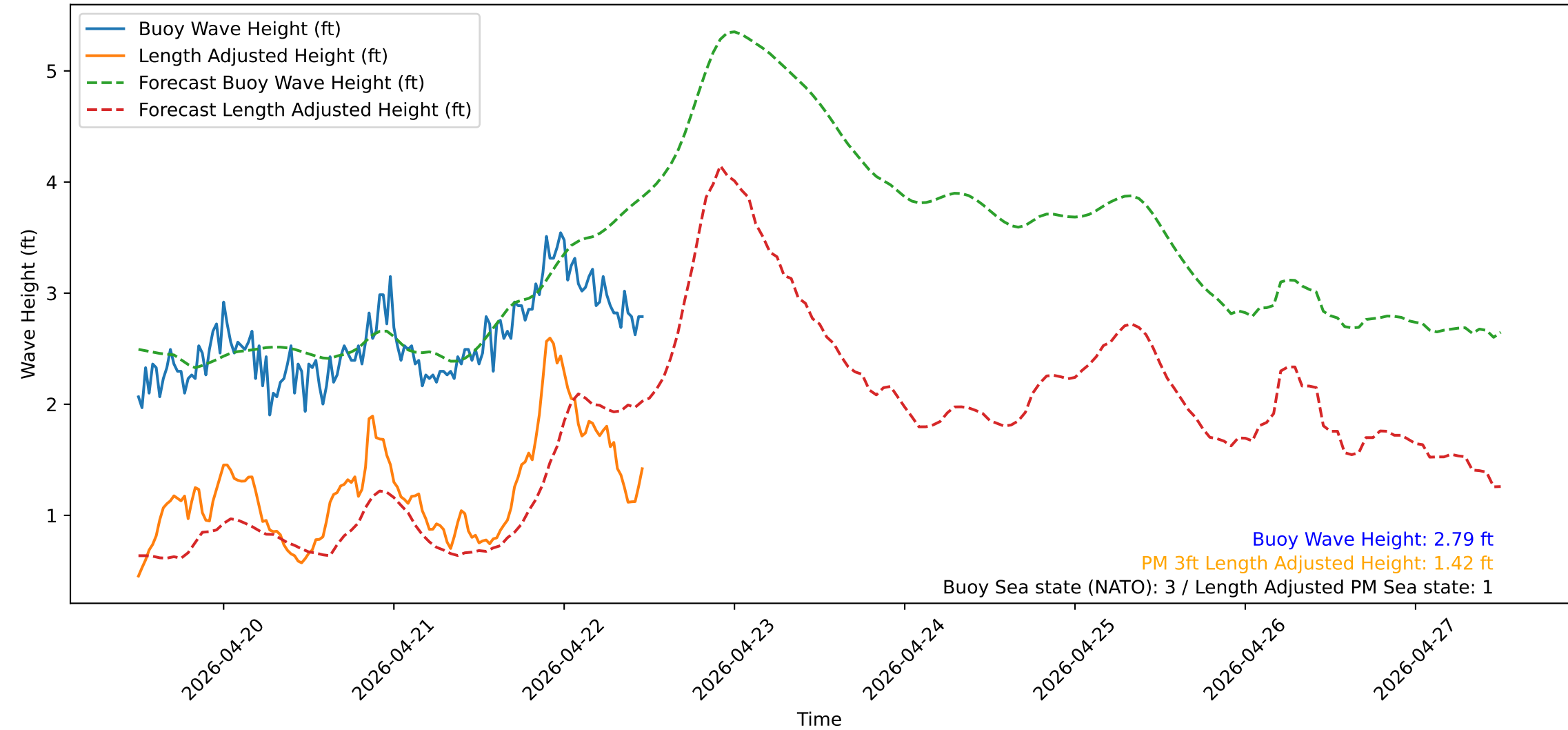
Wave Heights over Time for Green Beach at 2026-04-22 11:51:13
