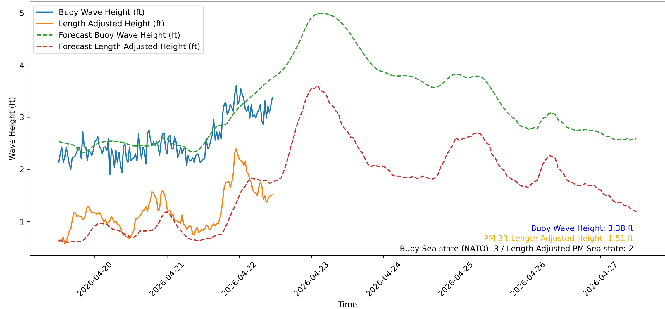
Wave Heights over Time for Oceanside Harbor at 2026-04-22 11:50:31
