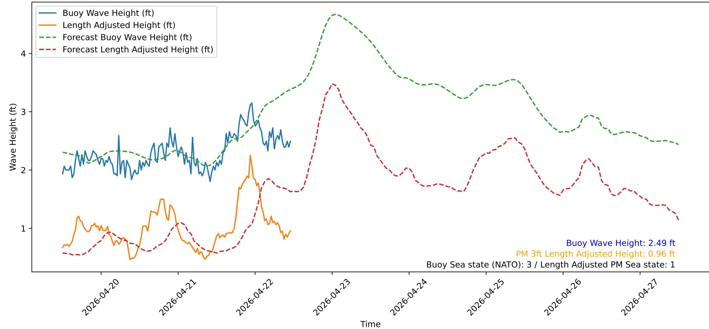
Wave Heights over Time for Red Beach at 2026-04-22 11:50:51
