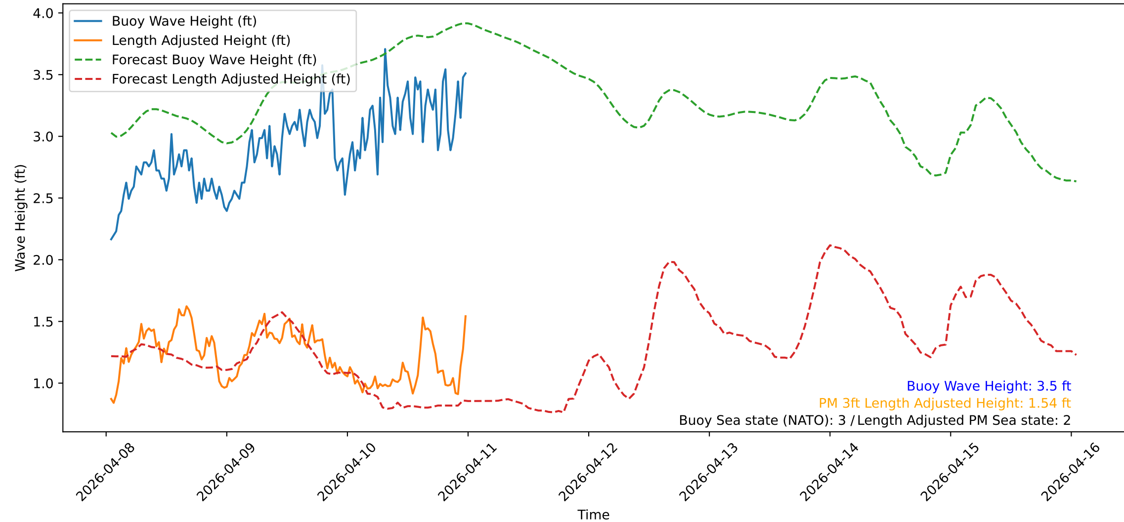
Wave Heights over Time for Red Beach at 2026-04-11 00:40:51
