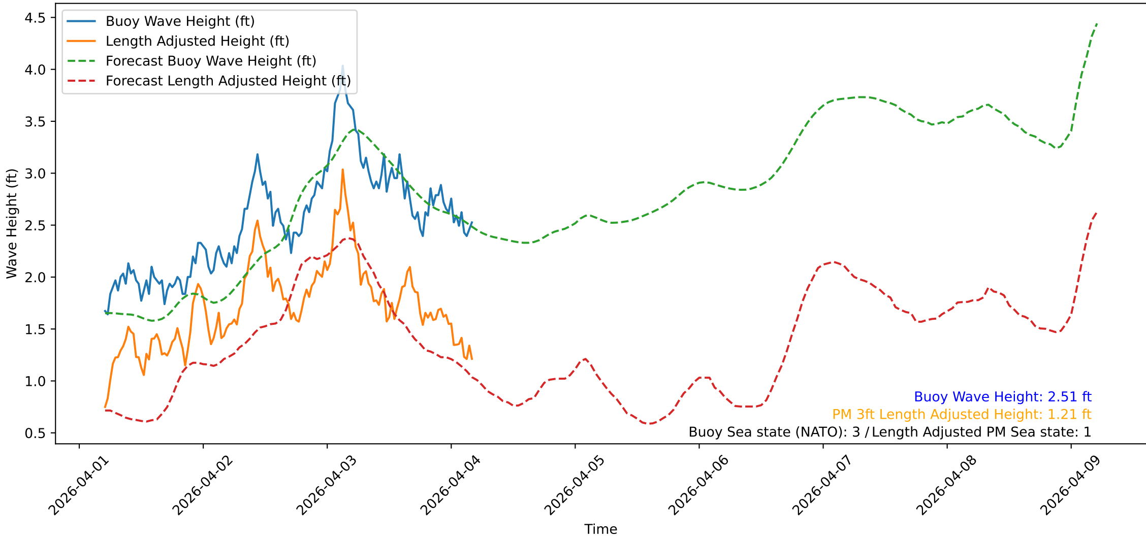
Wave Heights over Time for Oceanside Harbor at 2026-04-04 05:10:31
