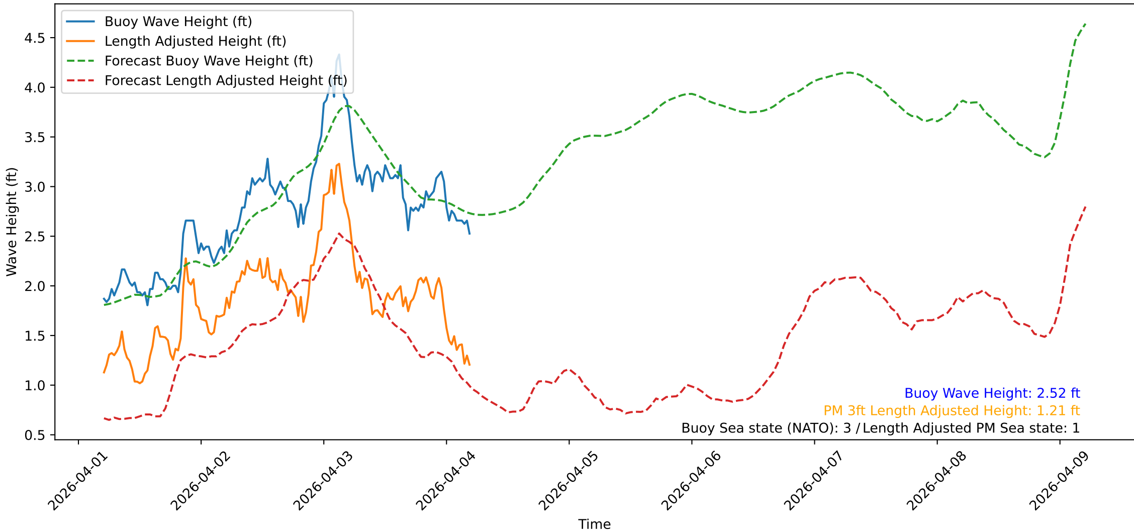
Wave Heights over Time for Green Beach at 2026-04-04 05:11:09
