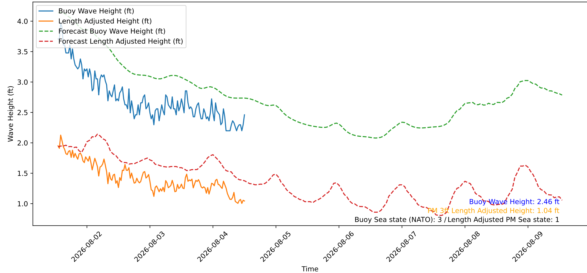
Wave Heights over Time for Oceanside Harbor at 2026-08-04 12:50:26
