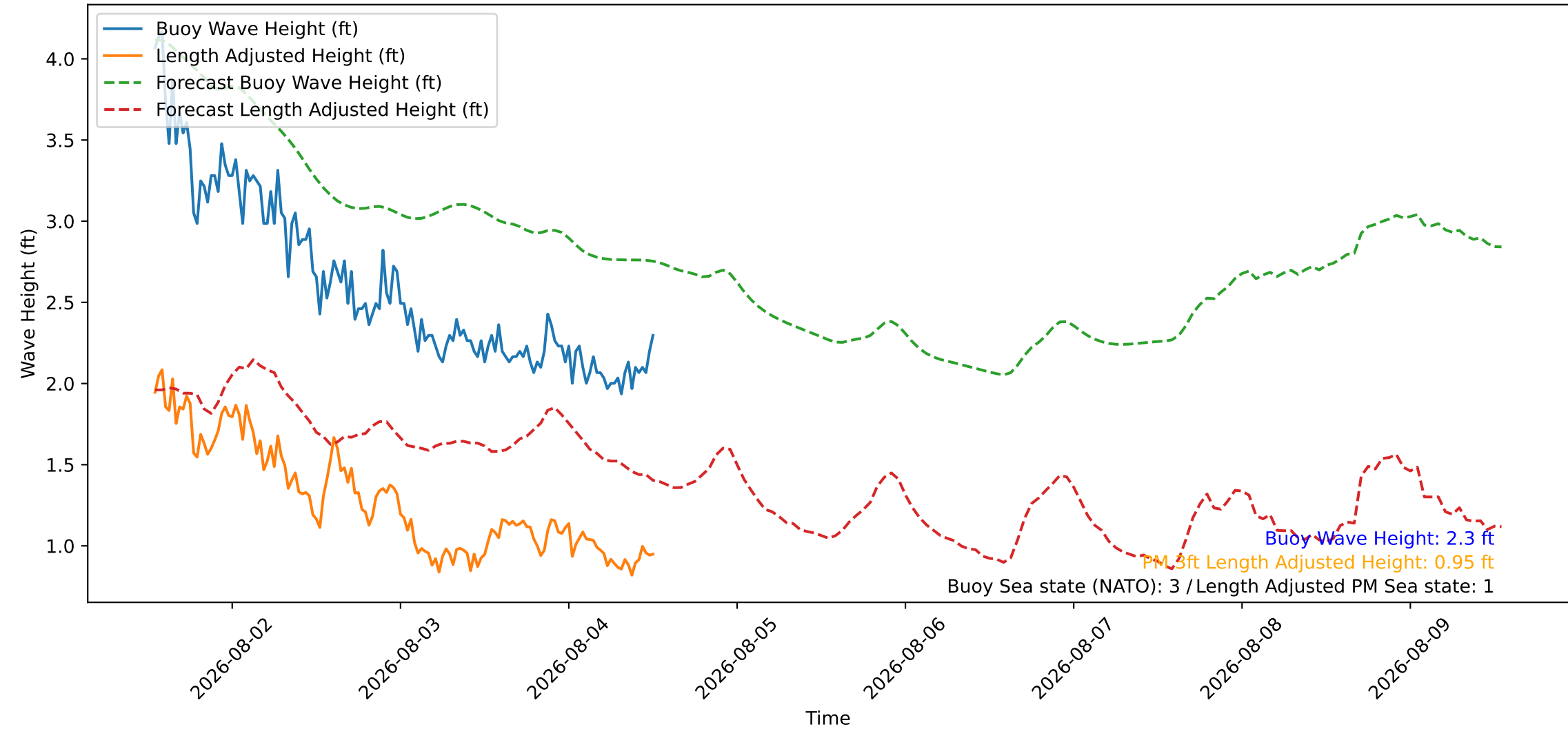
Wave Heights over Time for Green Beach at 2026-08-04 12:51:09
