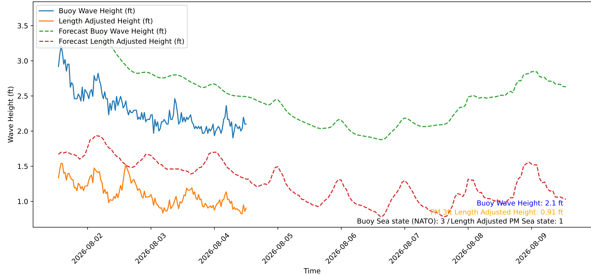
Wave Heights over Time for Red Beach at 2026-08-04 12:50:47
