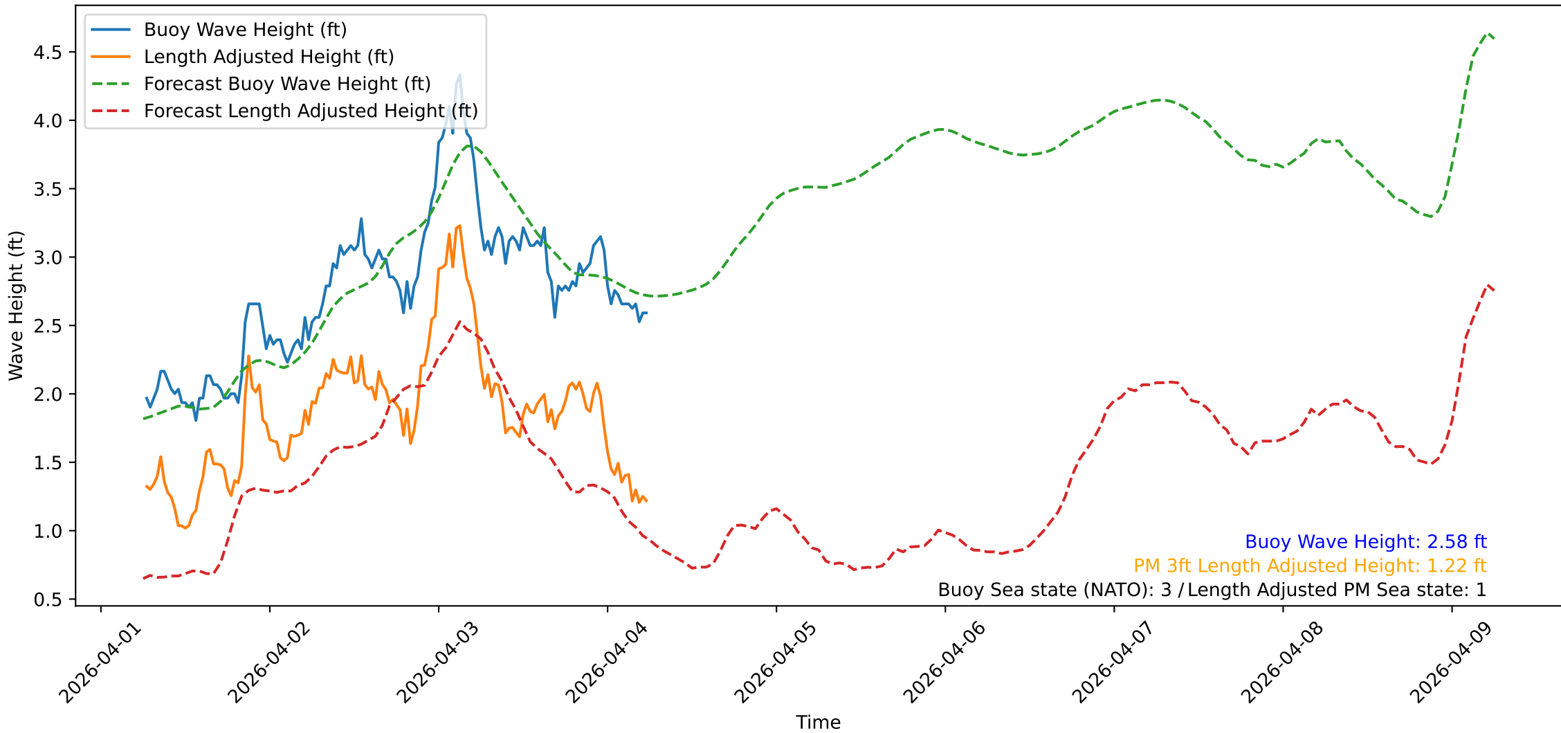
Wave Heights over Time for Green Beach at 2026-04-04 06:21:10
