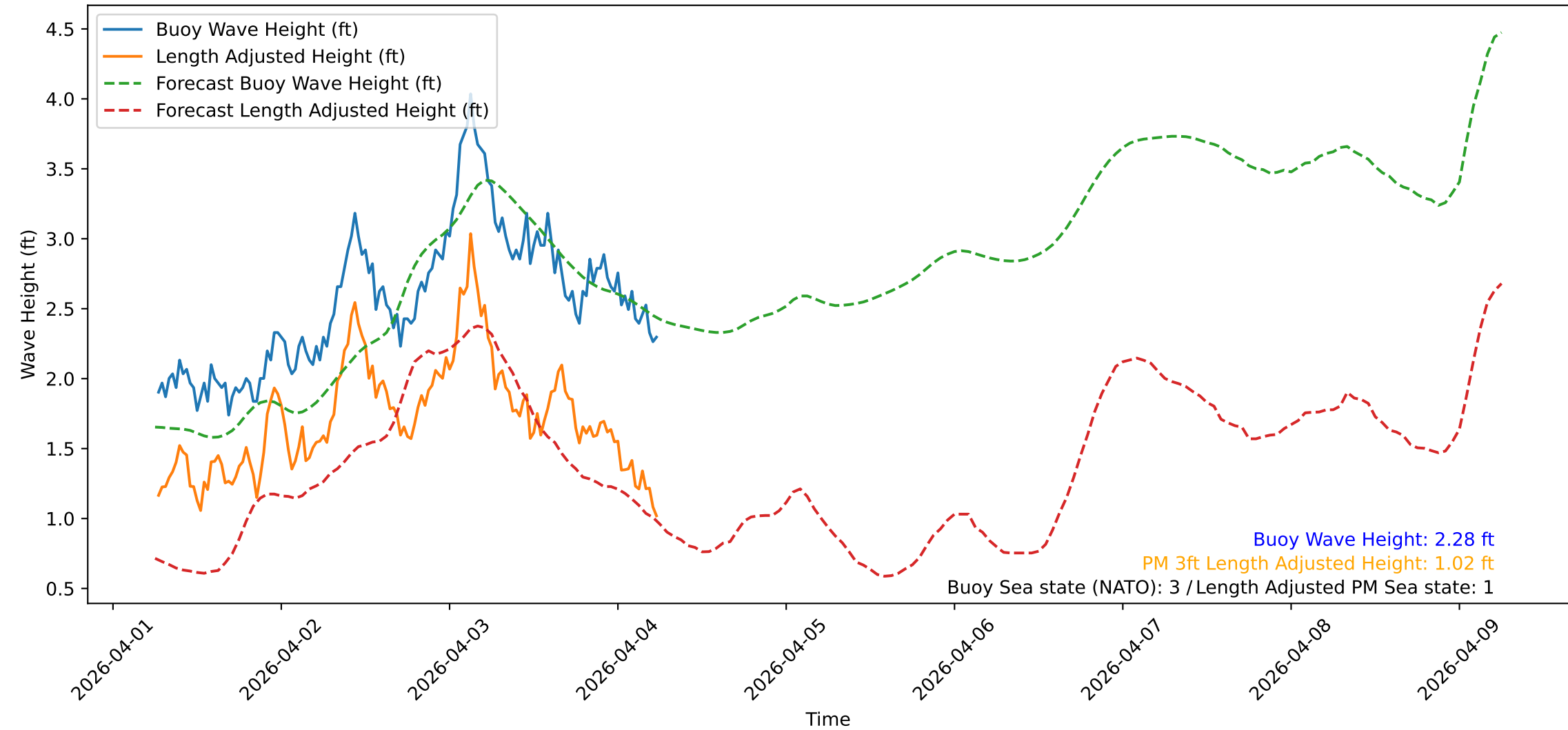
Wave Heights over Time for Oceanside Harbor at 2026-04-04 06:20:31
