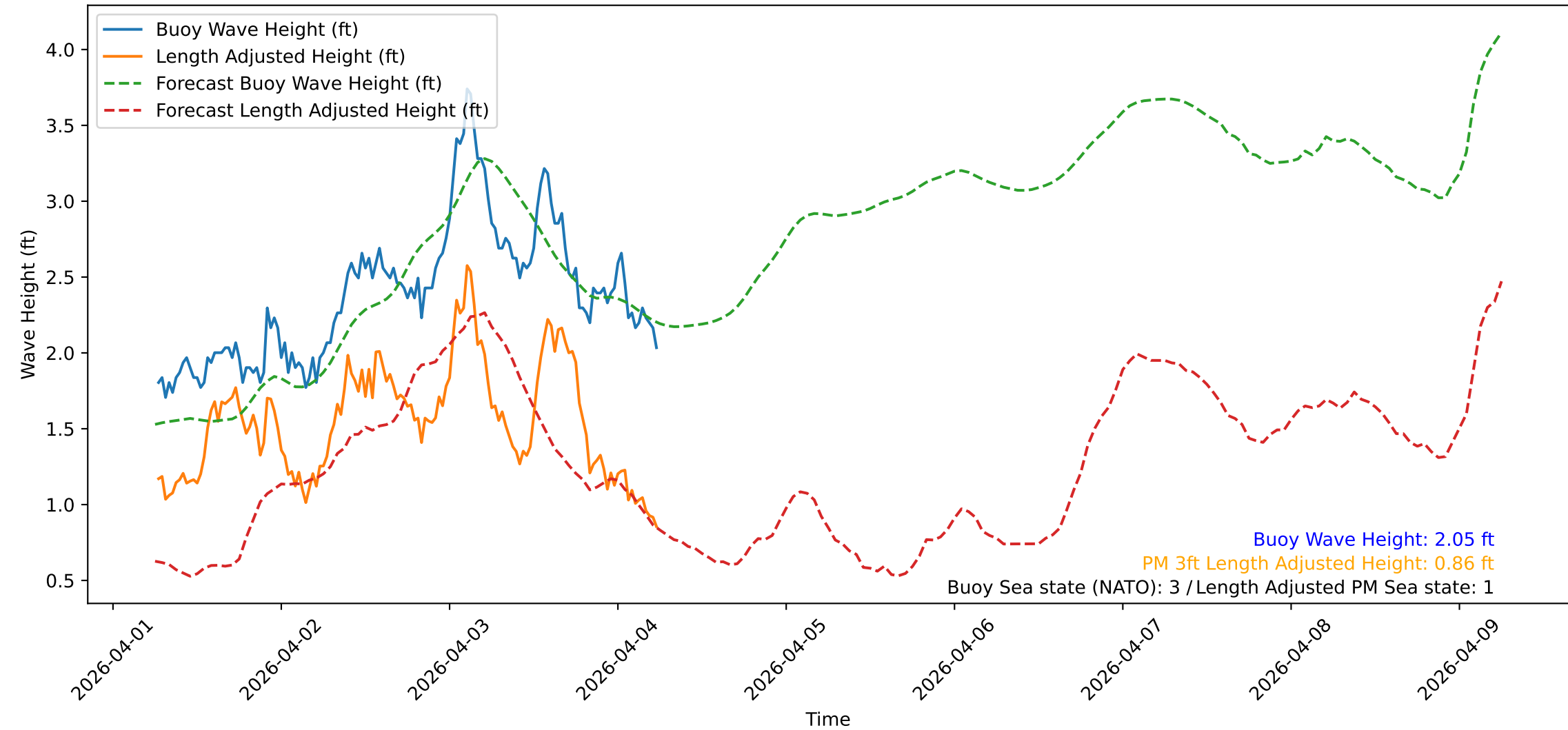
Wave Heights over Time for Red Beach at 2026-04-04 06:20:48
