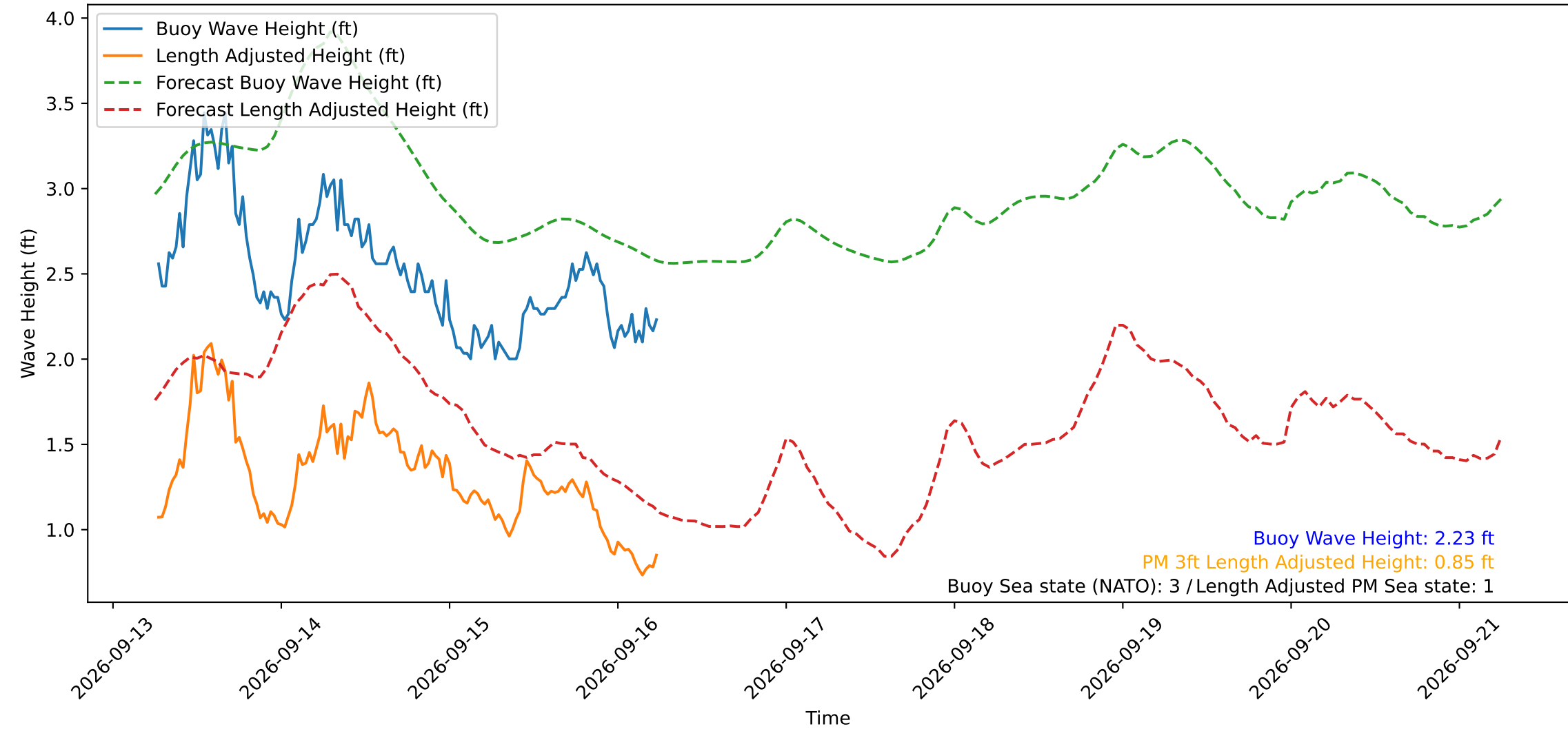
Wave Heights over Time for Red Beach at 2026-09-16 06:20:50
