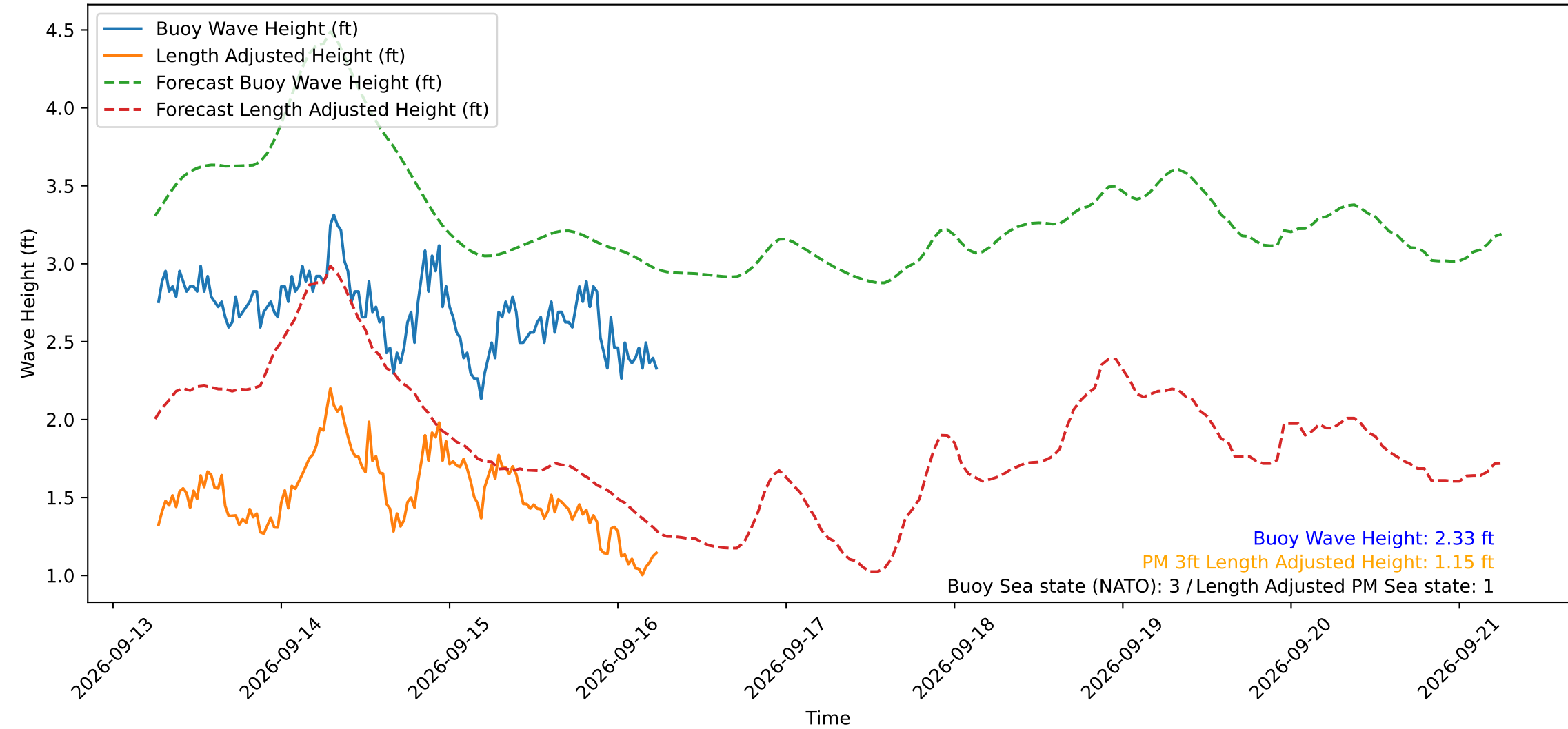
Wave Heights over Time for Green Beach at 2026-09-16 06:21:14
