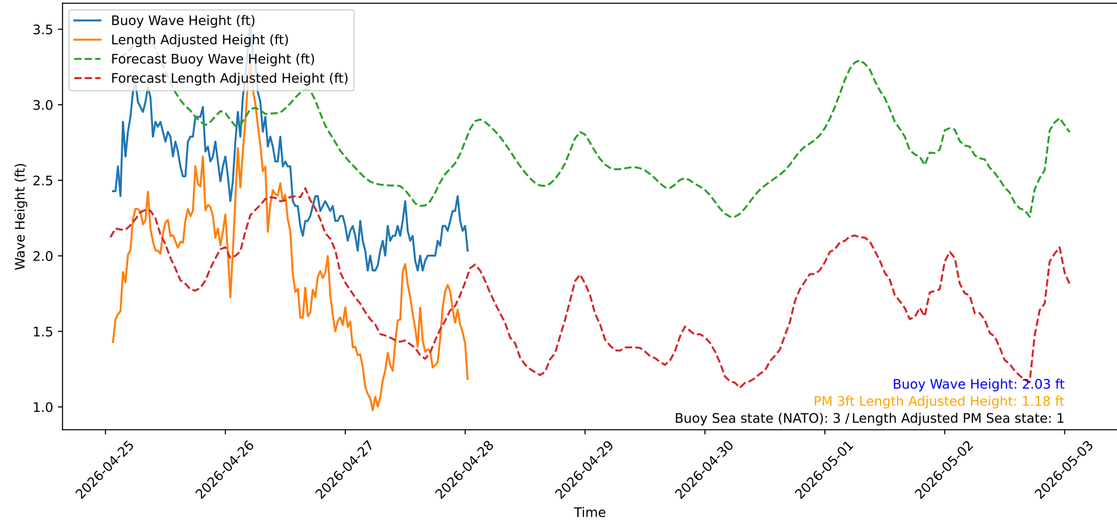
Wave Heights over Time for Red Beach at 2026-04-28 01:20:51
