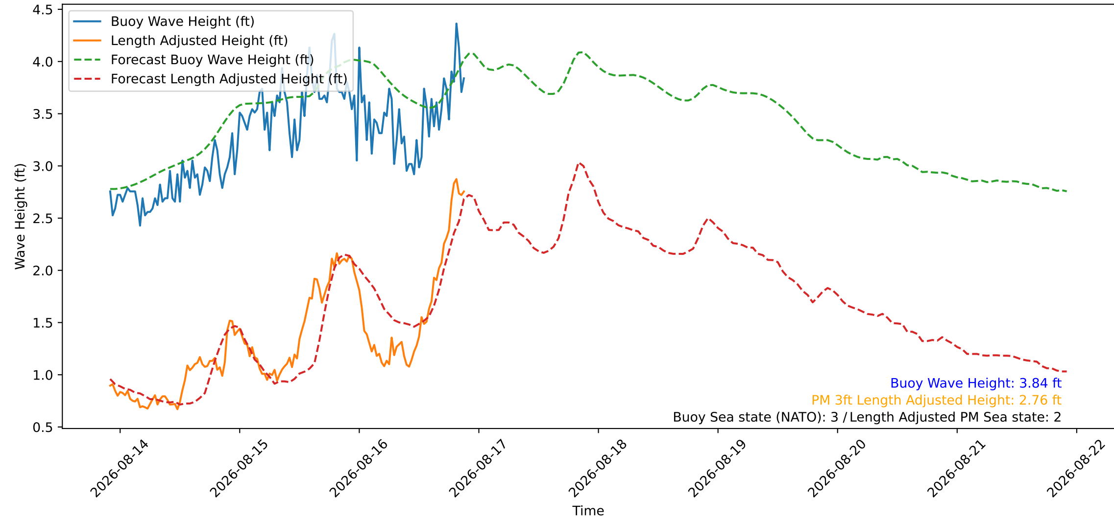
Wave Heights over Time for Green Beach at 2026-08-16 21:41:08
