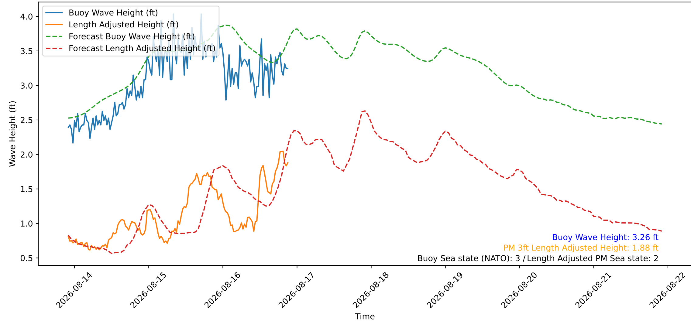
Wave Heights over Time for Red Beach at 2026-08-16 21:40:45
