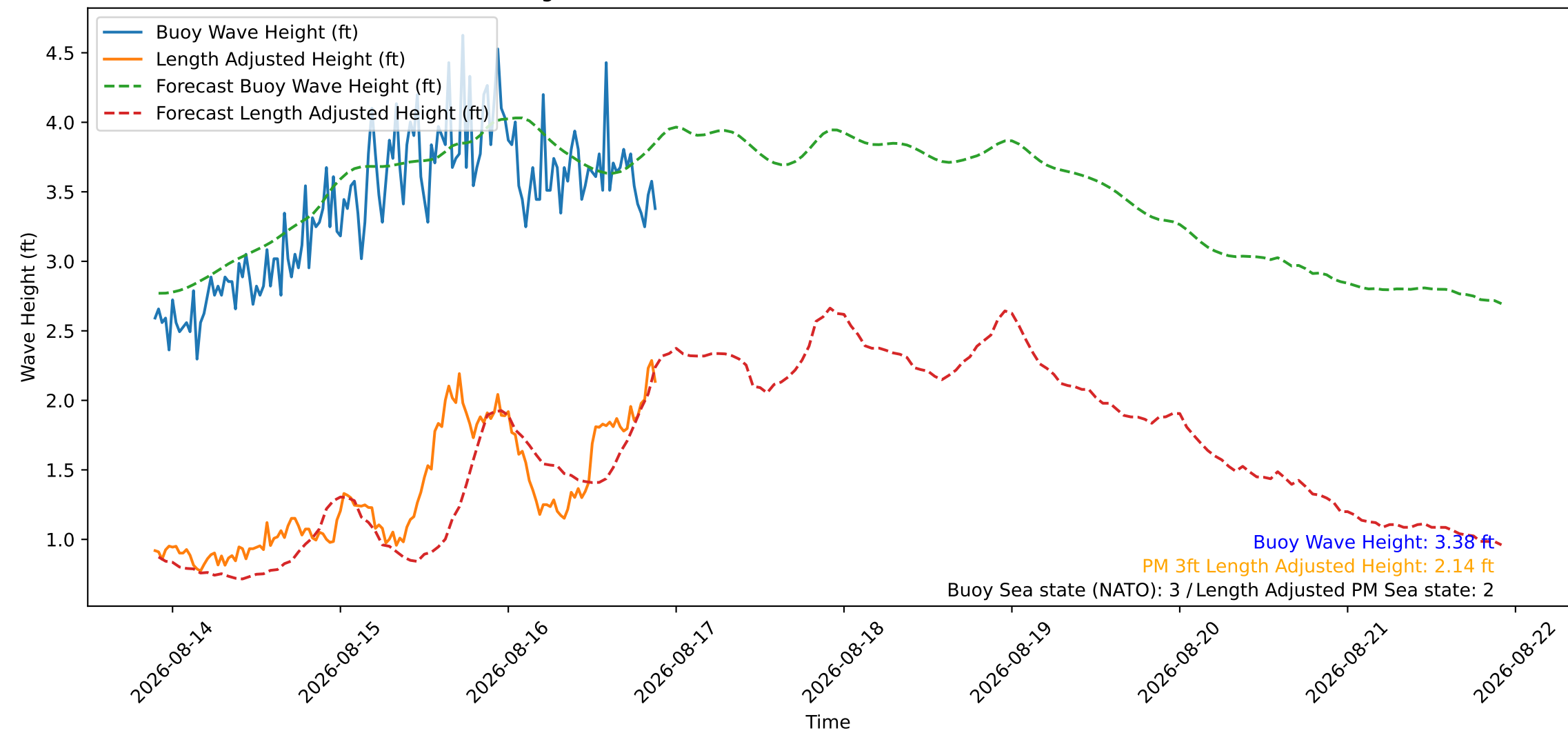
Wave Heights over Time for Oceanside Harbor at 2026-08-16 21:40:26
