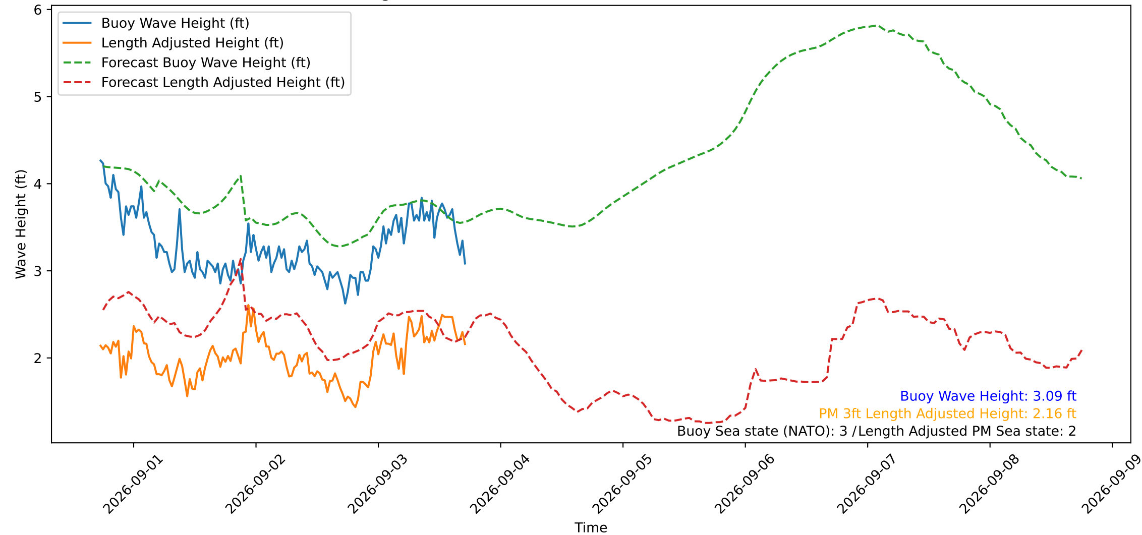
Wave Heights over Time for Oceanside Harbor at 2026-09-03 17:40:29
