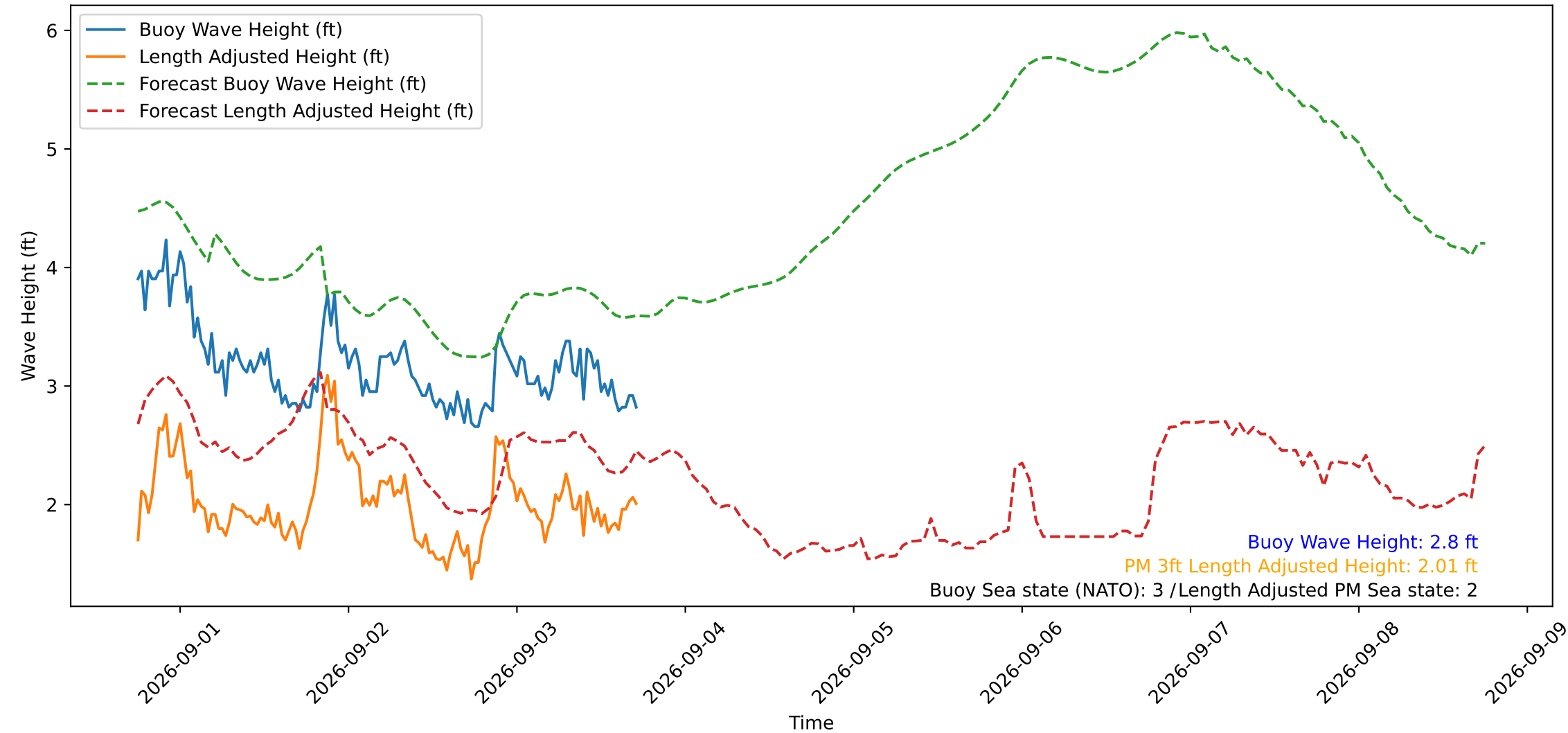
Wave Heights over Time for Green Beach at 2026-09-03 17:41:12
