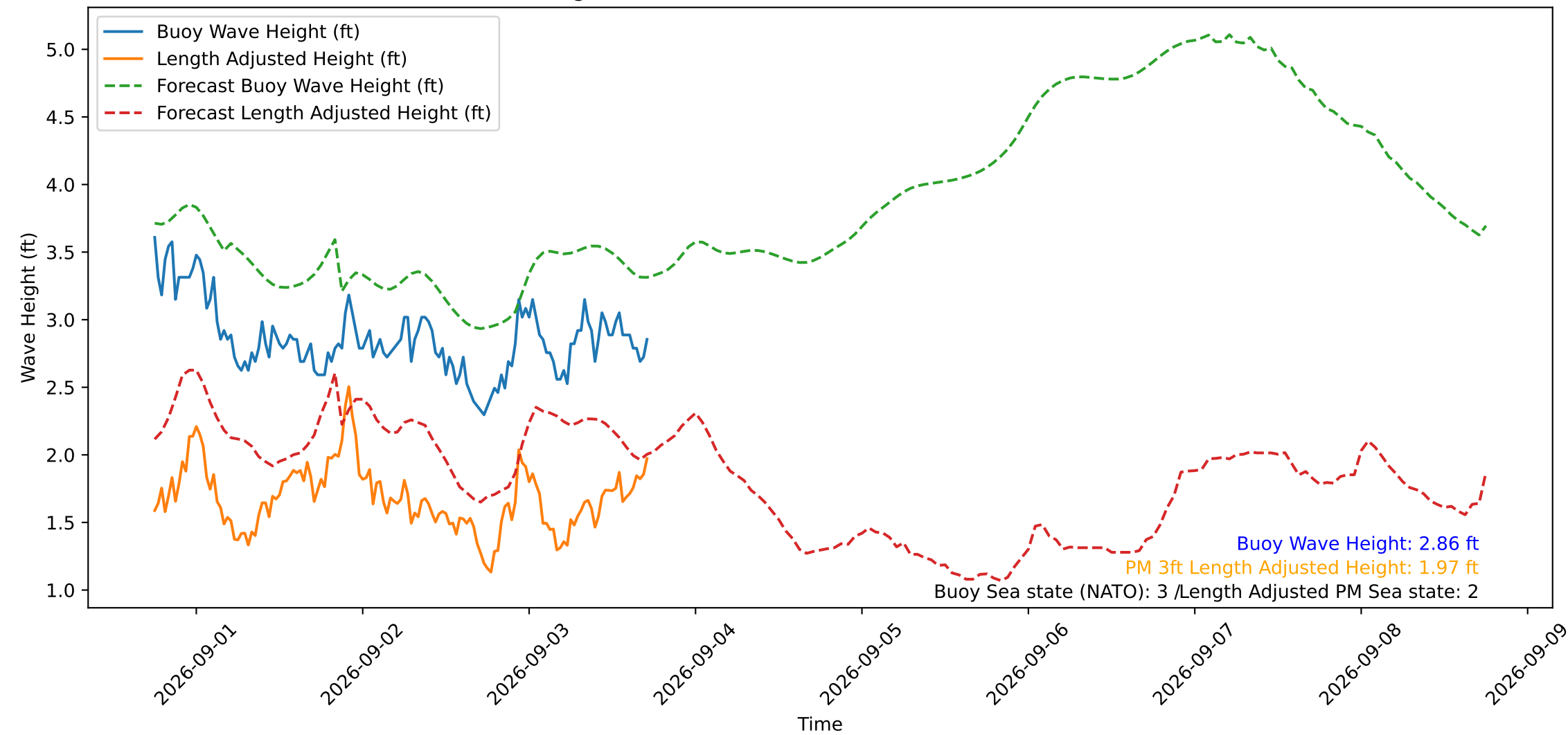
Wave Heights over Time for Red Beach at 2026-09-03 17:40:49
