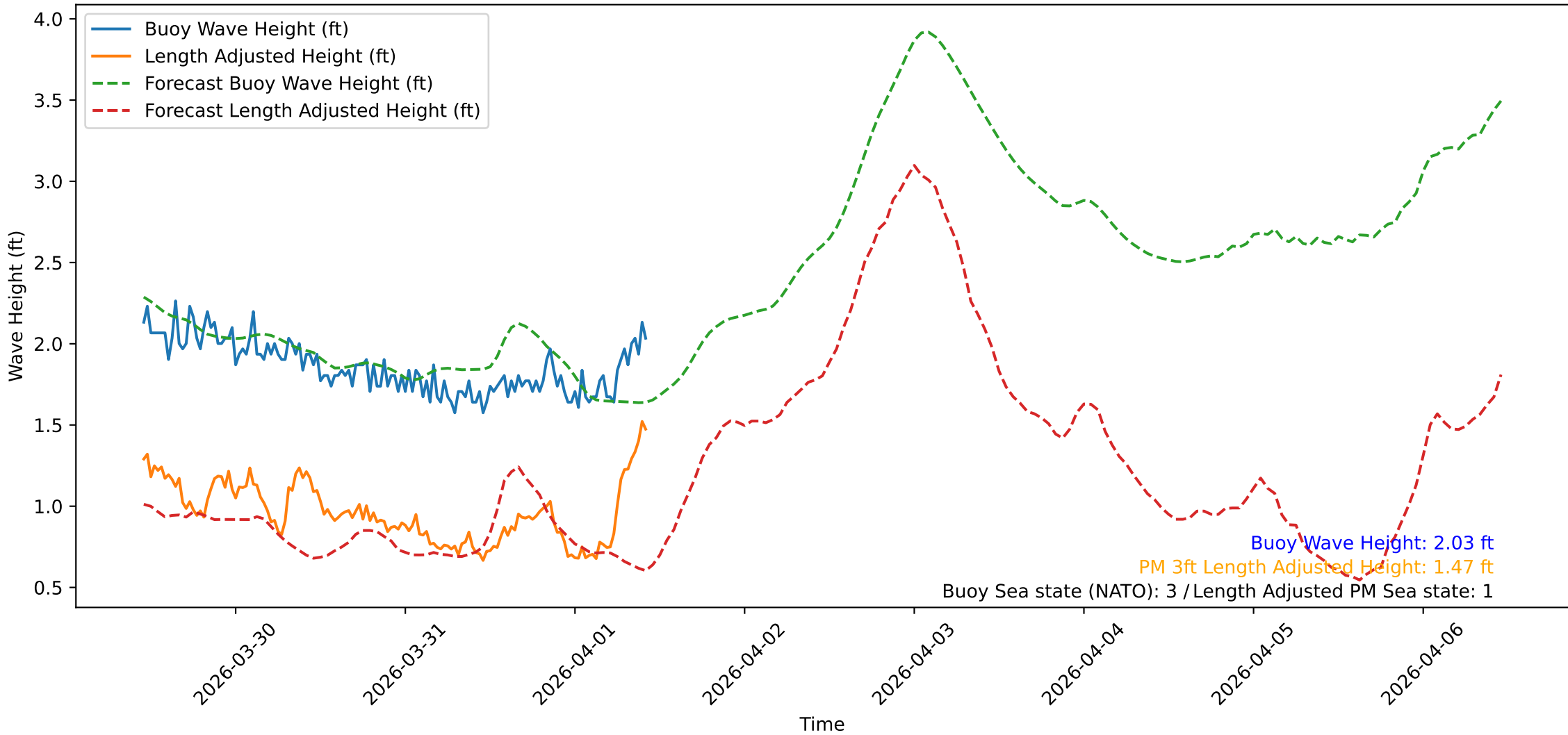
Wave Heights over Time for Oceanside Harbor at 2026-04-01 10:50:31
