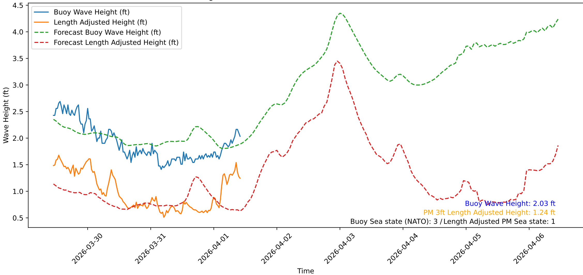
Wave Heights over Time for Green Beach at 2026-04-01 10:51:09
