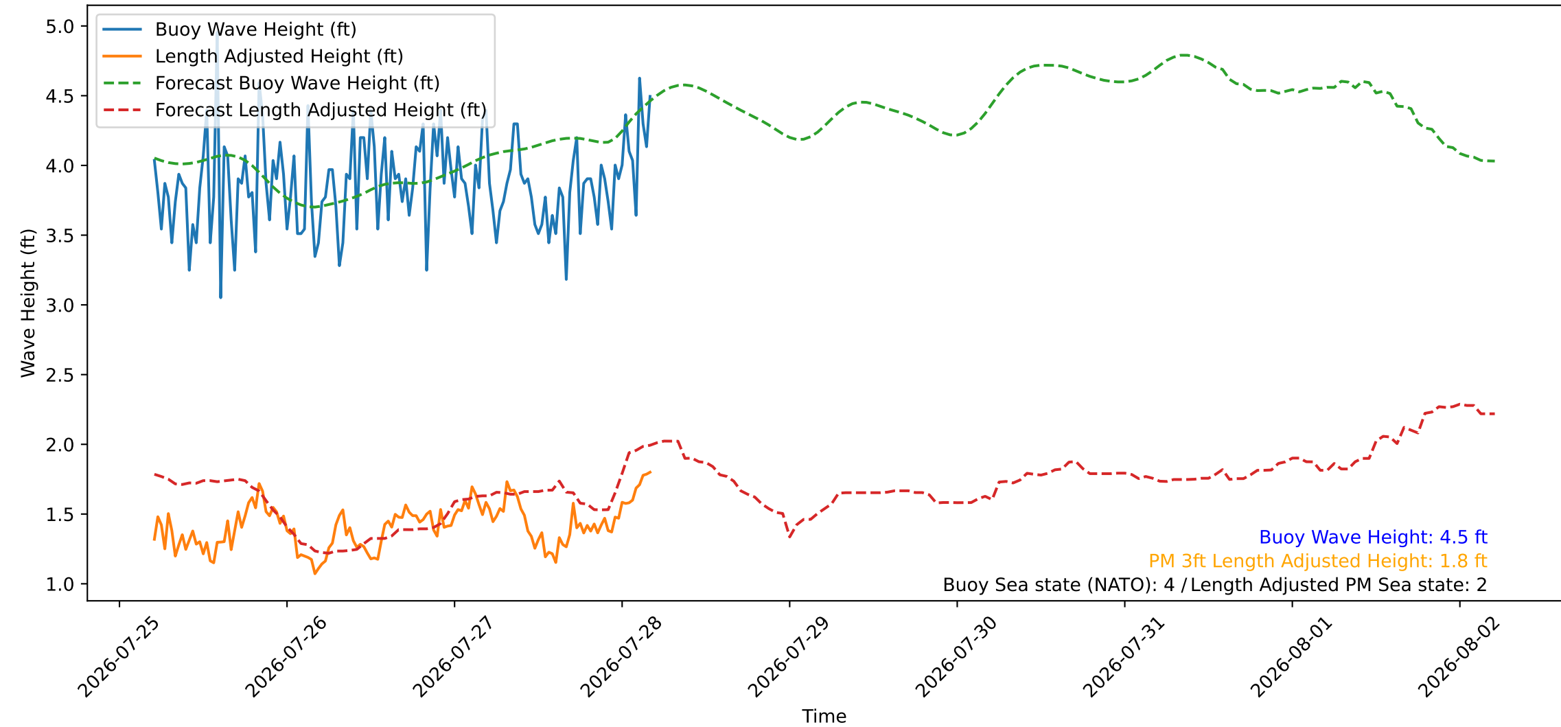
Wave Heights over Time for Oceanside Harbor at 2026-07-28 04:50:26
