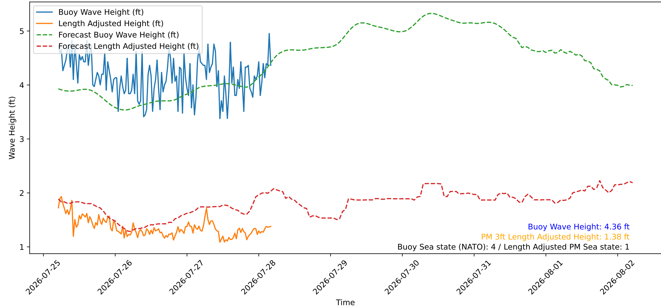
Wave Heights over Time for Green Beach at 2026-07-28 04:51:09
