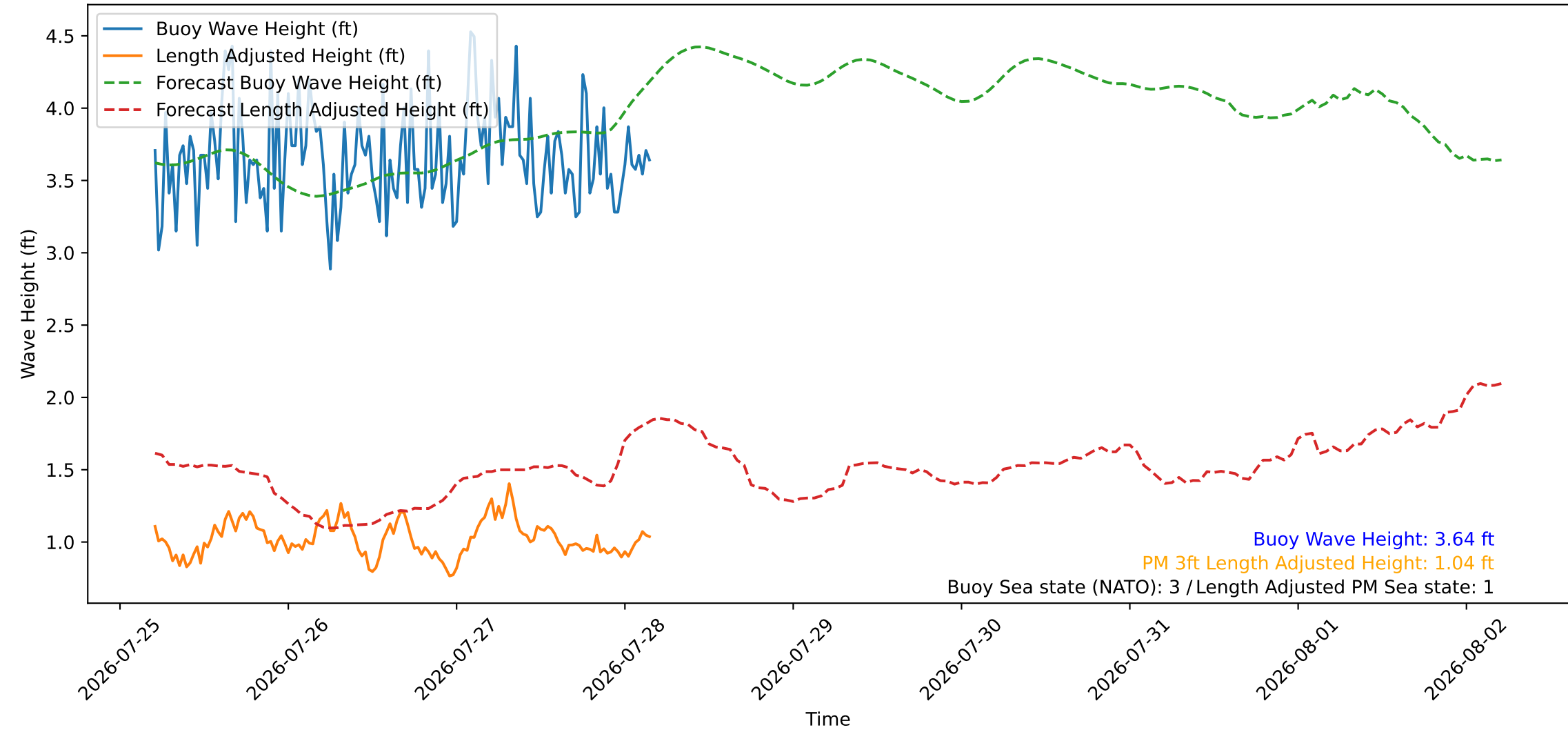
Wave Heights over Time for Red Beach at 2026-07-28 04:50:47
