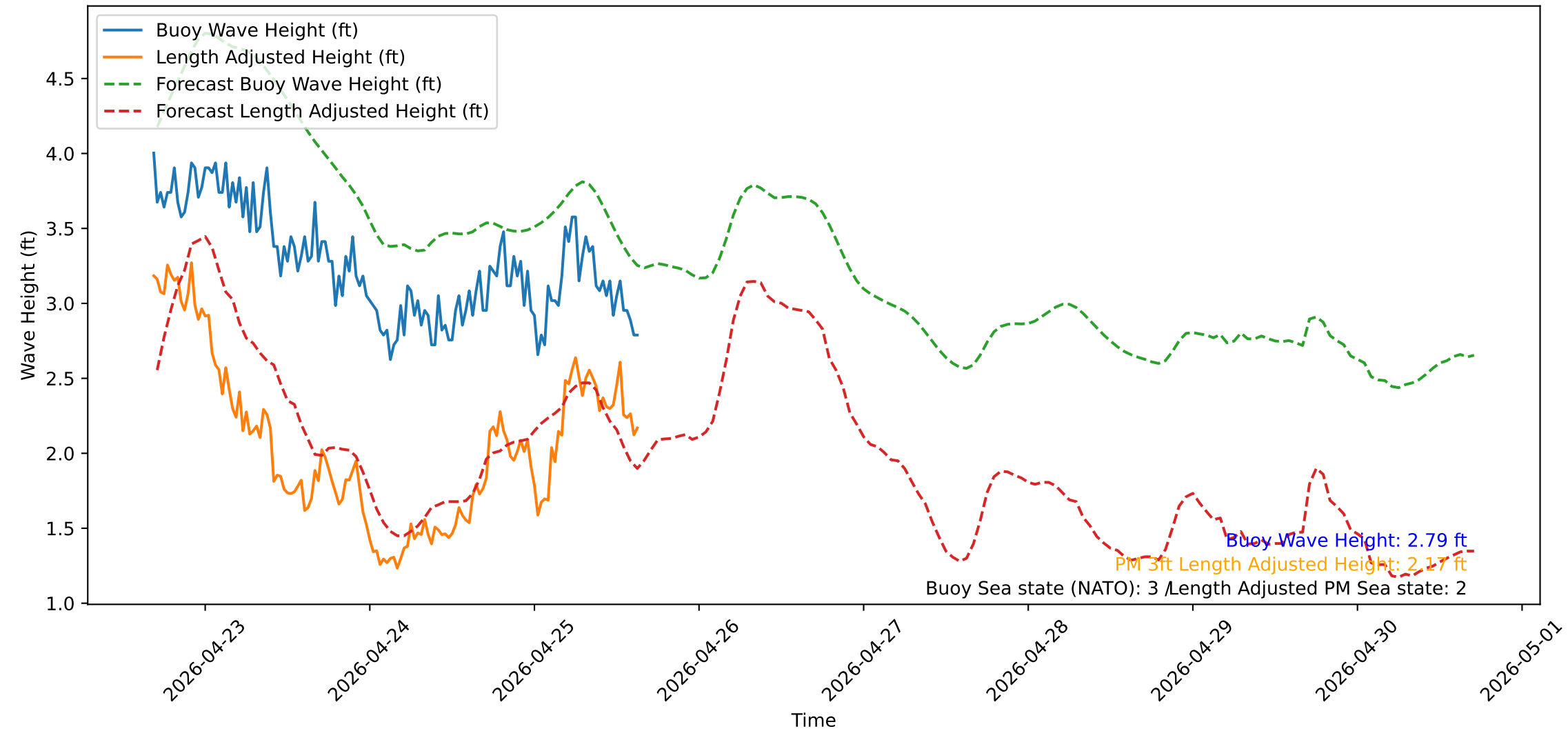
Wave Heights over Time for Green Beach at 2026-04-25 16:41:12
