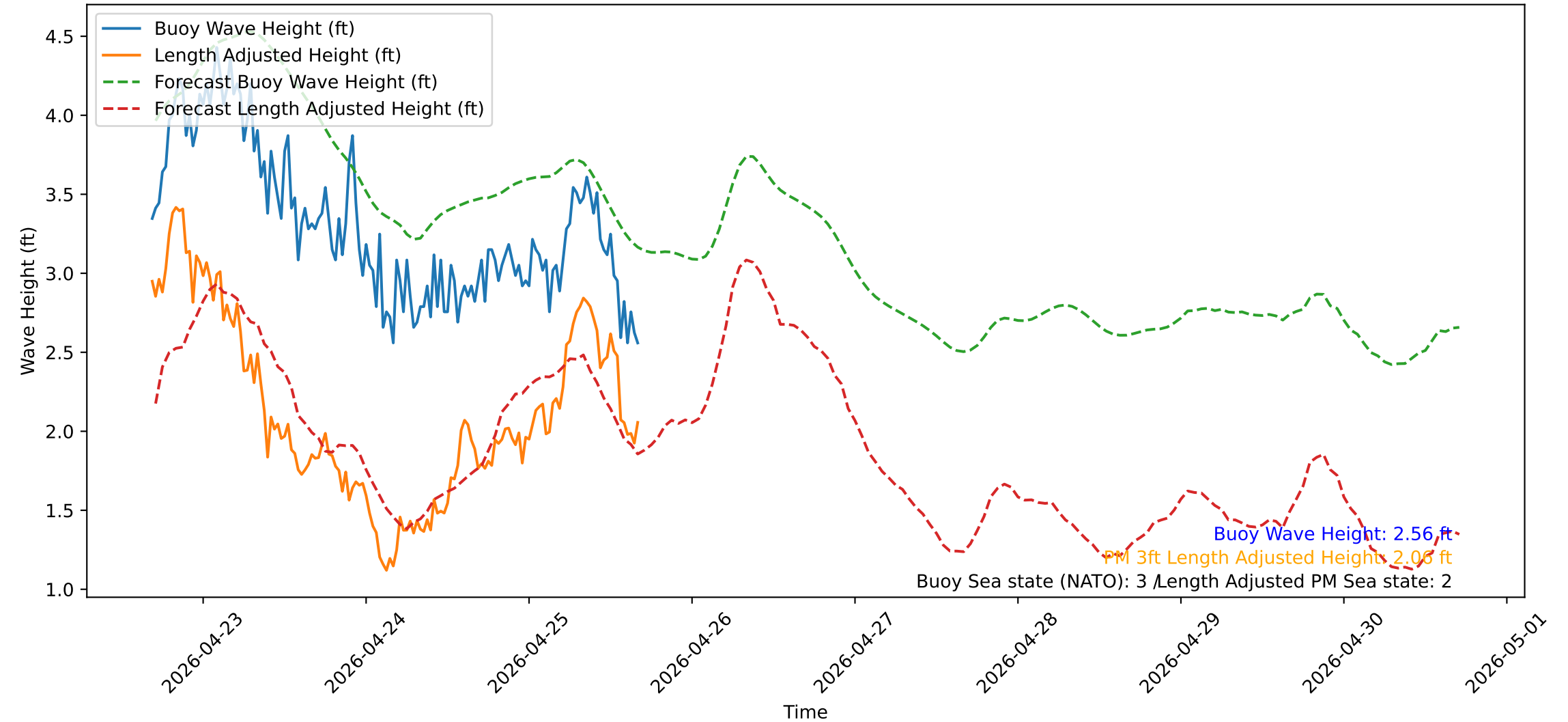
Wave Heights over Time for Oceanside Harbor at 2026-04-25 16:40:31
