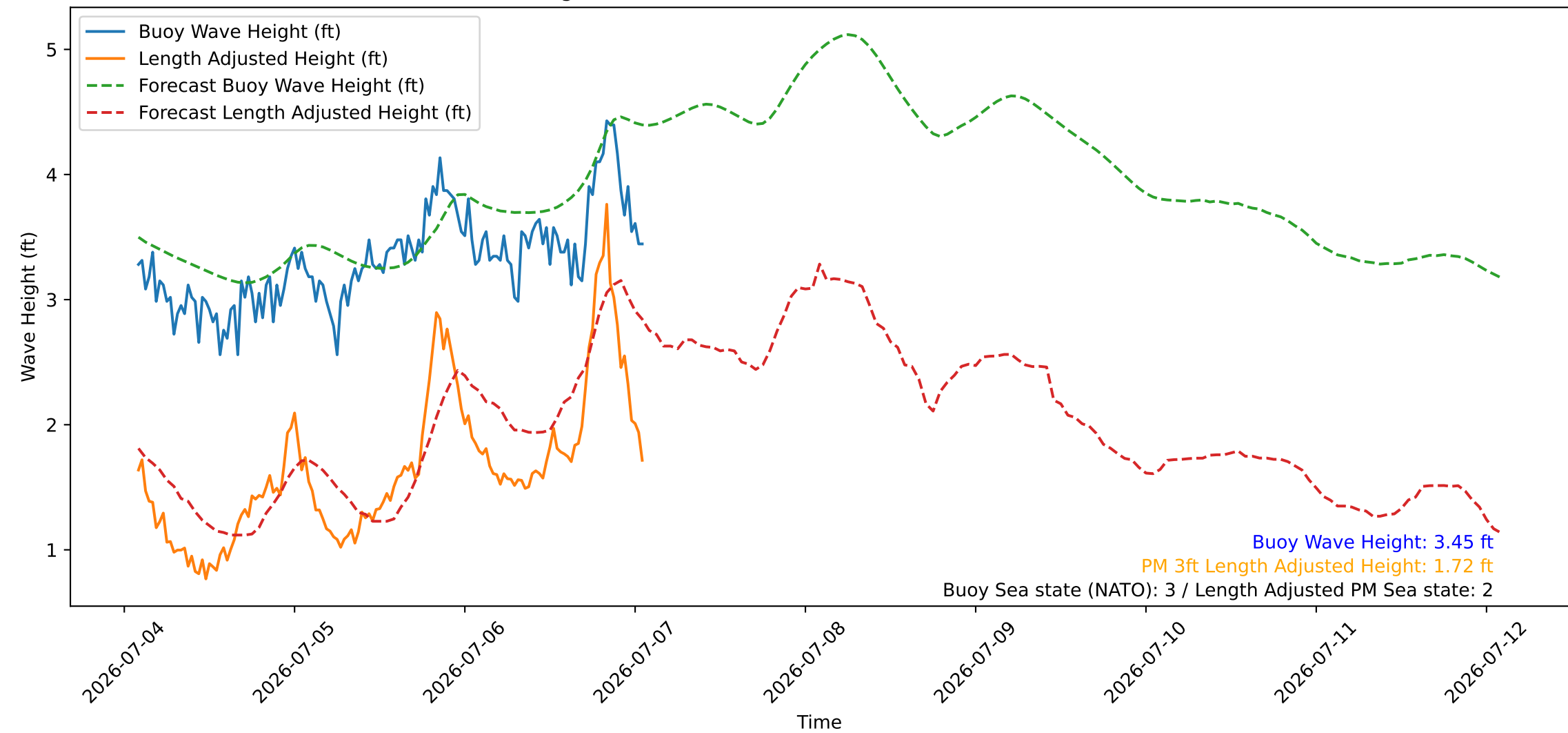
Wave Heights over Time for Green Beach at 2026-07-07 01:51:10
