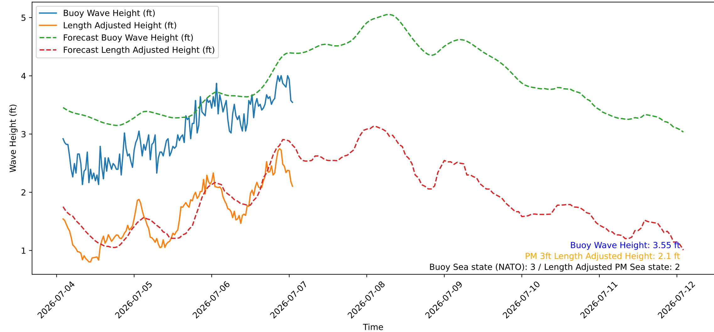
Wave Heights over Time for Oceanside Harbor at 2026-07-07 01:50:27
