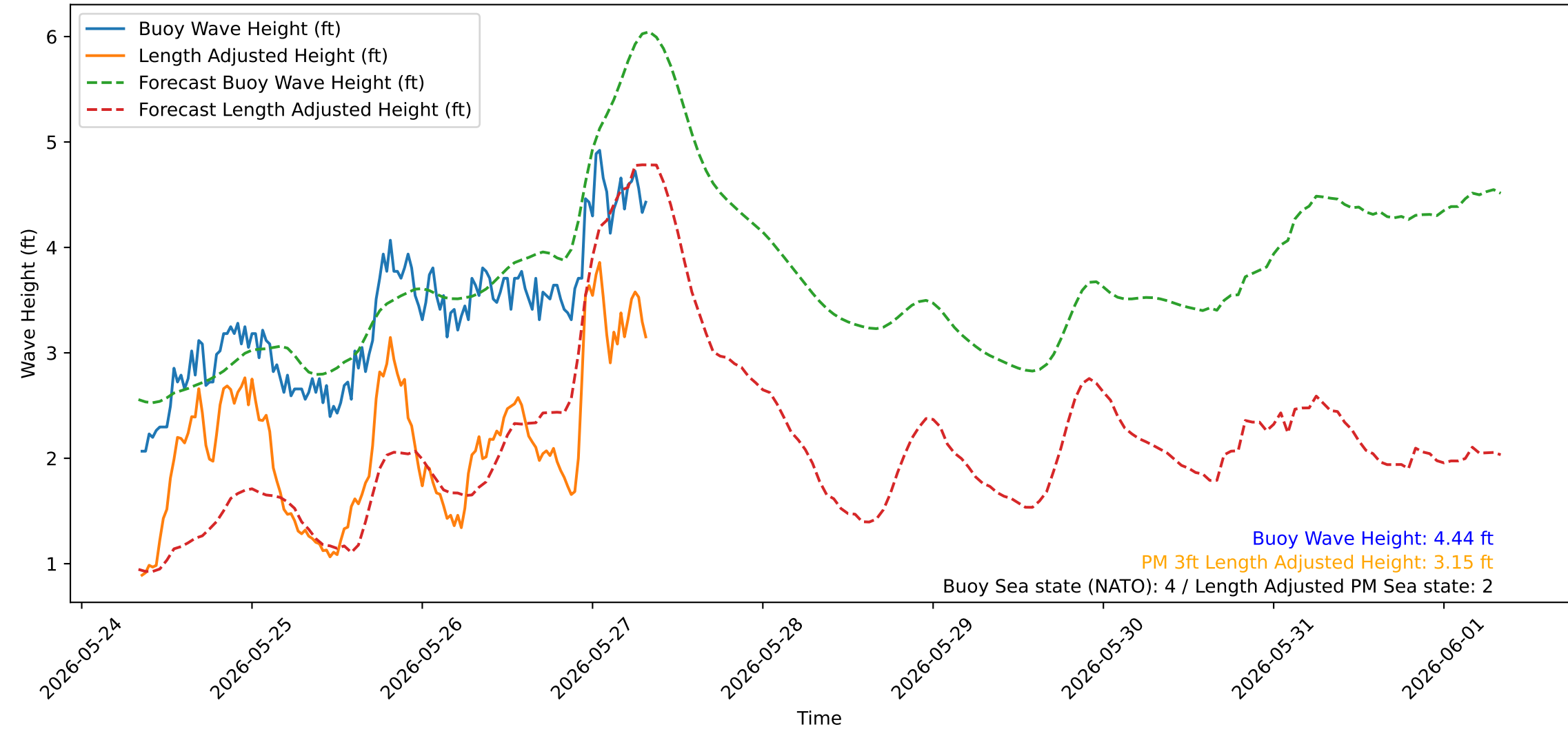
Wave Heights over Time for Green Beach at 2026-05-27 08:21:08
