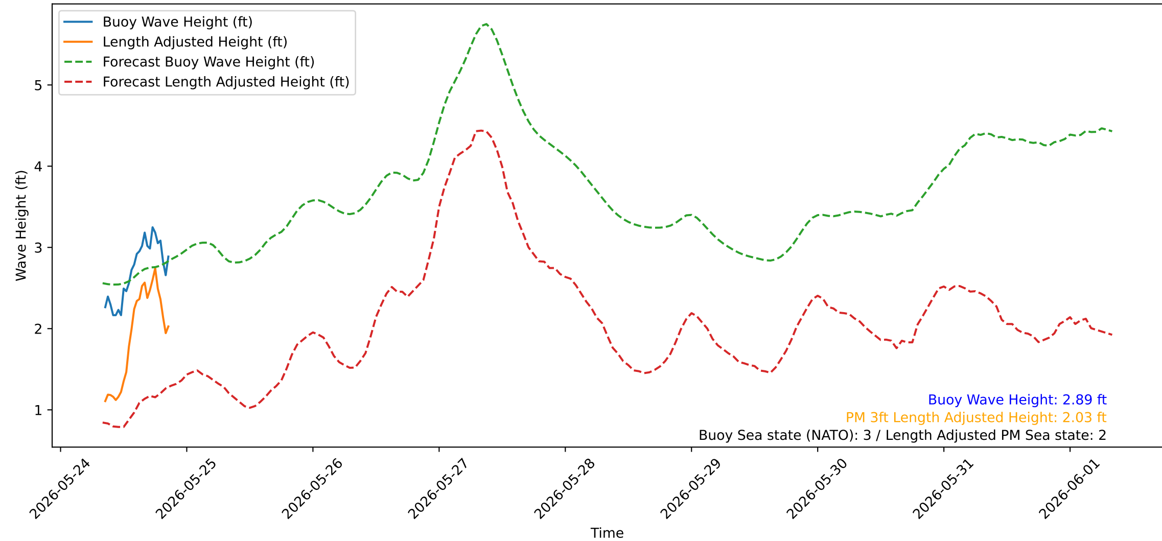
Wave Heights over Time for Oceanside Harbor at 2026-05-27 08:20:25
