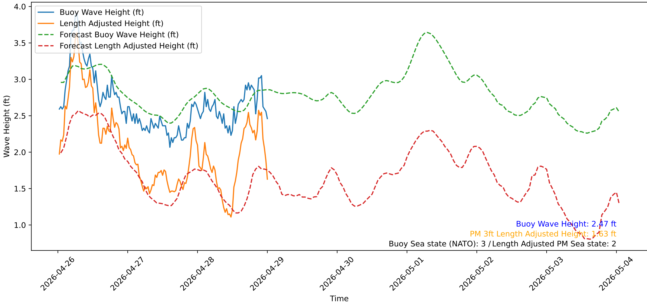
Wave Heights over Time for Oceanside Harbor at 2026-04-29 00:40:31
