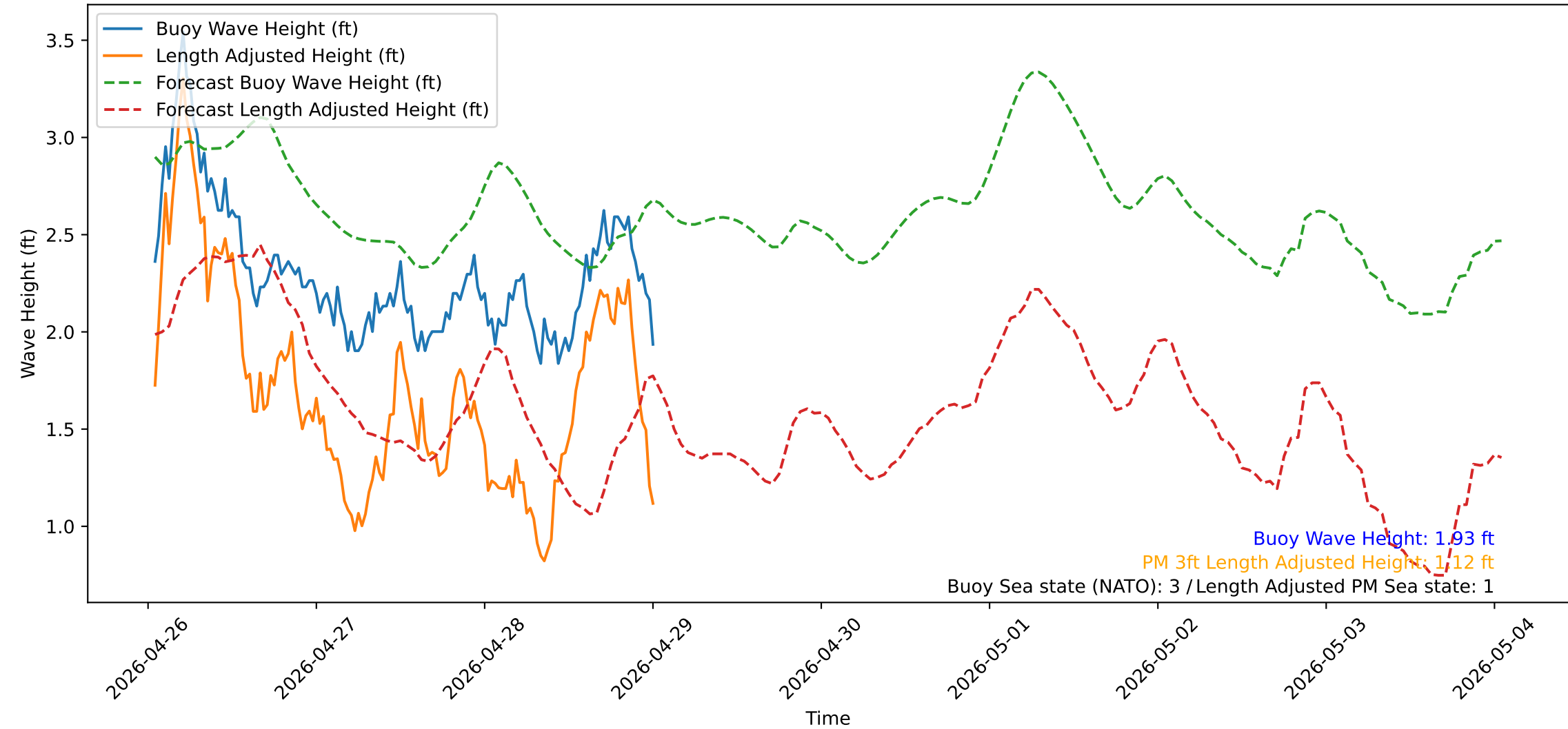
Wave Heights over Time for Red Beach at 2026-04-29 00:40:50
