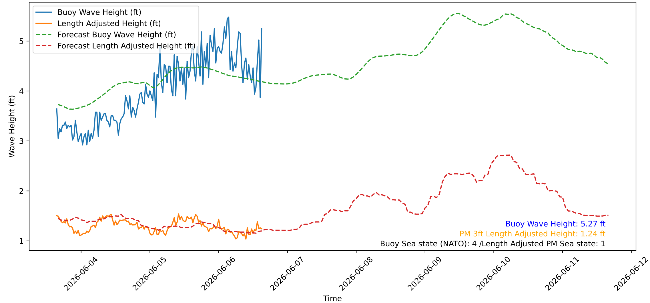
Wave Heights over Time for Oceanside Harbor at 2026-06-06 15:40:26
