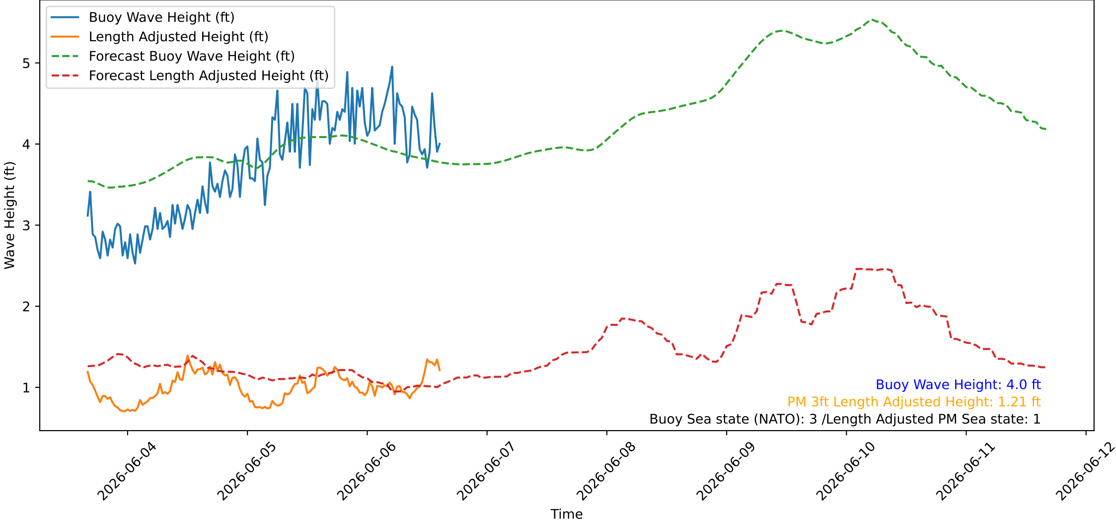
Wave Heights over Time for Red Beach at 2026-06-06 15:40:45
