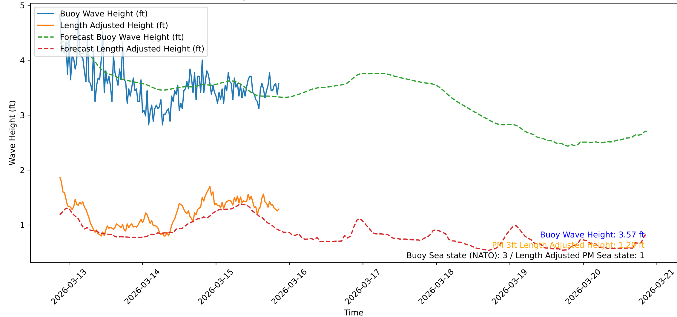
Wave Heights over Time for Green Beach at 2026-03-15 21:12:11
