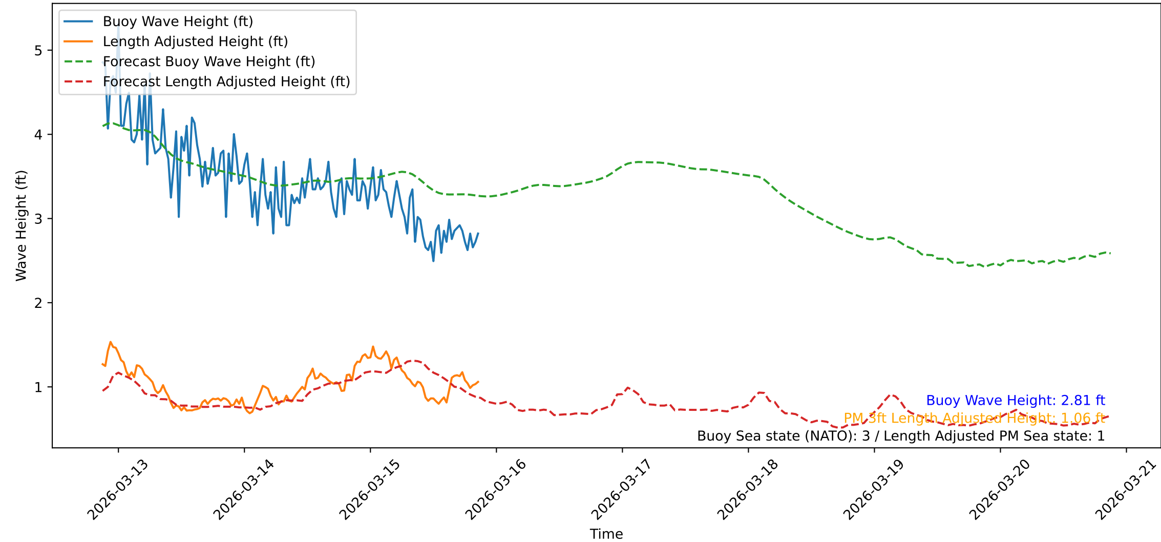
Wave Heights over Time for Oceanside Harbor at 2026-03-15 21:10:43
