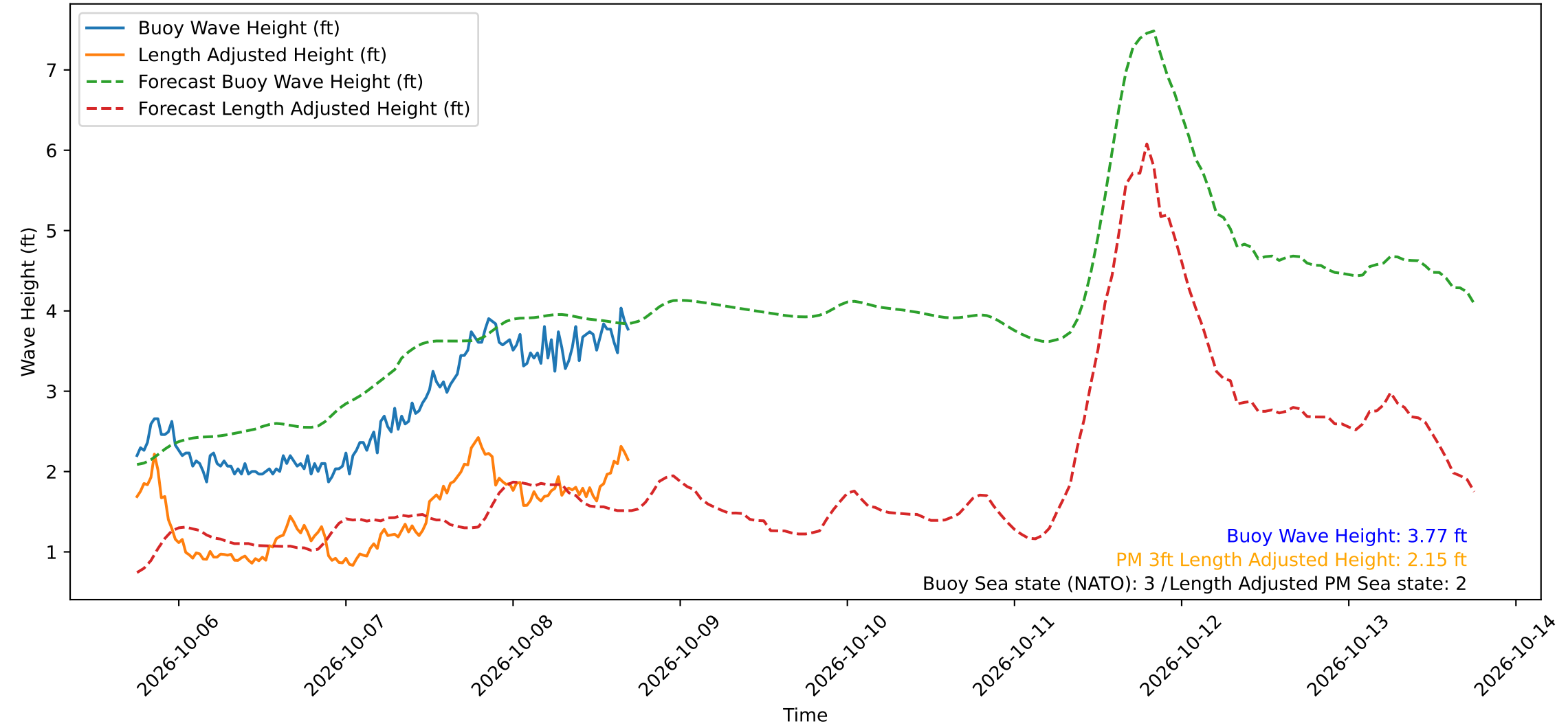
Wave Heights over Time for Red Beach at 2026-10-08 17:30:49
