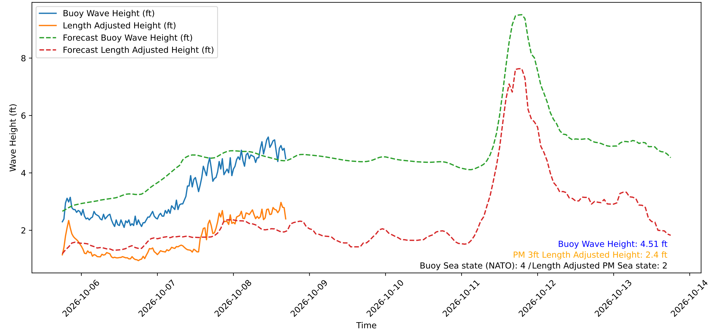
Wave Heights over Time for Green Beach at 2026-10-08 17:31:11
