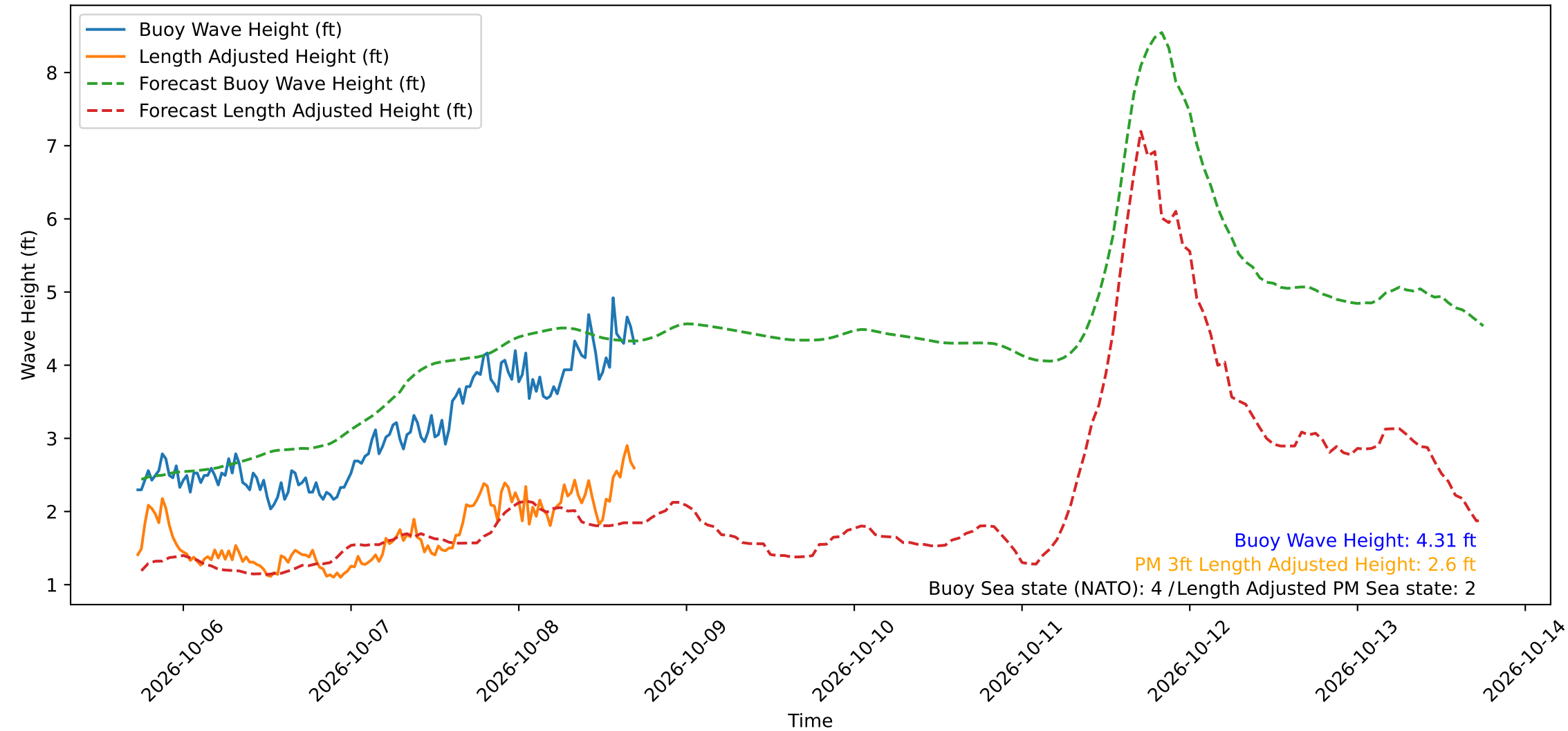
Wave Heights over Time for Oceanside Harbor at 2026-10-08 17:30:29
