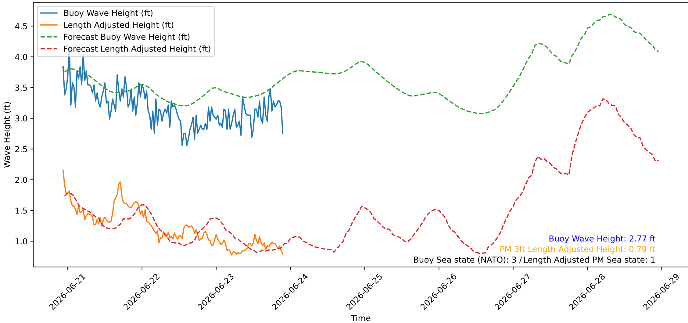
Wave Heights over Time for Oceanside Harbor at 2026-06-23 22:40:26
