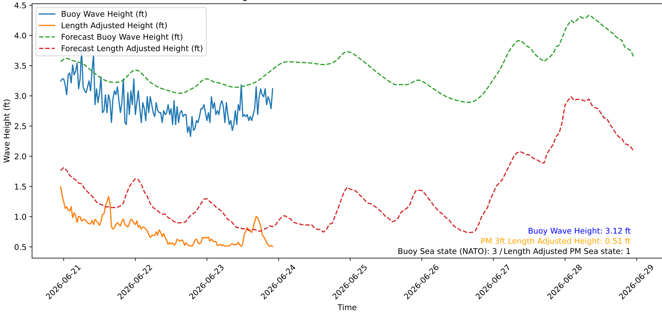
Wave Heights over Time for Red Beach at 2026-06-23 22:40:46
