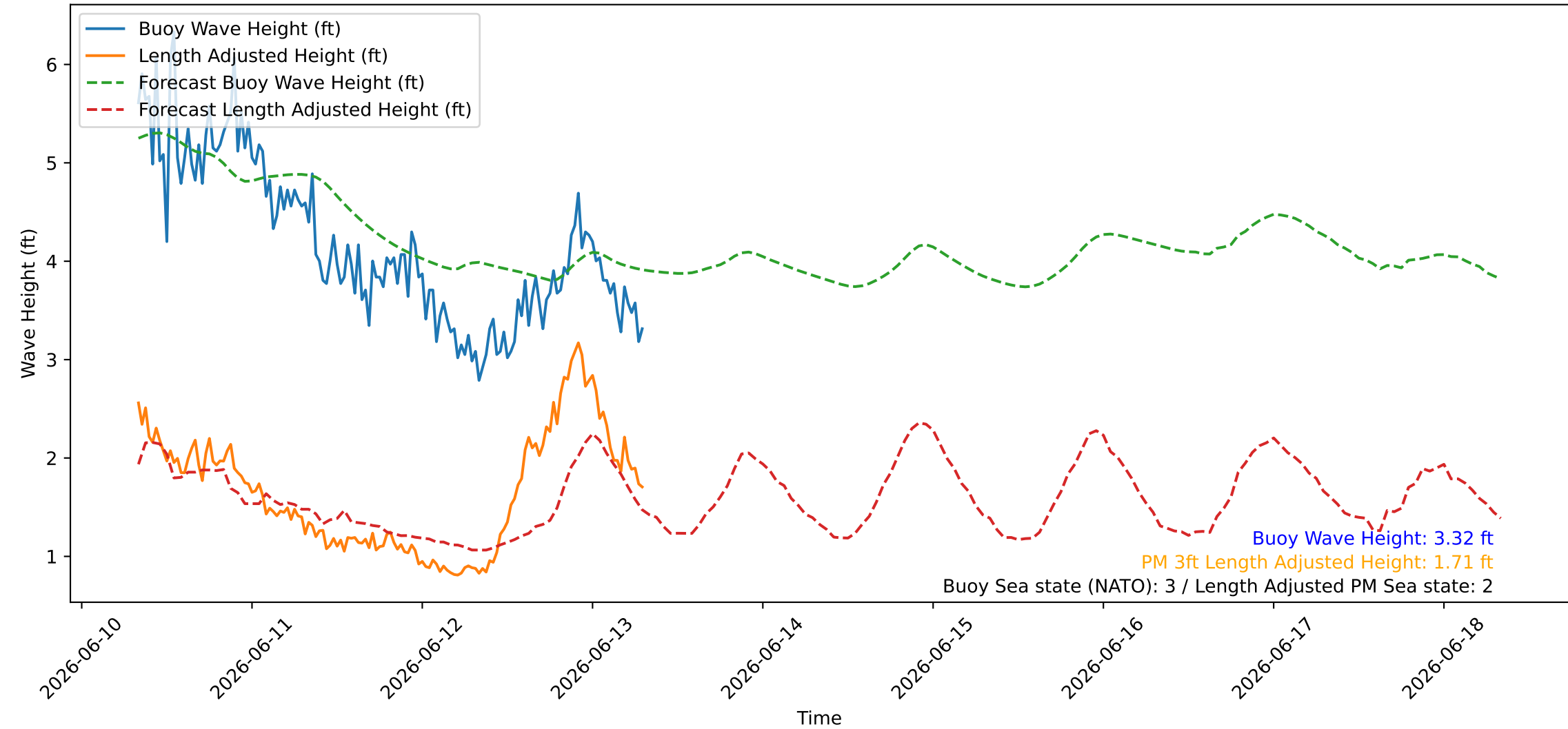
Wave Heights over Time for Oceanside Harbor at 2026-06-13 07:50:27
