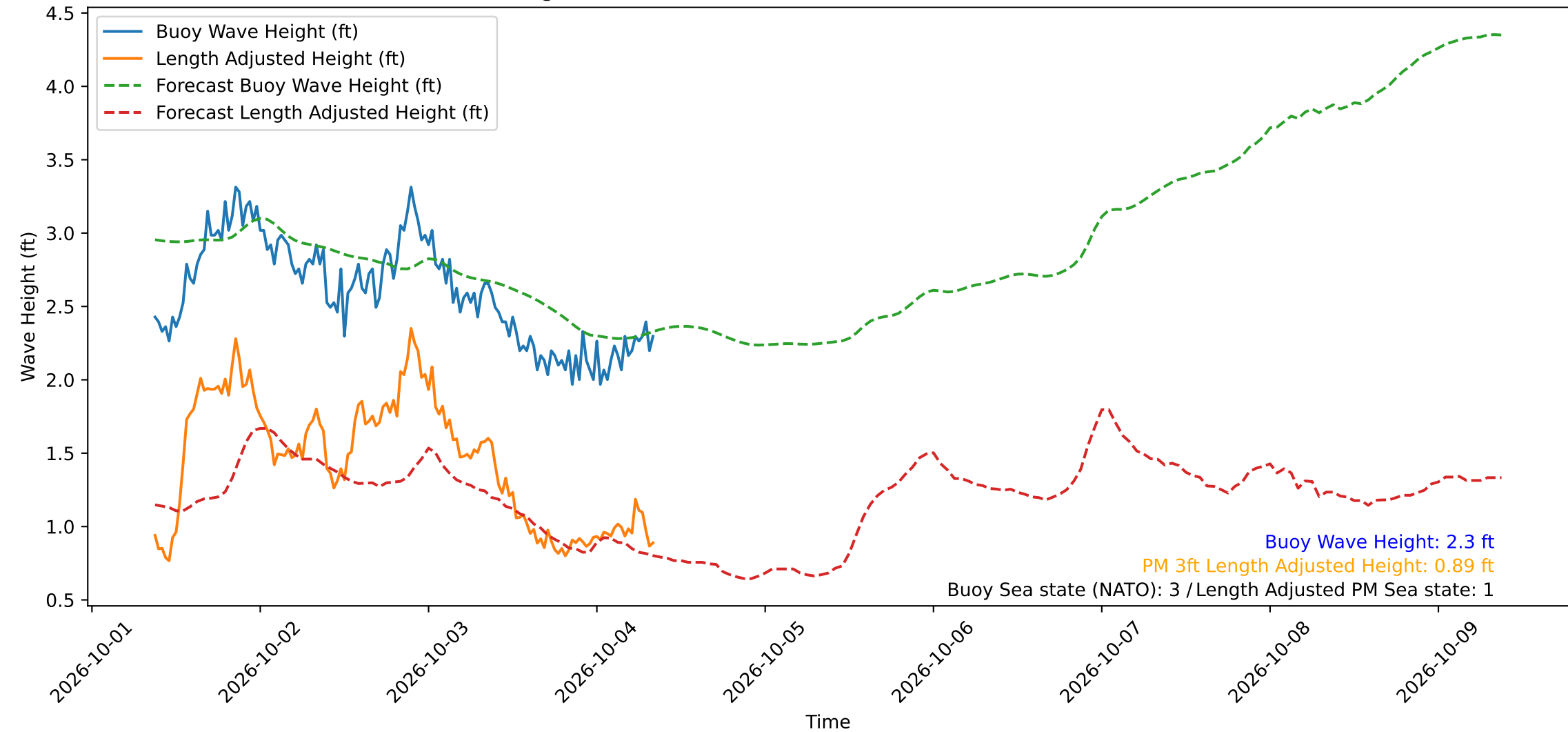
Wave Heights over Time for Oceanside Harbor at 2026-10-04 08:50:30
