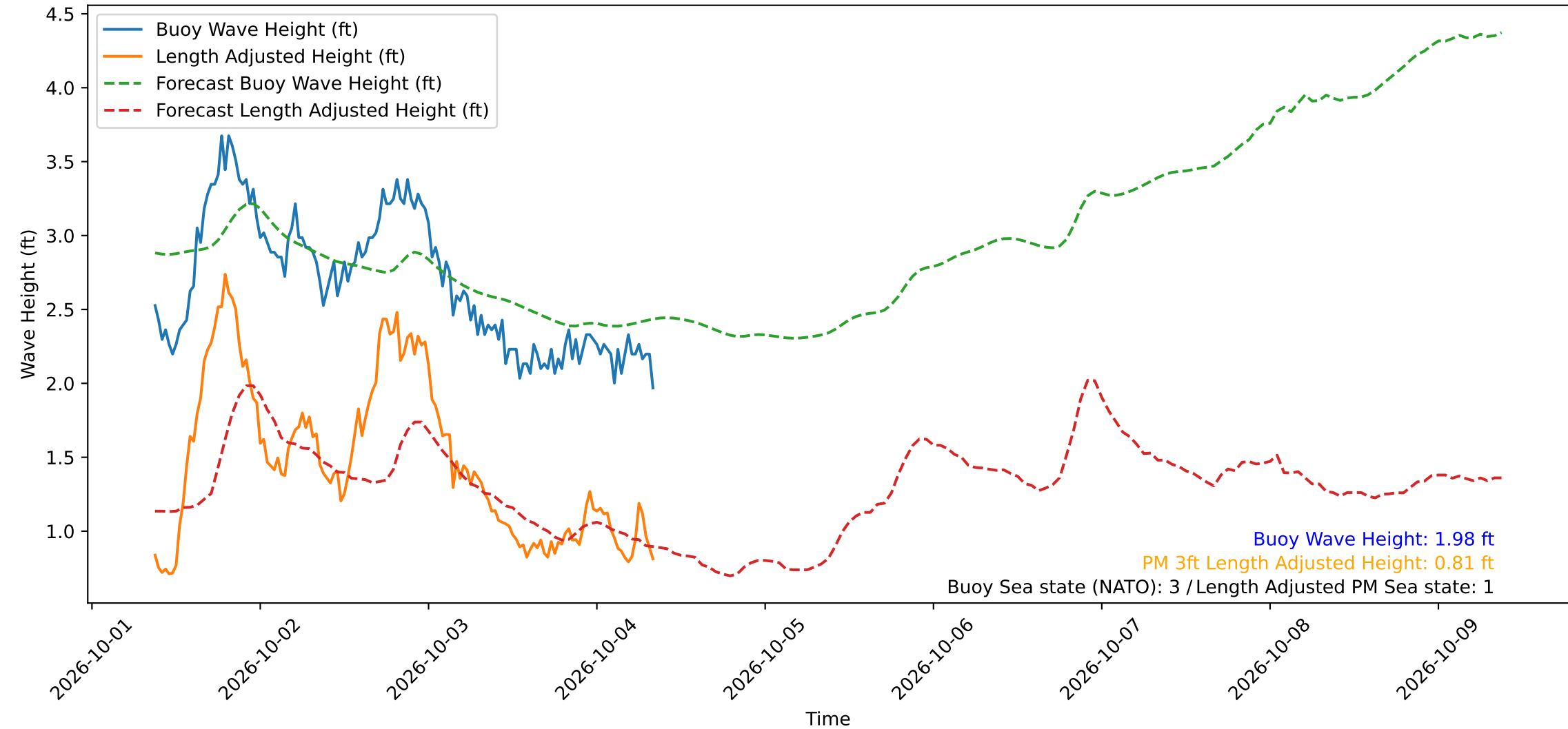
Wave Heights over Time for Green Beach at 2026-10-04 08:51:15
