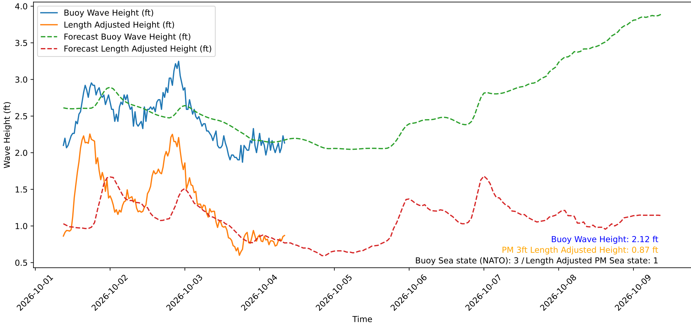
Wave Heights over Time for Red Beach at 2026-10-04 08:50:50
