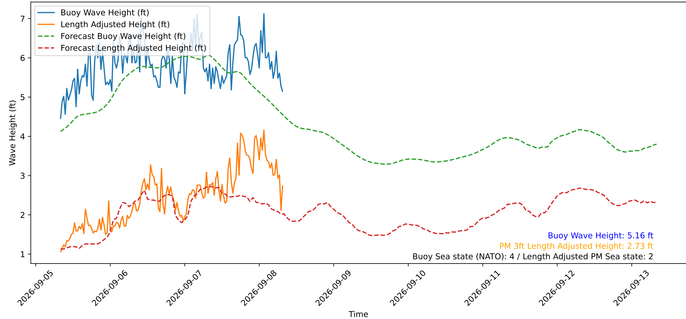
Wave Heights over Time for Oceanside Harbor at 2026-09-08 08:00:30
