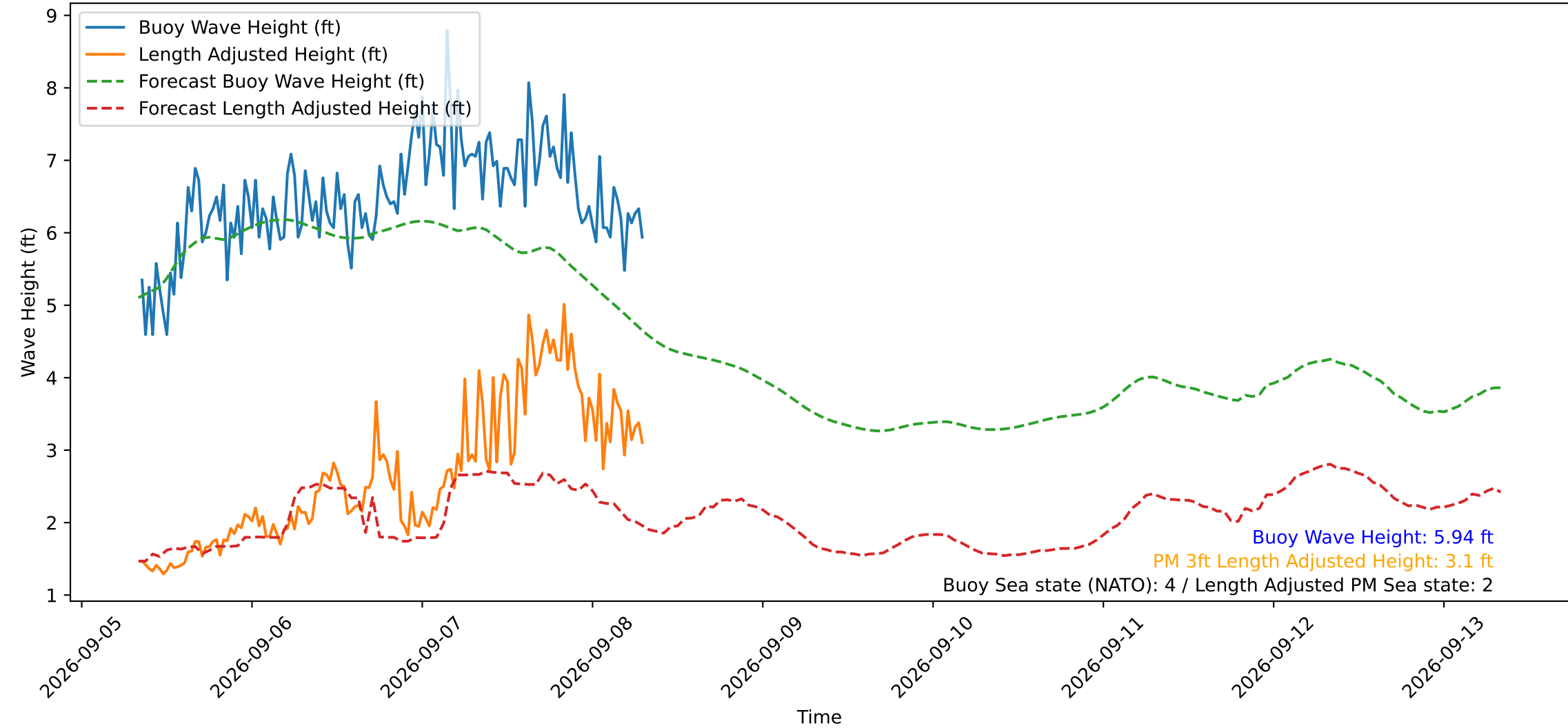
Wave Heights over Time for Green Beach at 2026-09-08 08:01:12
