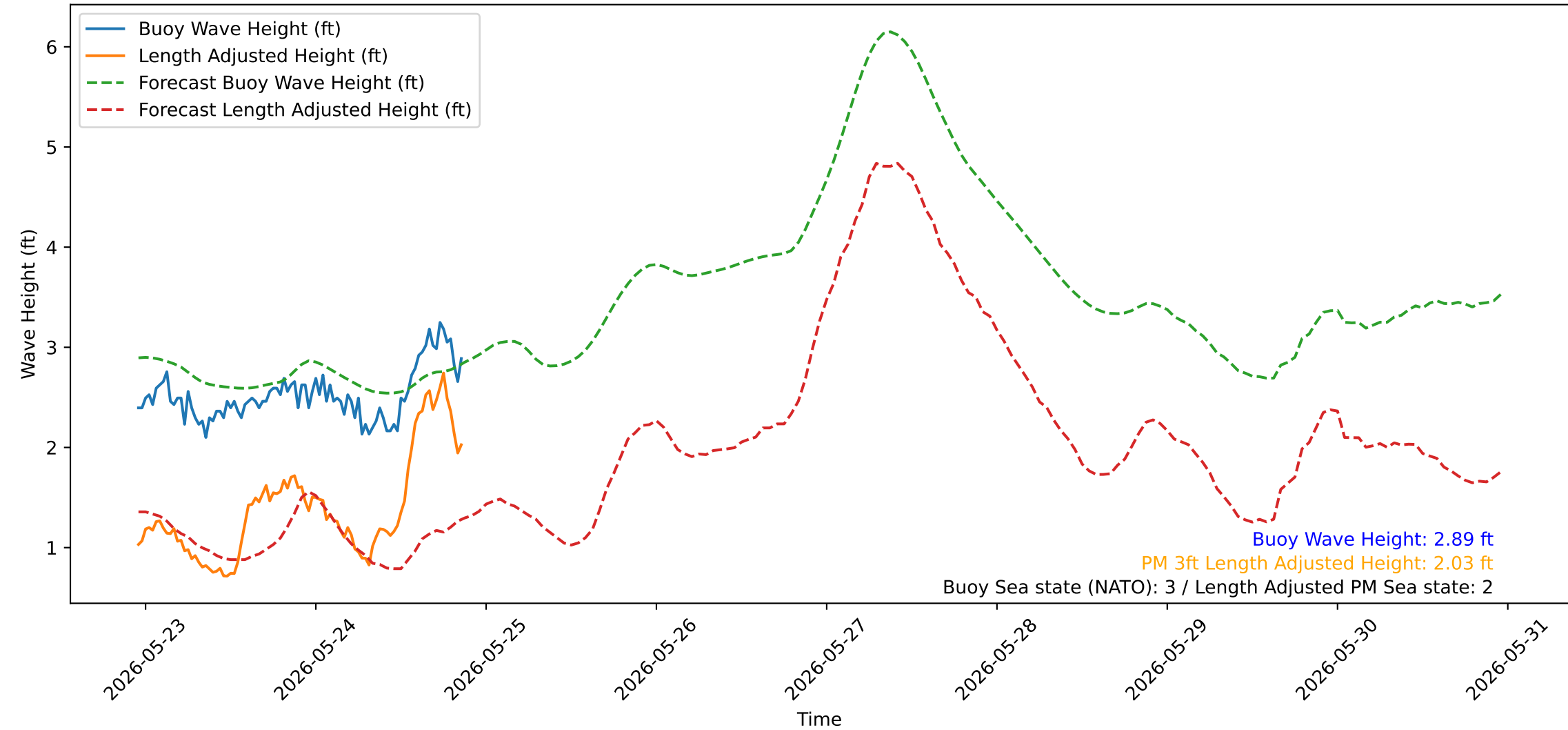
Wave Heights over Time for Oceanside Harbor at 2026-05-25 22:50:28
