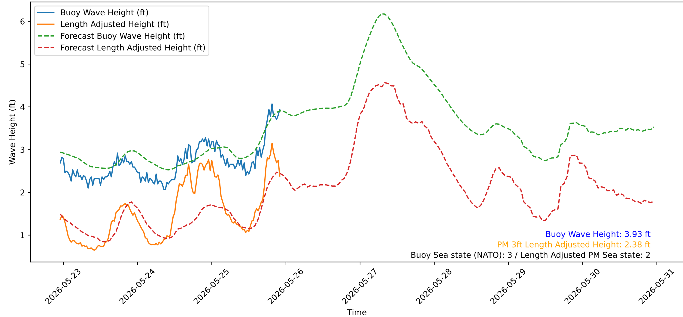
Wave Heights over Time for Green Beach at 2026-05-25 22:51:12
