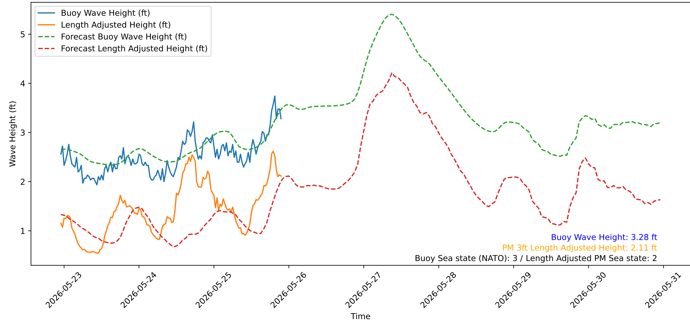
Wave Heights over Time for Red Beach at 2026-05-25 22:50:49
