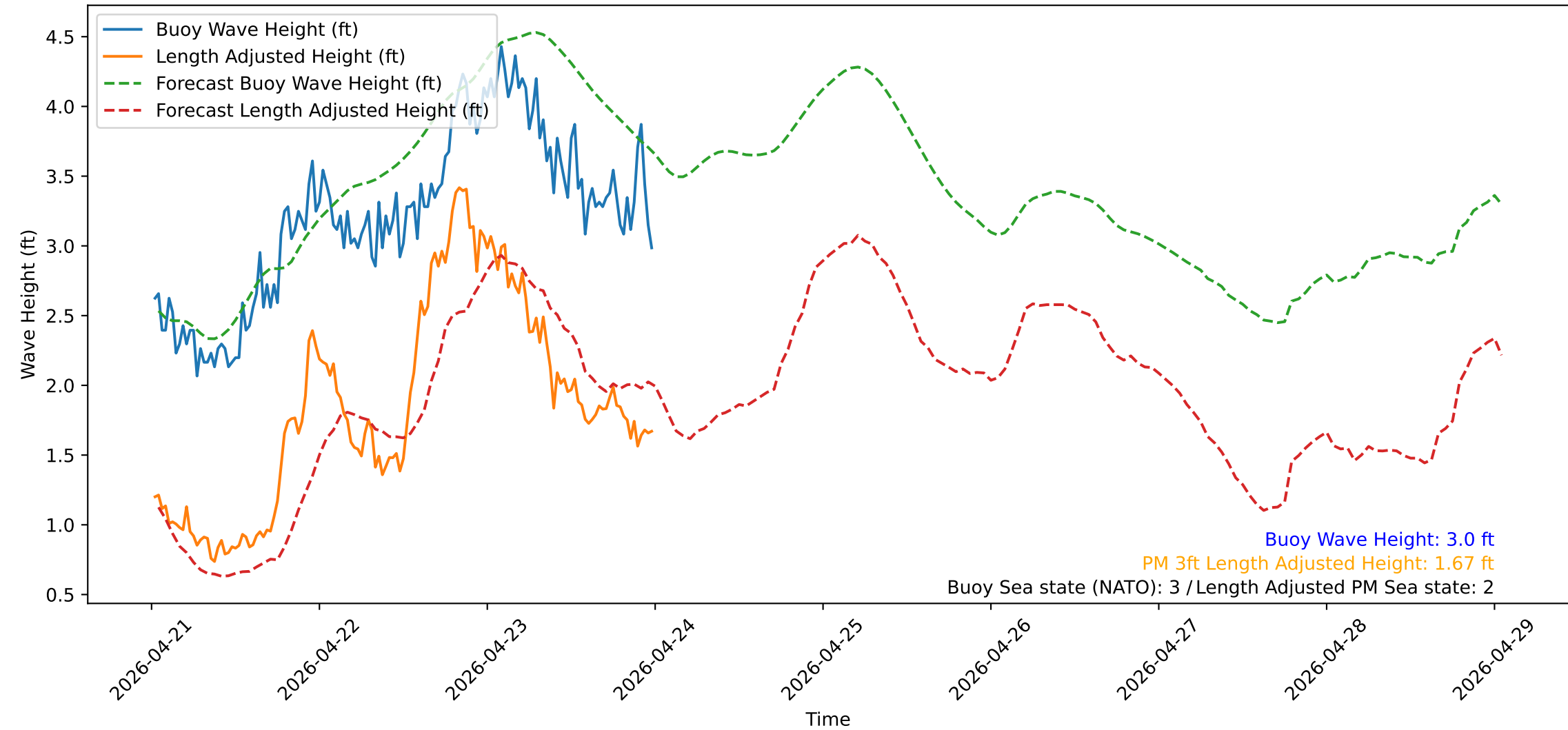
Wave Heights over Time for Oceanside Harbor at 2026-04-24 00:30:31
