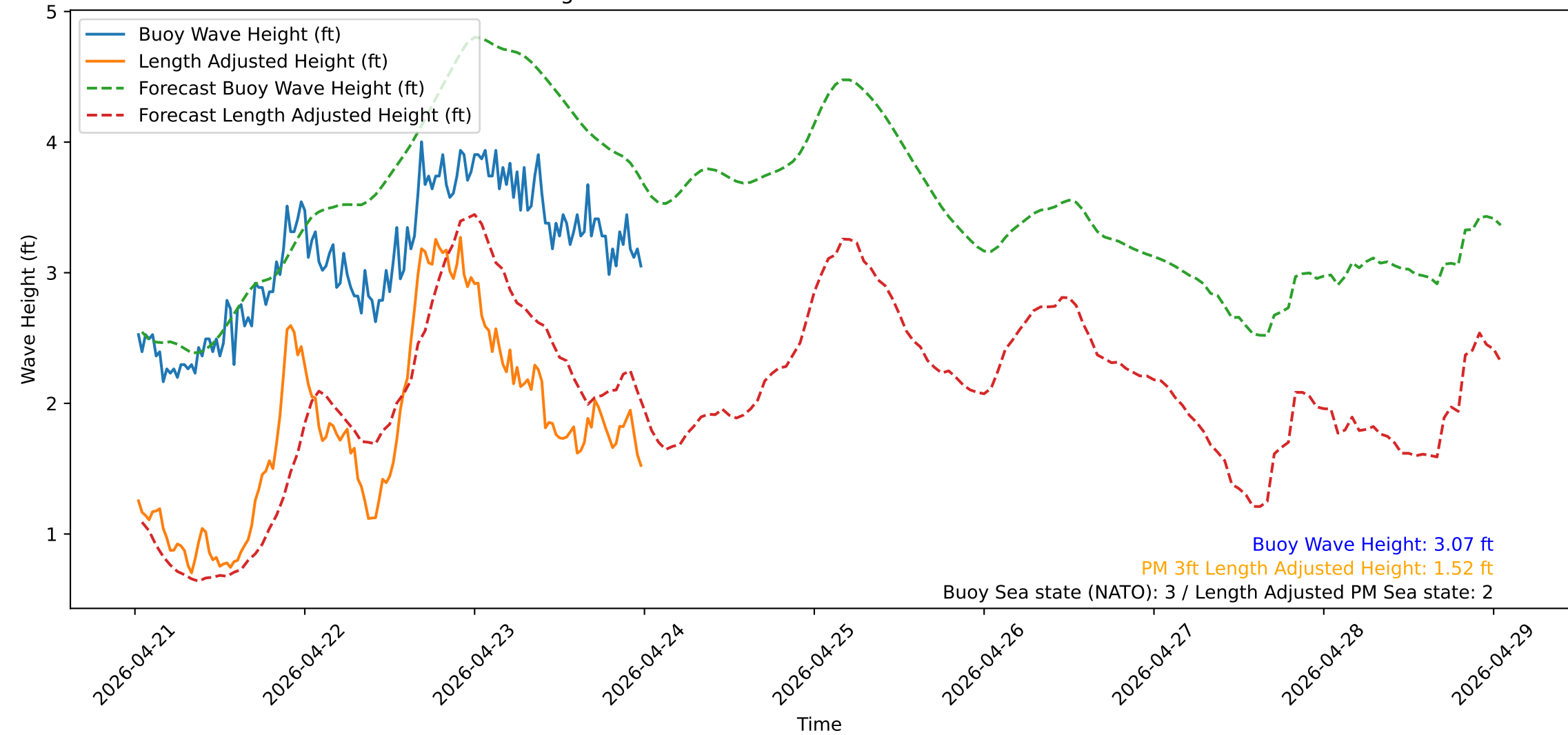
Wave Heights over Time for Green Beach at 2026-04-24 00:31:12
