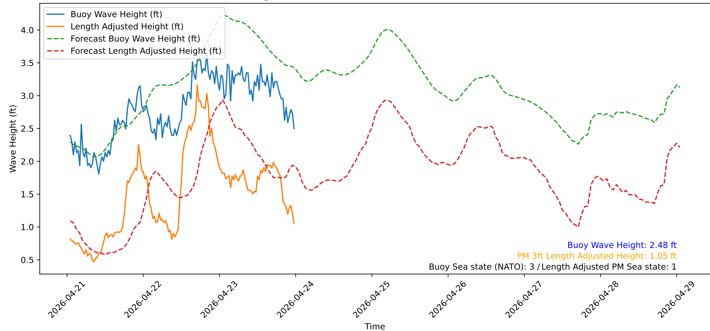
Wave Heights over Time for Red Beach at 2026-04-24 00:30:50
