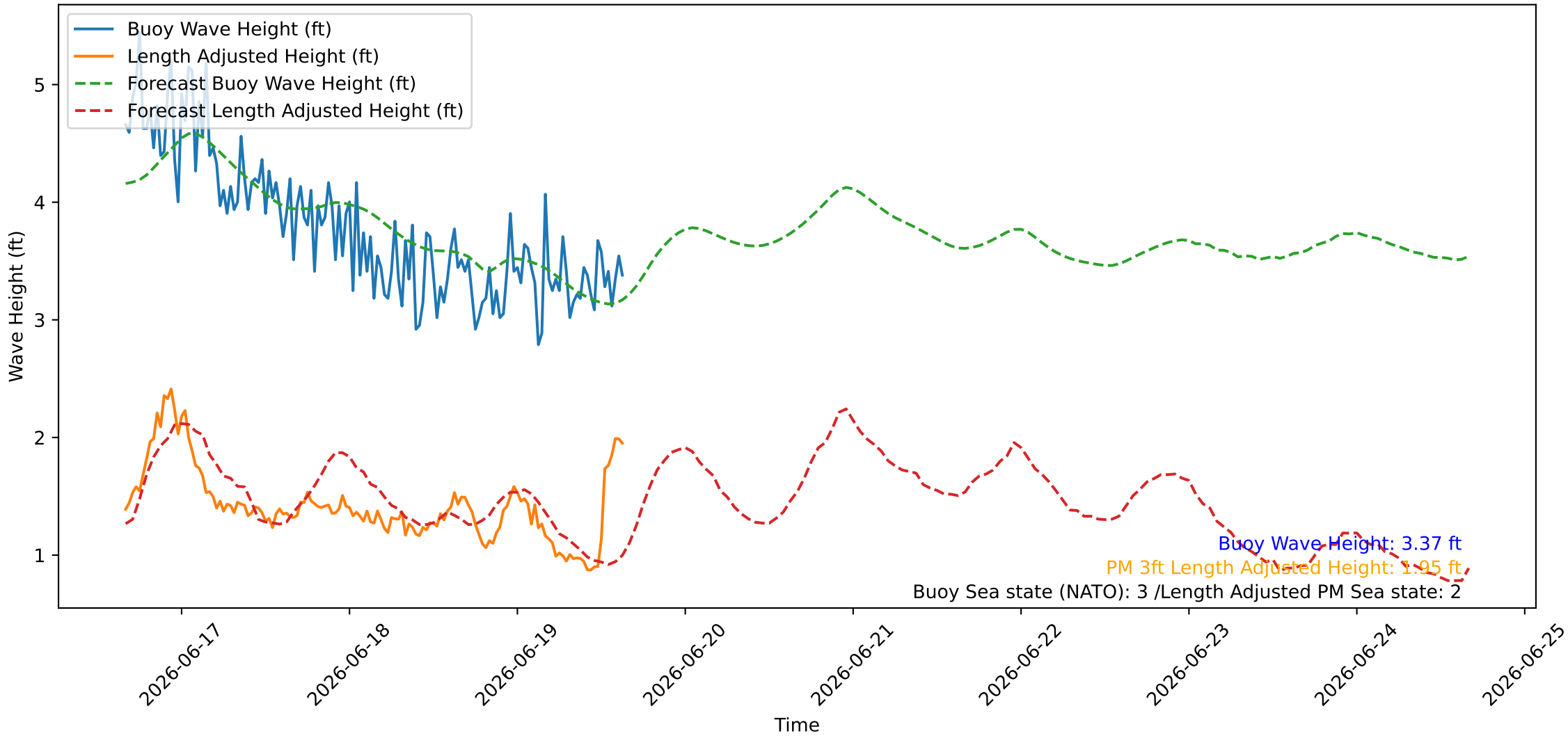
Wave Heights over Time for Oceanside Harbor at 2026-06-19 15:50:25
