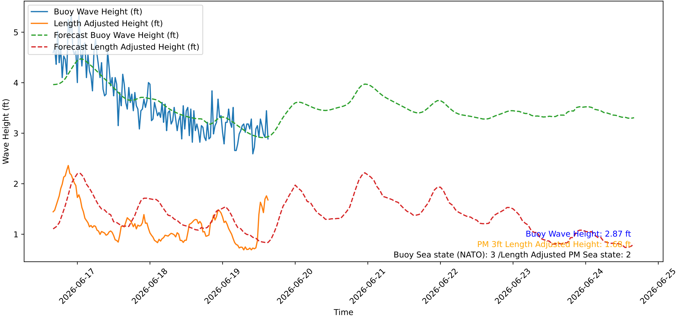
Wave Heights over Time for Red Beach at 2026-06-19 15:50:46
