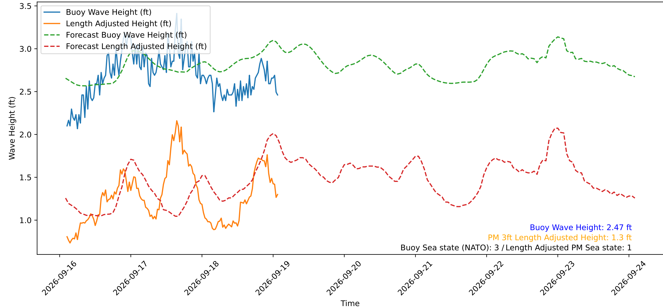
Wave Heights over Time for Red Beach at 2026-09-19 02:10:49
