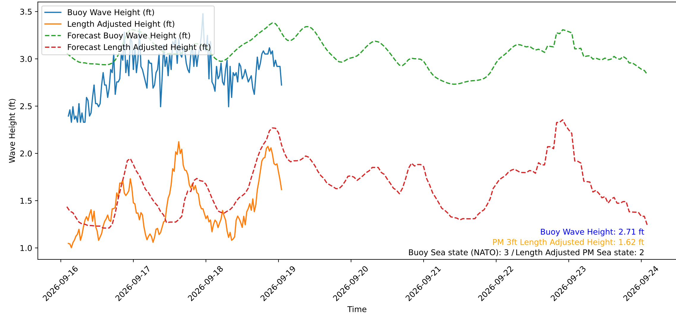
Wave Heights over Time for Green Beach at 2026-09-19 02:11:11
