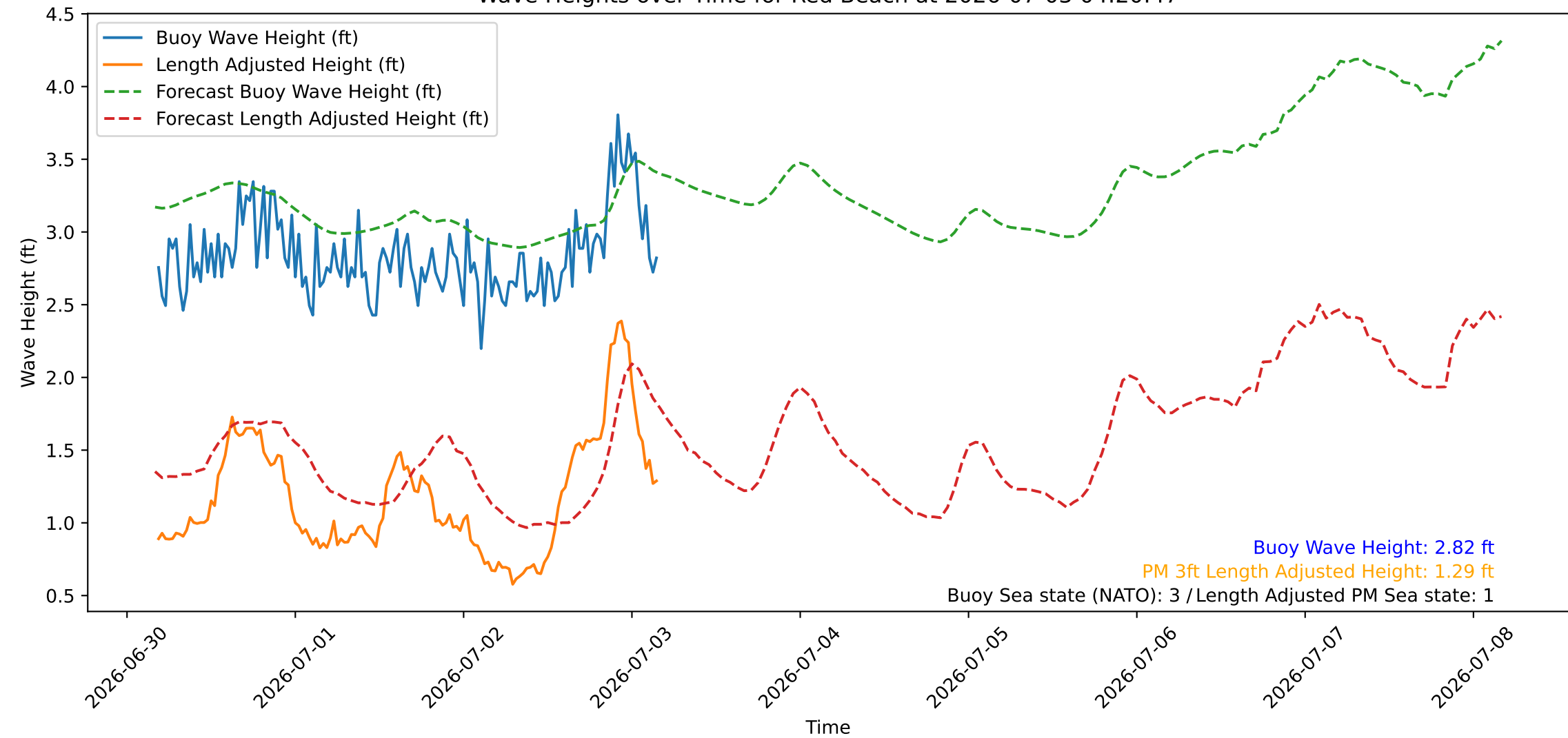
Wave Heights over Time for Red Beach at 2026-07-03 04:20:47
