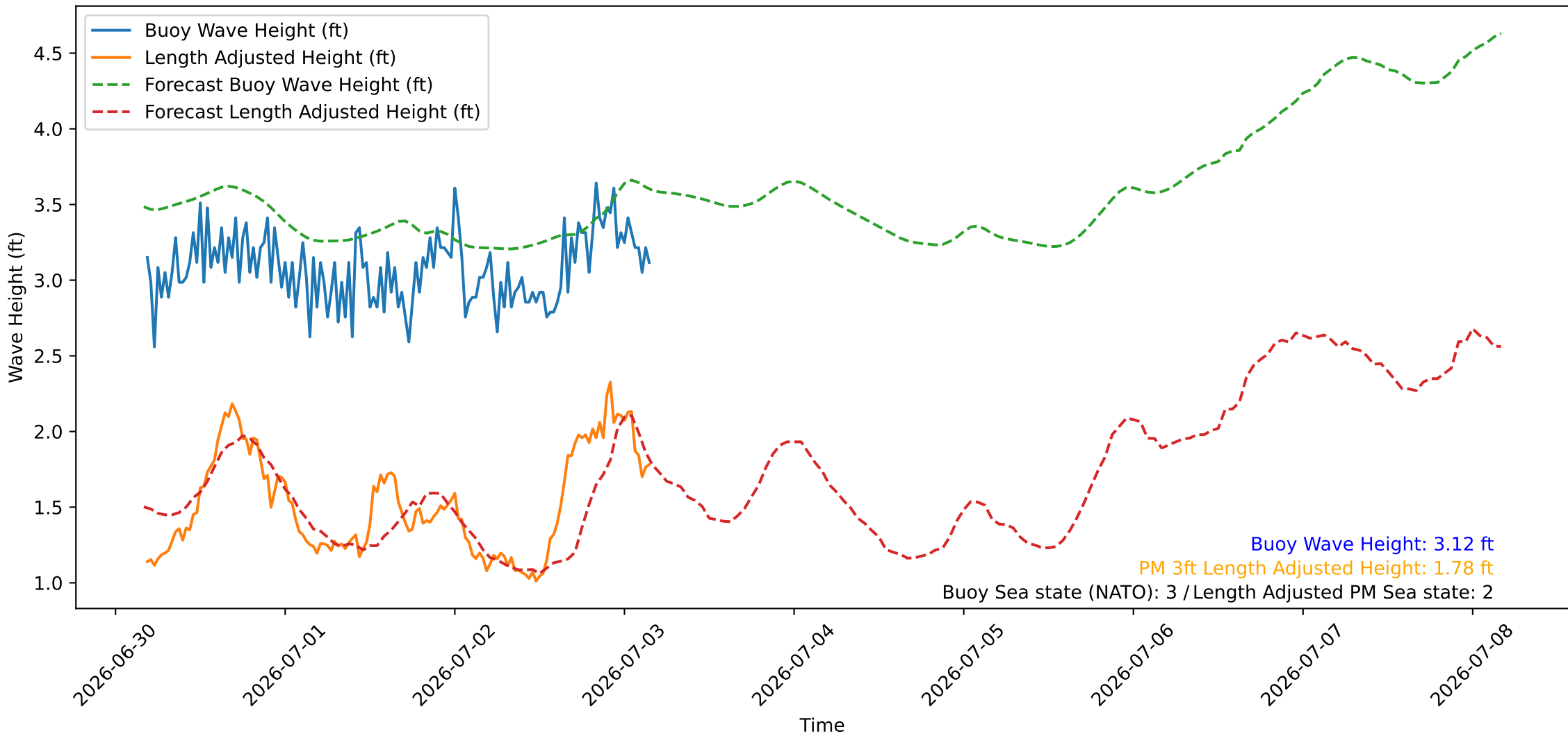
Wave Heights over Time for Oceanside Harbor at 2026-07-03 04:20:27
