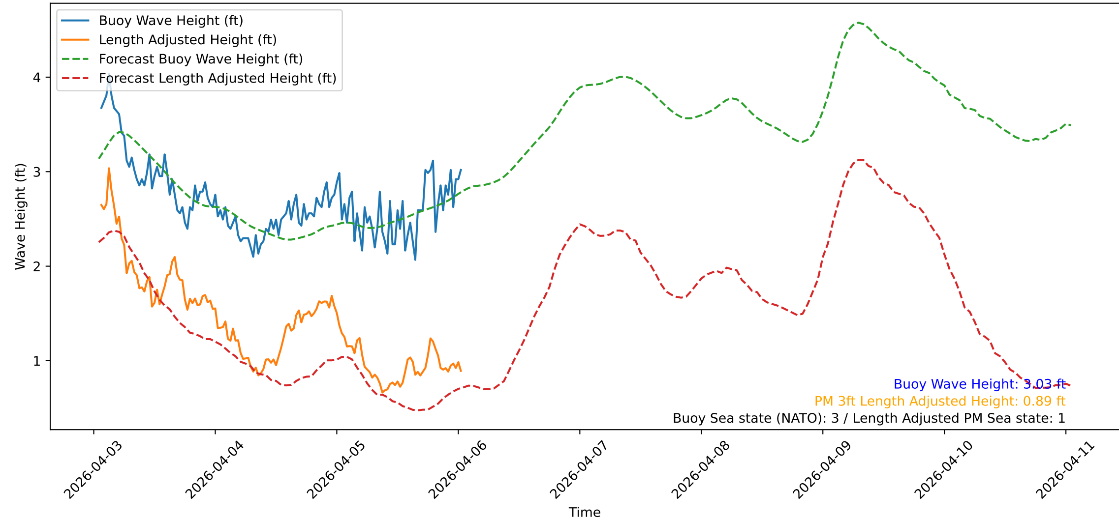
Wave Heights over Time for Oceanside Harbor at 2026-04-06 01:20:31
