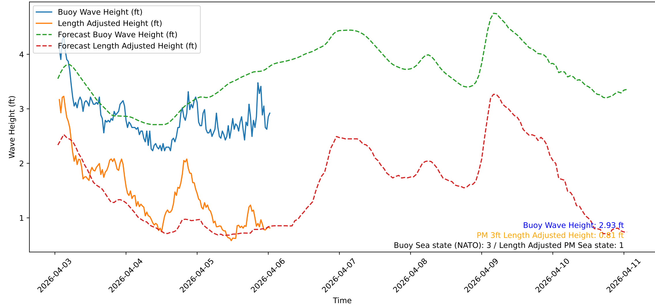
Wave Heights over Time for Green Beach at 2026-04-06 01:21:12
