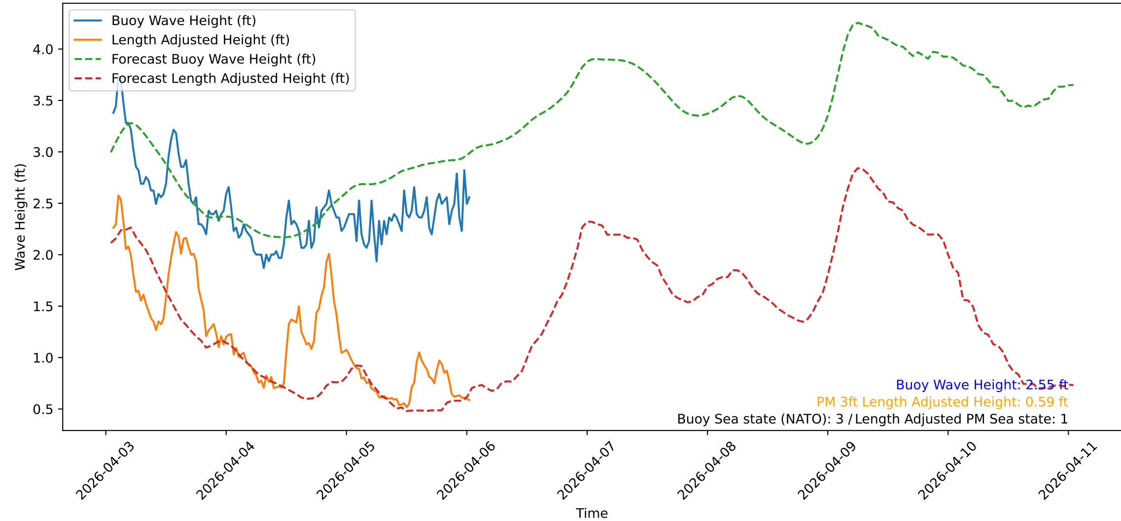
Wave Heights over Time for Red Beach at 2026-04-06 01:20:49
