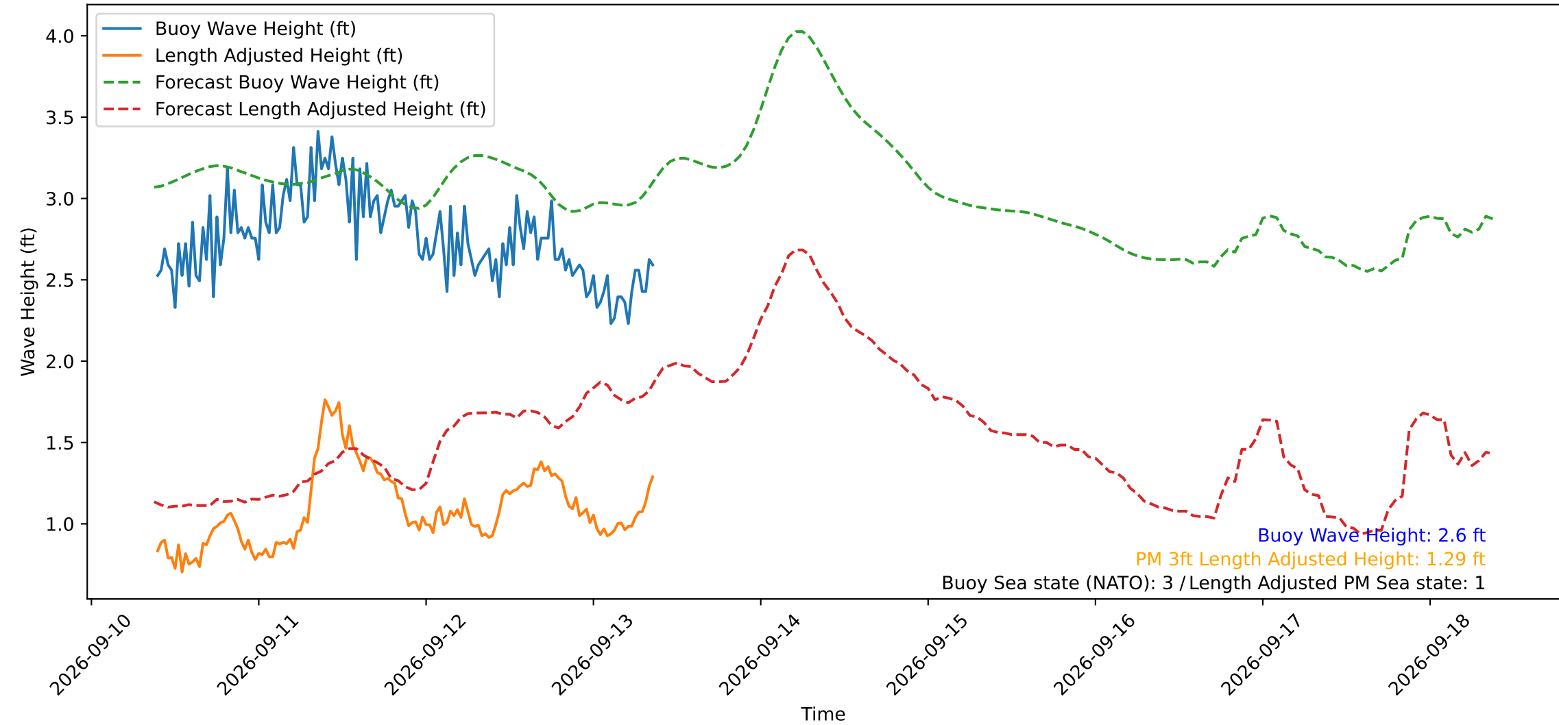
Wave Heights over Time for Red Beach at 2026-09-13 09:10:49
