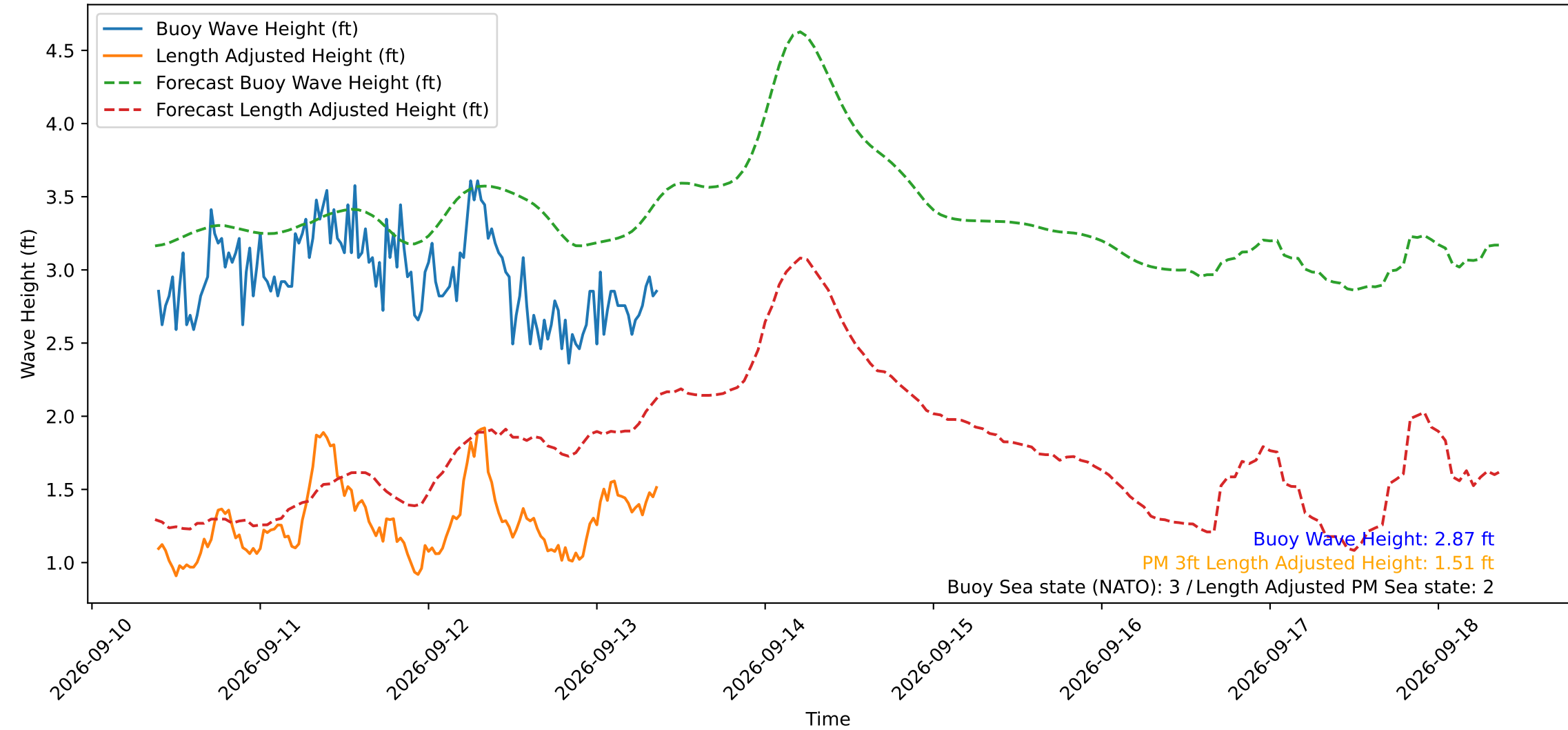
Wave Heights over Time for Green Beach at 2026-09-13 09:11:12
