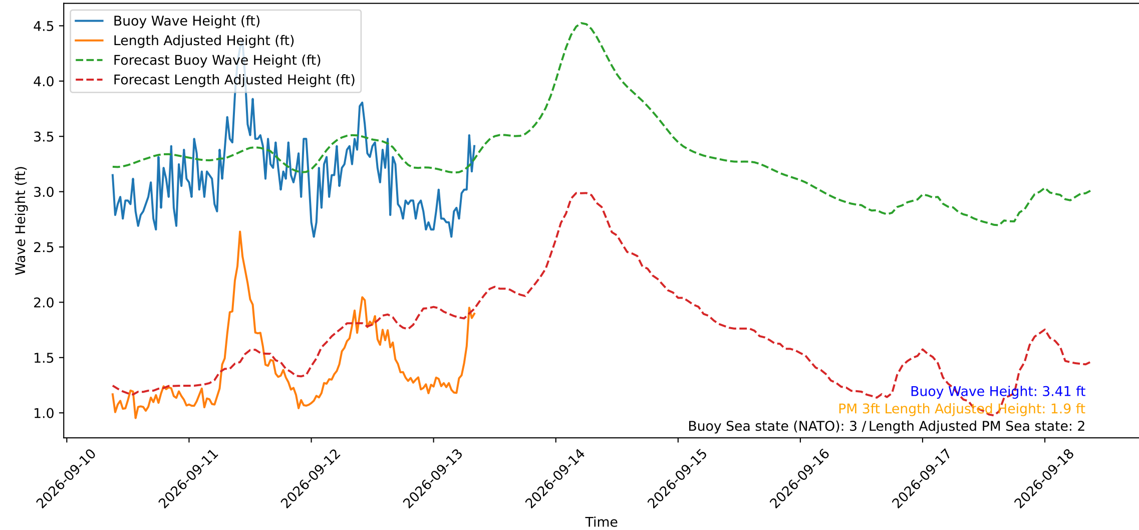
Wave Heights over Time for Oceanside Harbor at 2026-09-13 09:10:30
