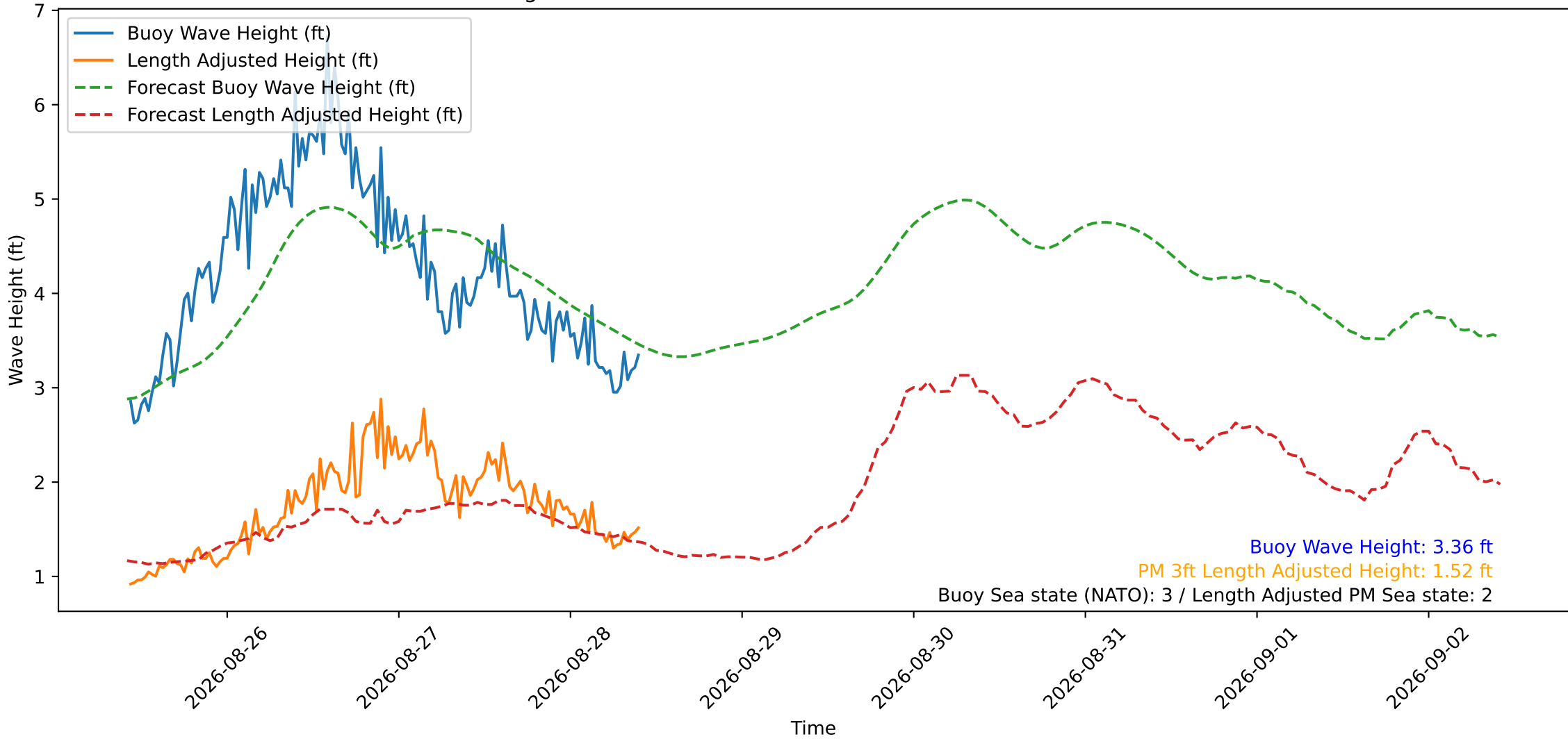
Wave Heights over Time for Oceanside Harbor at 2026-08-28 10:20:30
