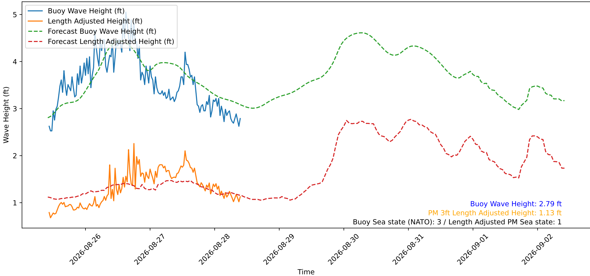
Wave Heights over Time for Red Beach at 2026-08-28 10:20:51
