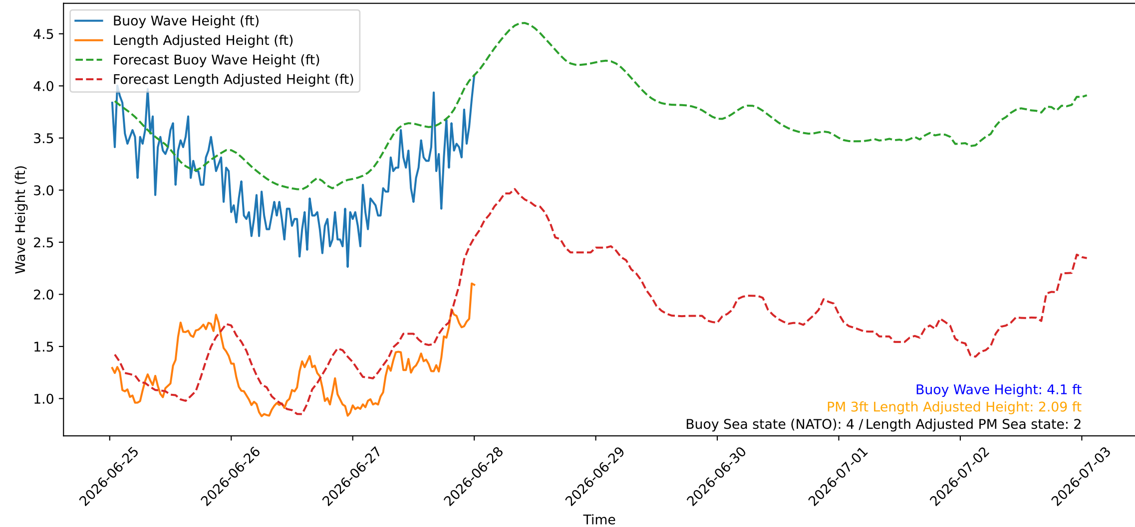
Wave Heights over Time for Green Beach at 2026-06-28 00:41:08
