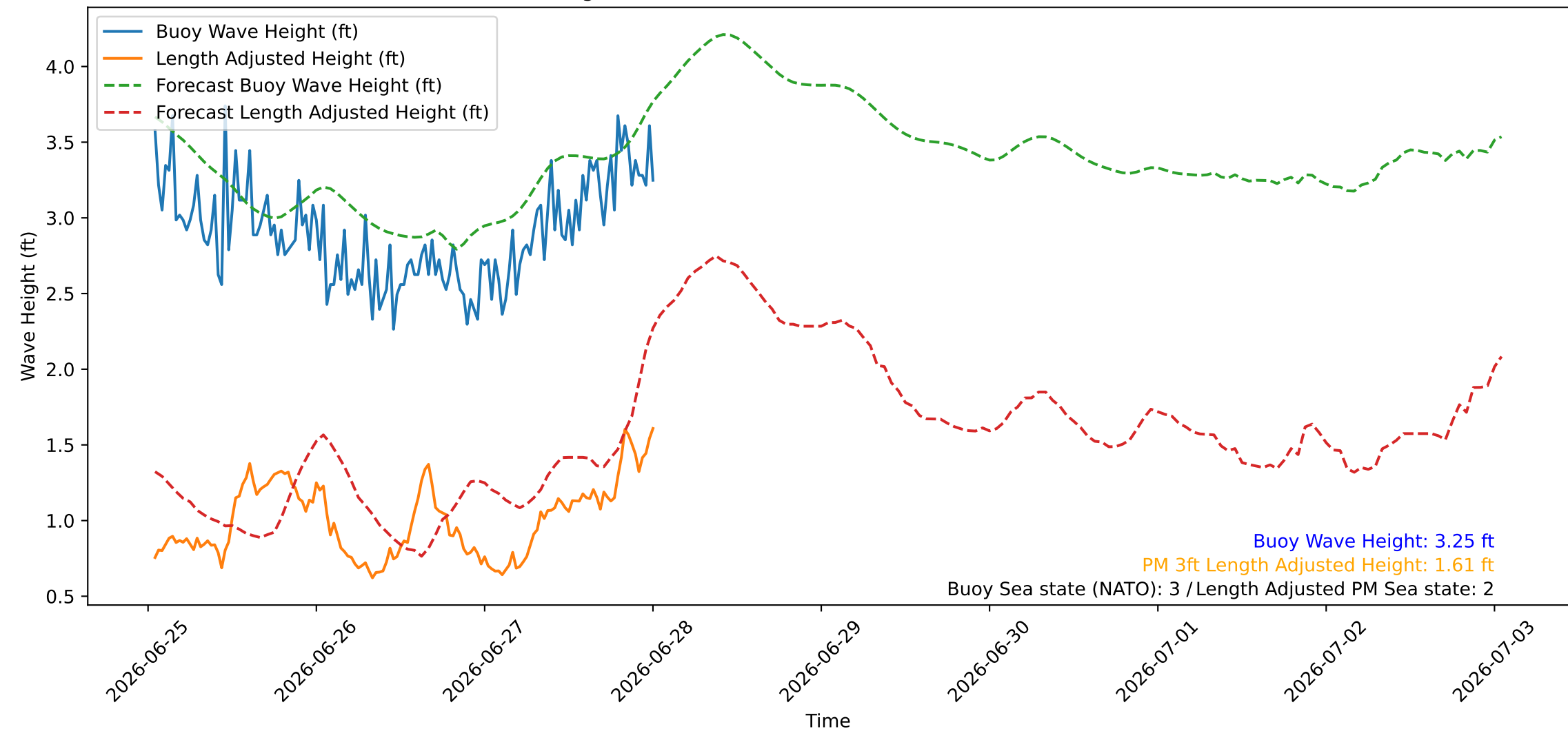
Wave Heights over Time for Red Beach at 2026-06-28 00:40:45
