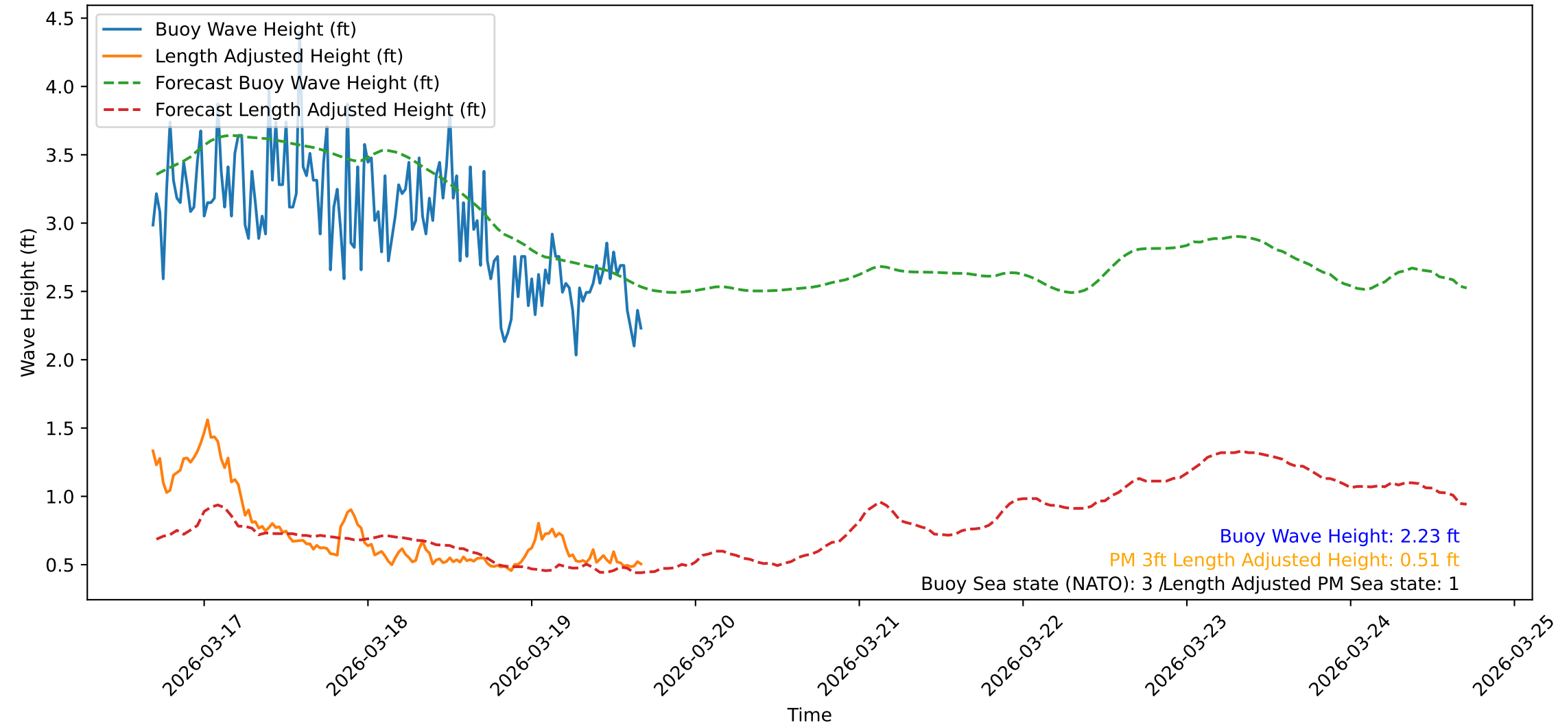
Wave Heights over Time for Oceanside Harbor at 2026-03-19 16:30:31
