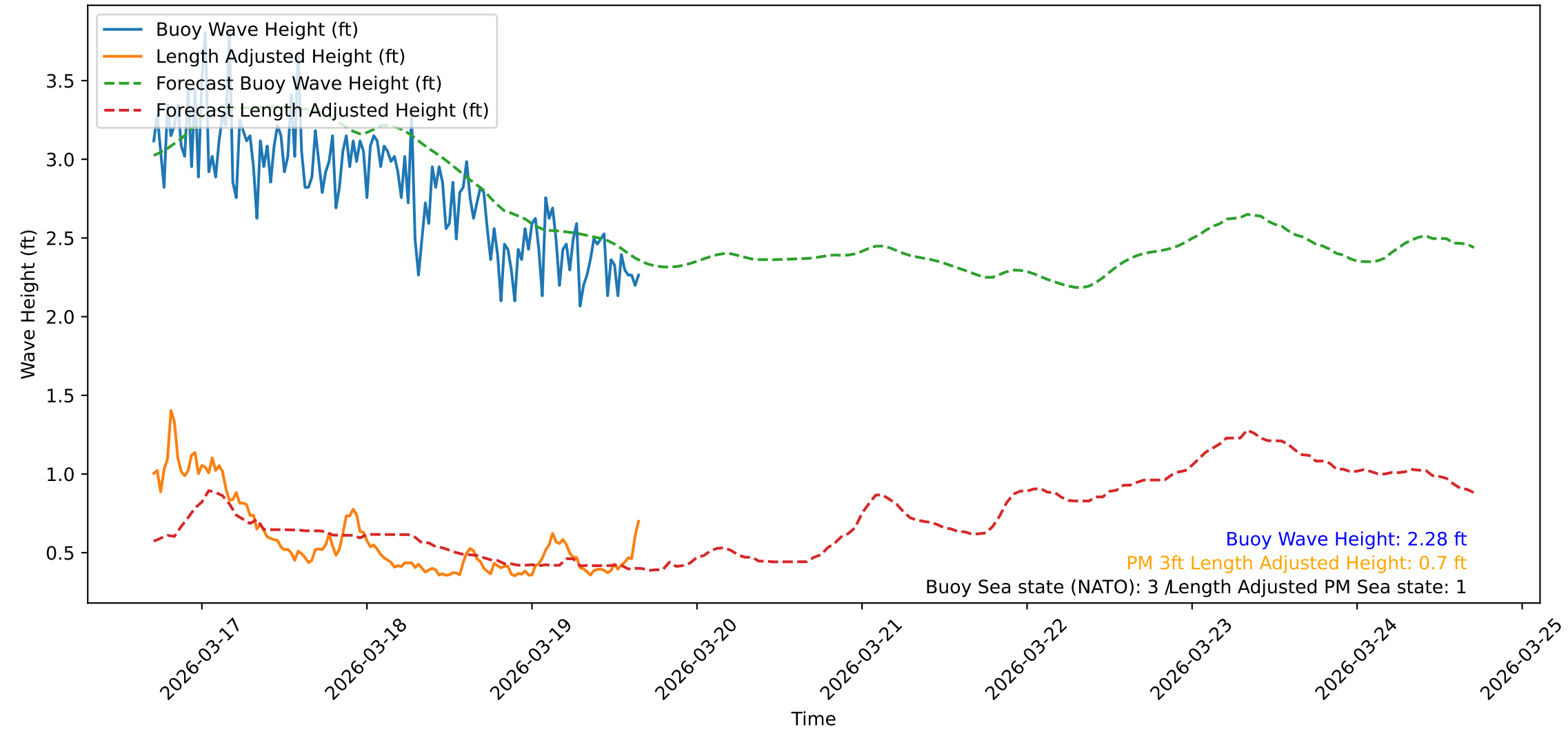
Wave Heights over Time for Red Beach at 2026-03-19 16:30:48
