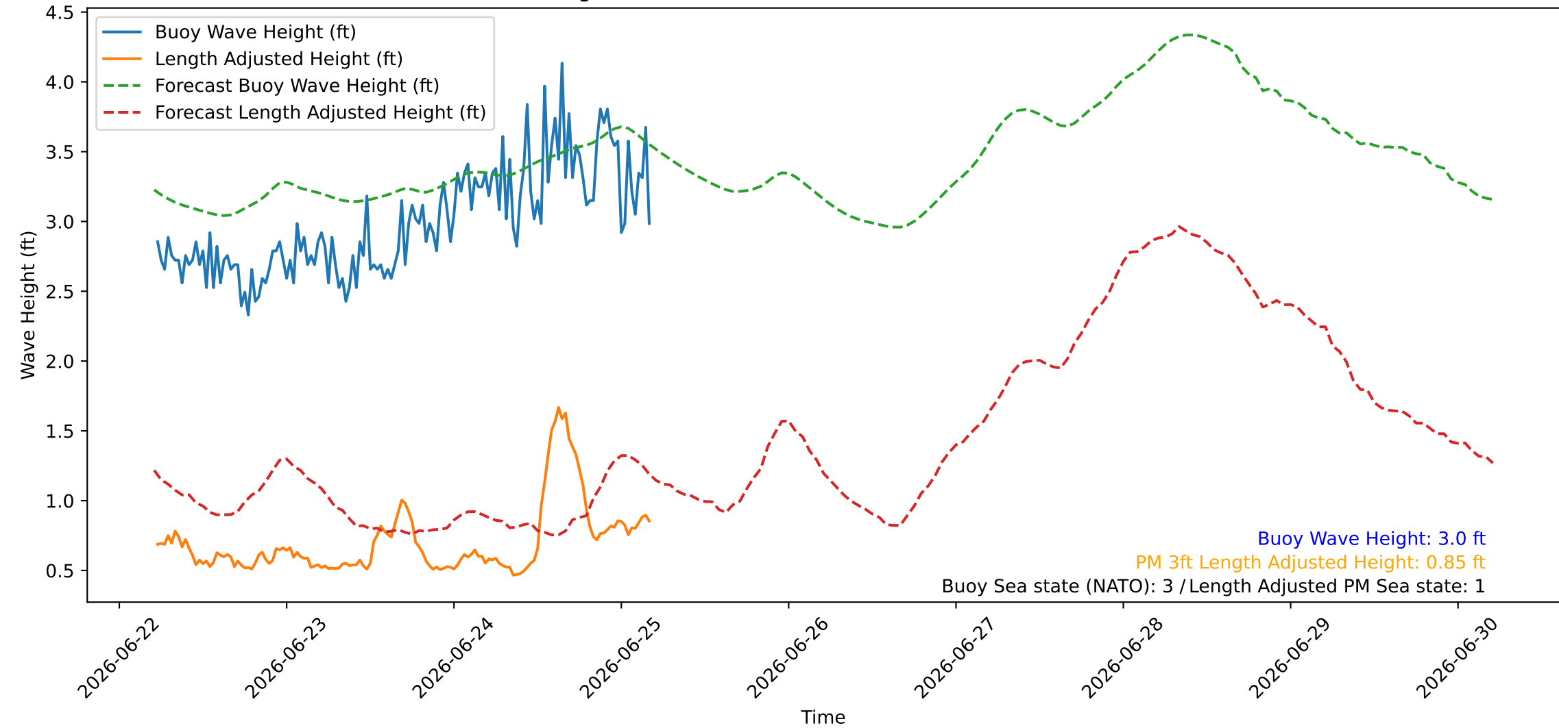
Wave Heights over Time for Red Beach at 2026-06-25 05:00:45
