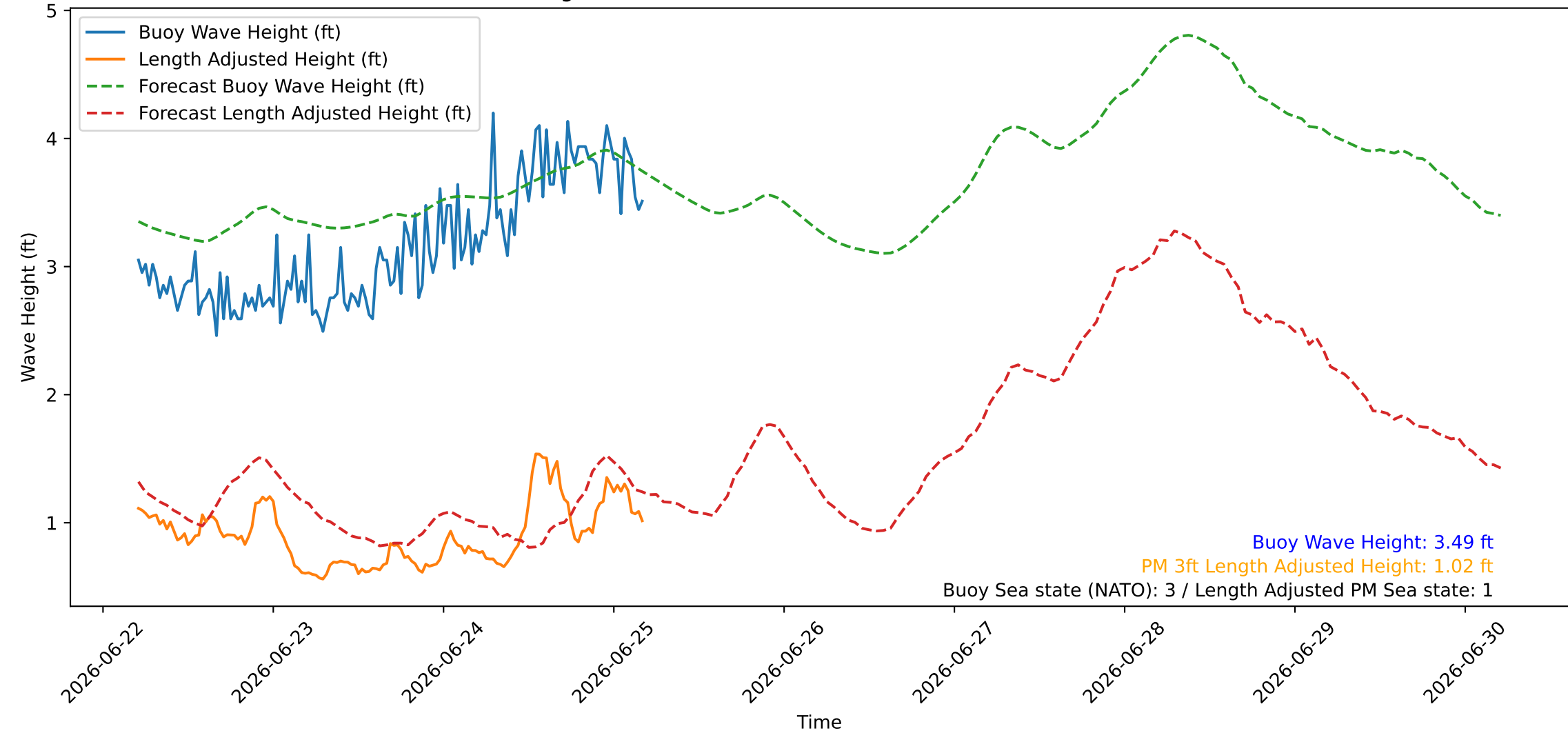
Wave Heights over Time for Green Beach at 2026-06-25 05:01:07
